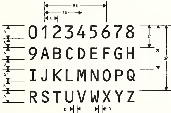
Figure C1. Alphanumeric Characters (refer to Table C1)
