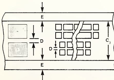
Figure 13c. Duo and Duo Duplex Roll Microfilm Formats (area E located on both edges of the microfilm)
