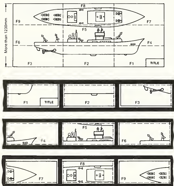
Document as it appears on roll film.*
