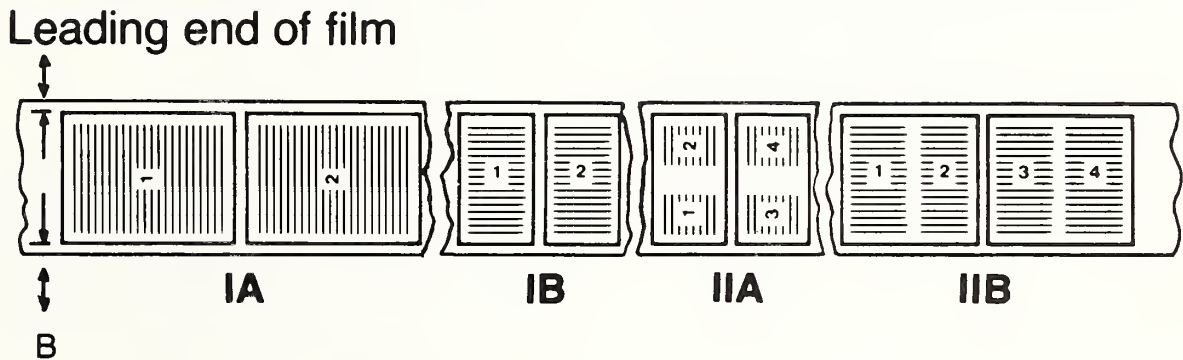
Figure 5. Simplex Format (See Tables 1 and 2 for dimensions)
