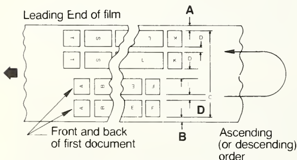
Figure 7. Duplex Format (See Tables 1 and 2 for dimensions)
