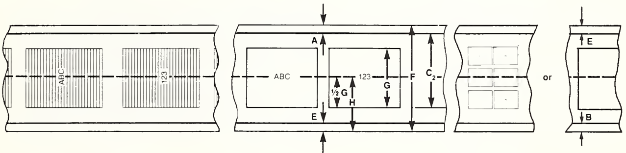
Figure 13b. Simplex, Duplex, and Multiplex Roll Microfilm Formats (area E may be located on either edge of the microfilm)
