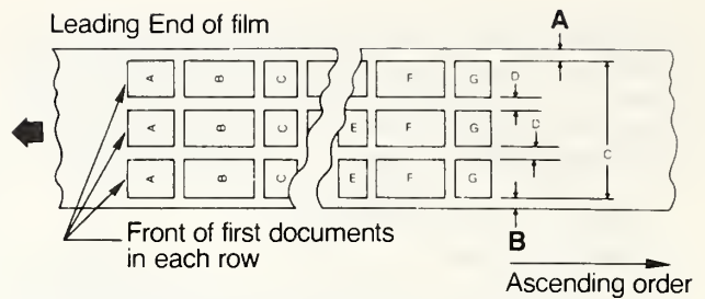
Figure 9. Multiplex Format—Two or More Rows (See Tables 1 and 2 for dimensions)
