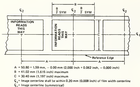
Figure 14. Microimage Placement for 35 mm COM
