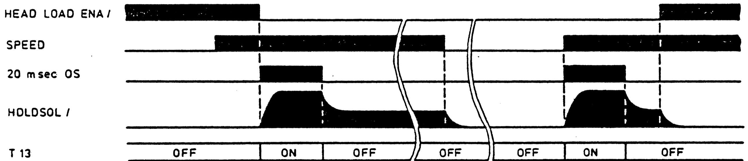
FIGURE 2 - 20 HEAD LOAD - TIMING DIAGRAM
