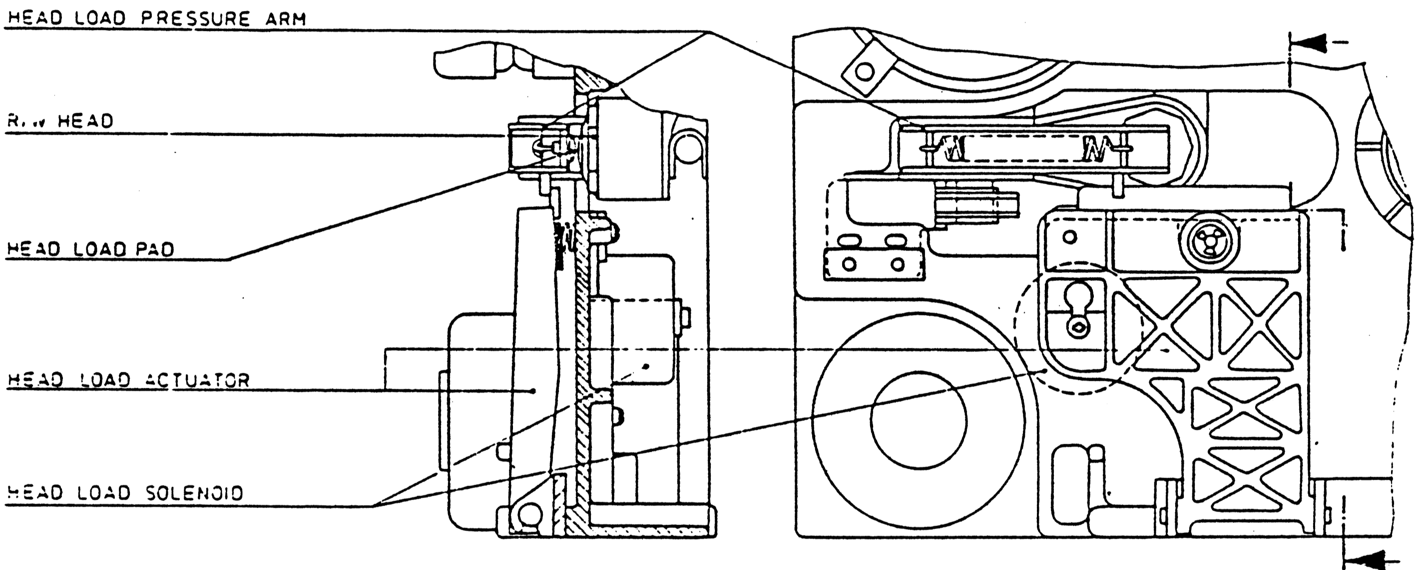
FIGURE 2 - 5a) HEAD LOAD MECHANISM BASF 6106
