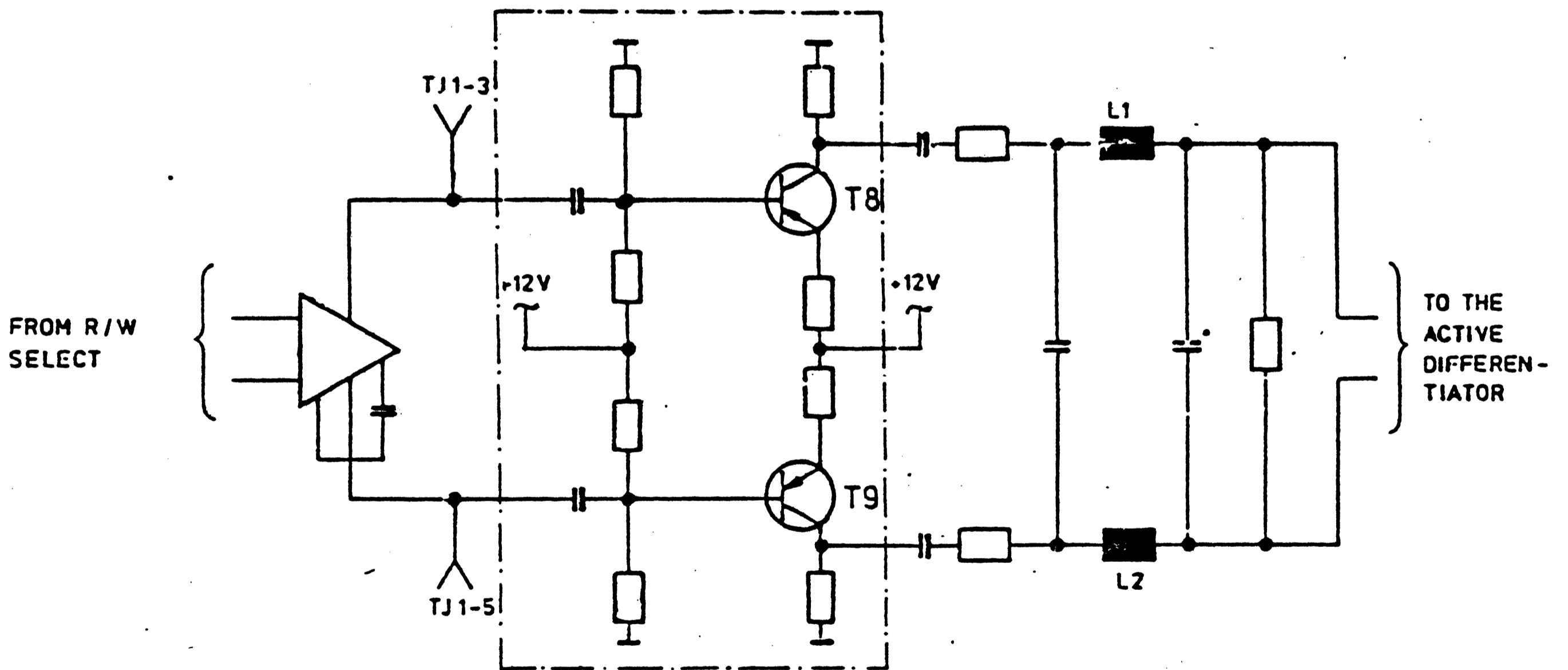
FIG. 2 - 37 READ AMPLIFIERS AND FILTER NETWORK
