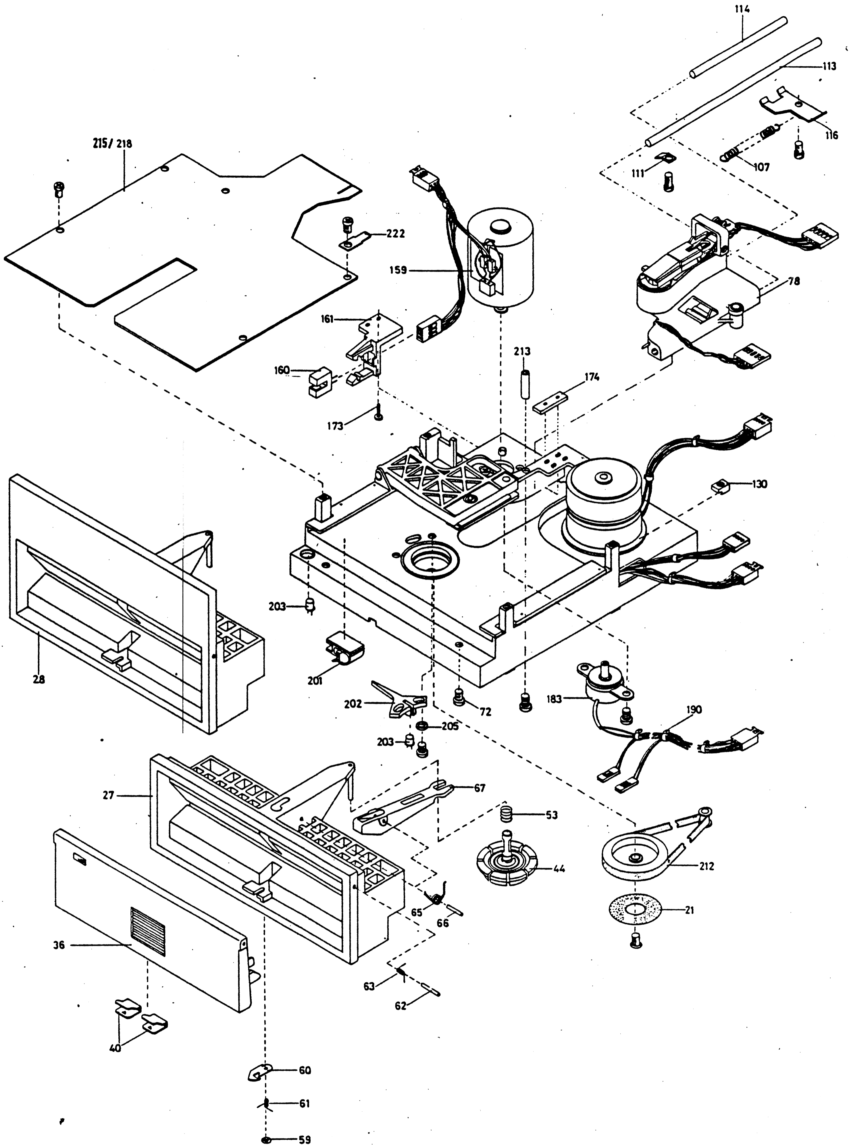
PARTS BREAKDOWN MOD. 6108
