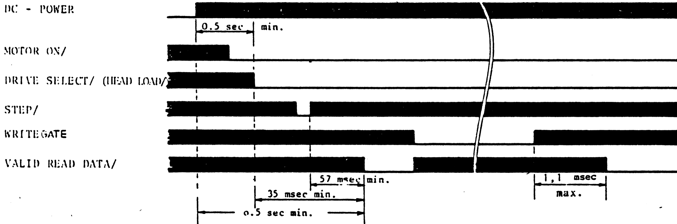
FIGURE 2 - 35 READ INITIATE TIMING
