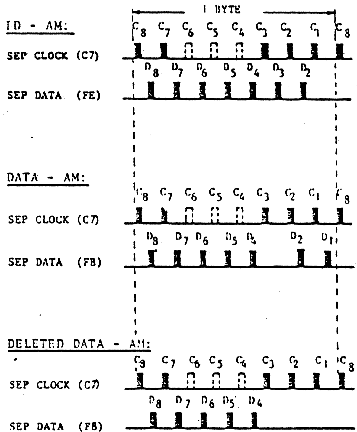
FIG. 1 - 5 ADDRESS MARK PATTERNS
