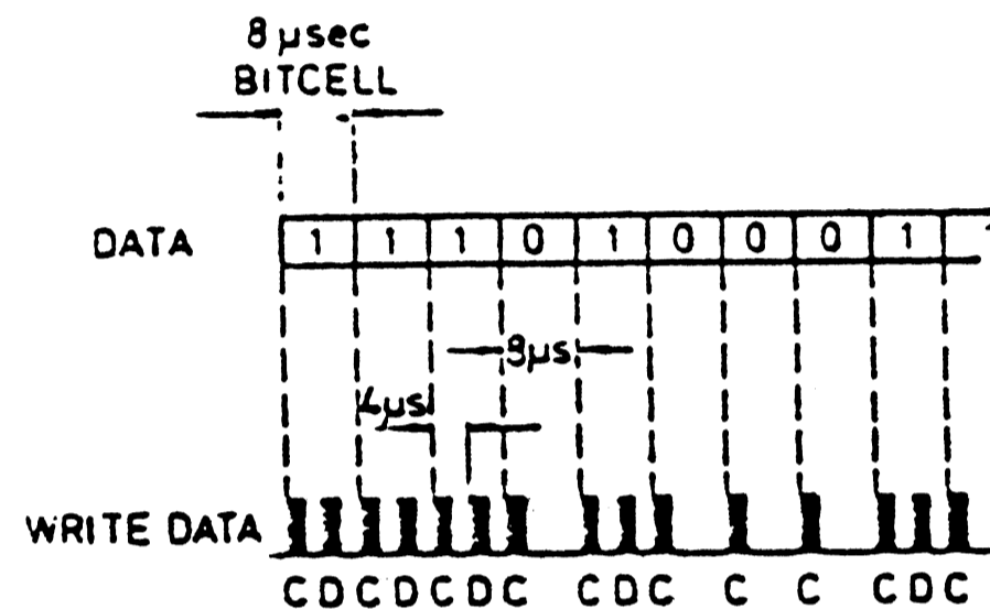
FIG. 1 - 3 FM-ENCODING
