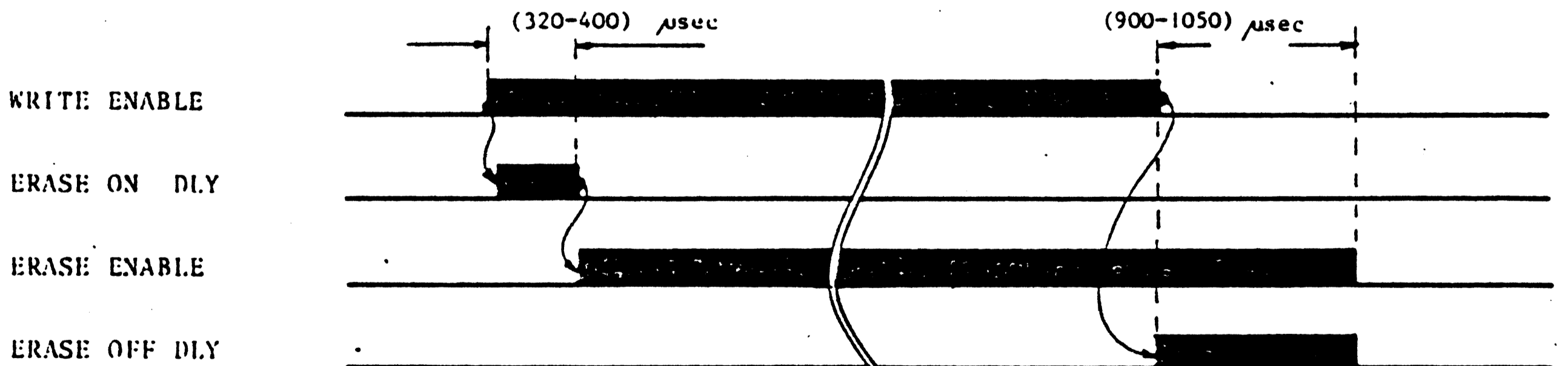
FIGURE 2 - 33 ERASE DELAY TIMING
