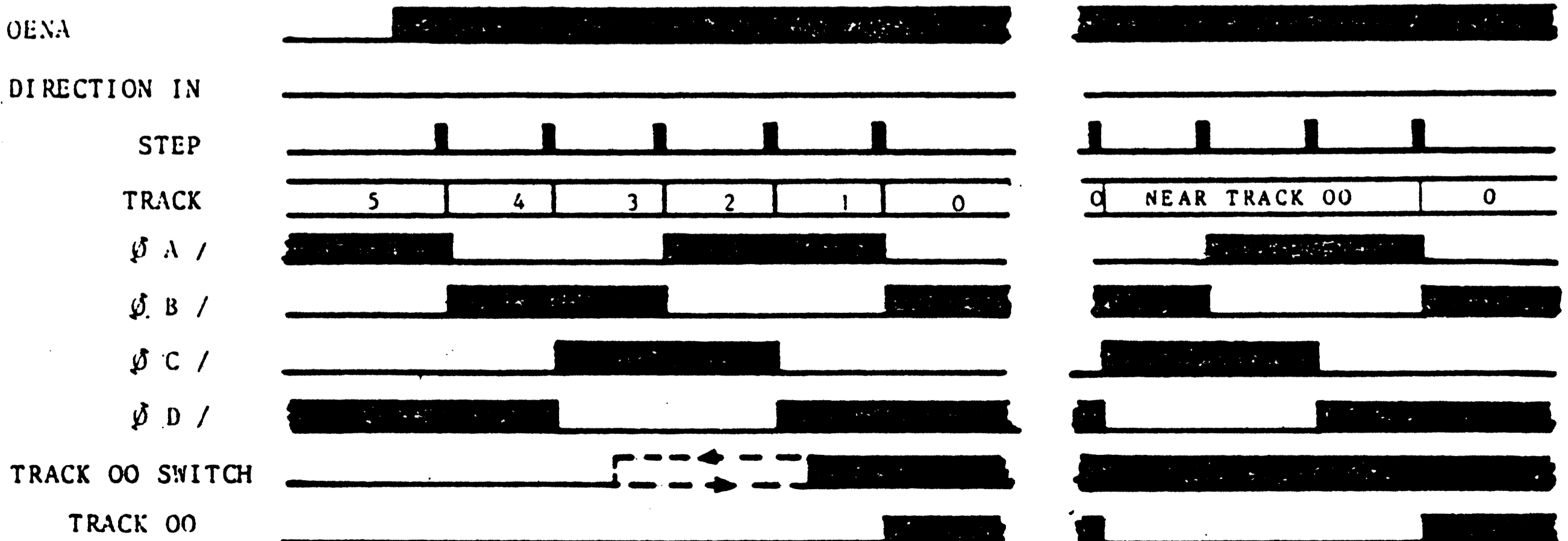
FIGURE 2 - 22 TRACK ZERO - TIMING DIAGRAM
