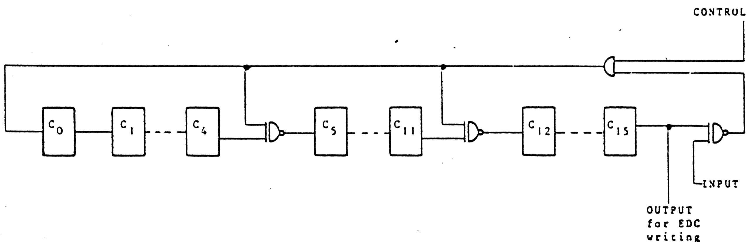
FIGURE 1 - 7 SIMPLIFIED EDC SHIFT REGISTER
