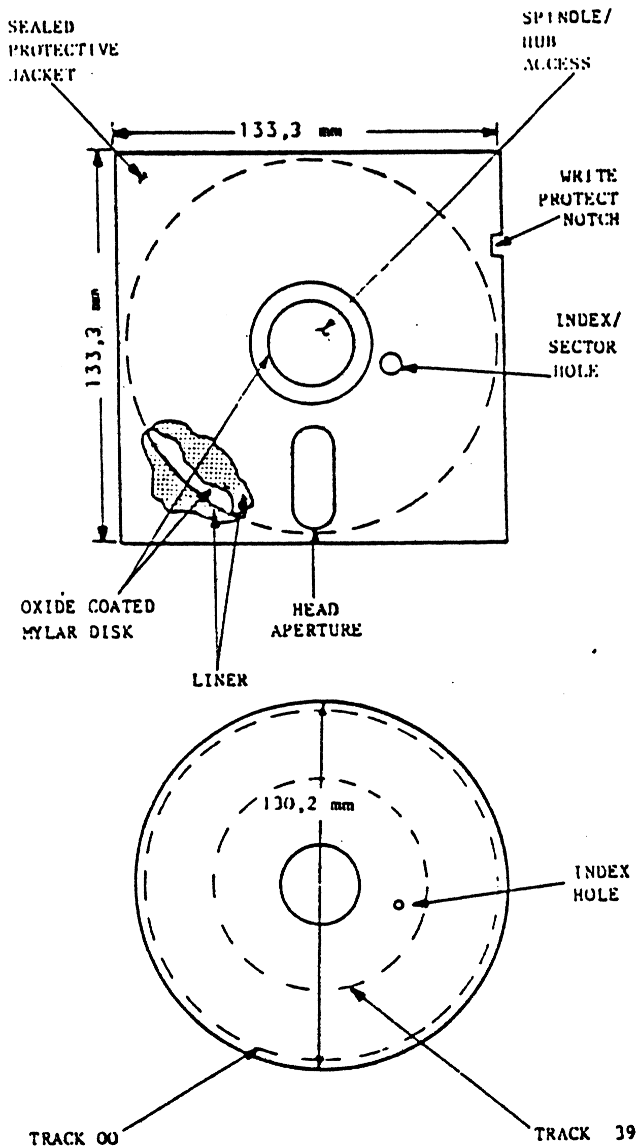
FIG. 1 - 2 FLEXIBLE DISK CONSTRUCTION AND DIMENSIONS
