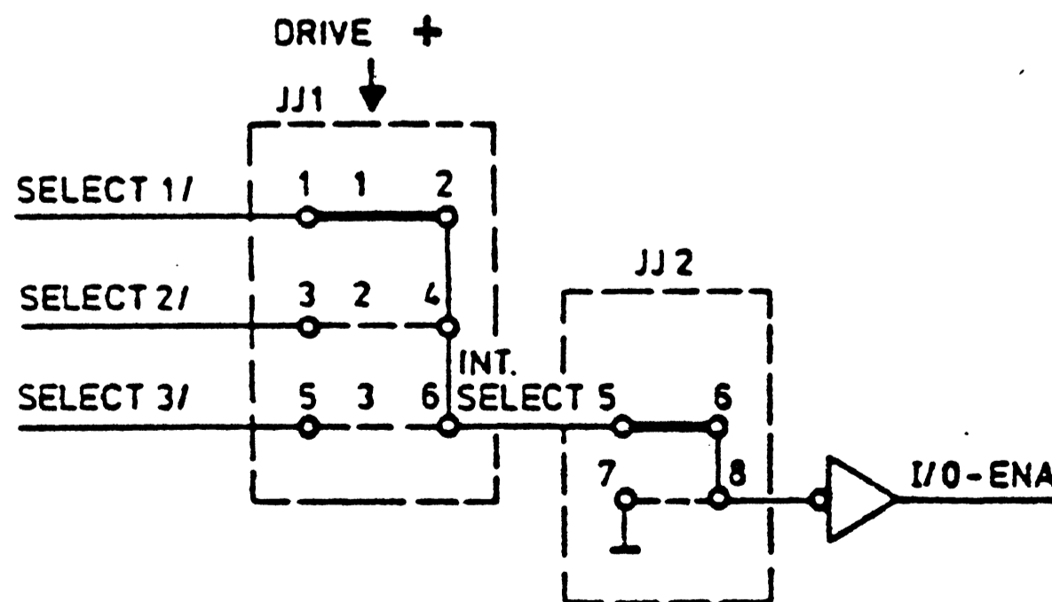
FIGURE 2-8 RADIAL SELECT OPTION
