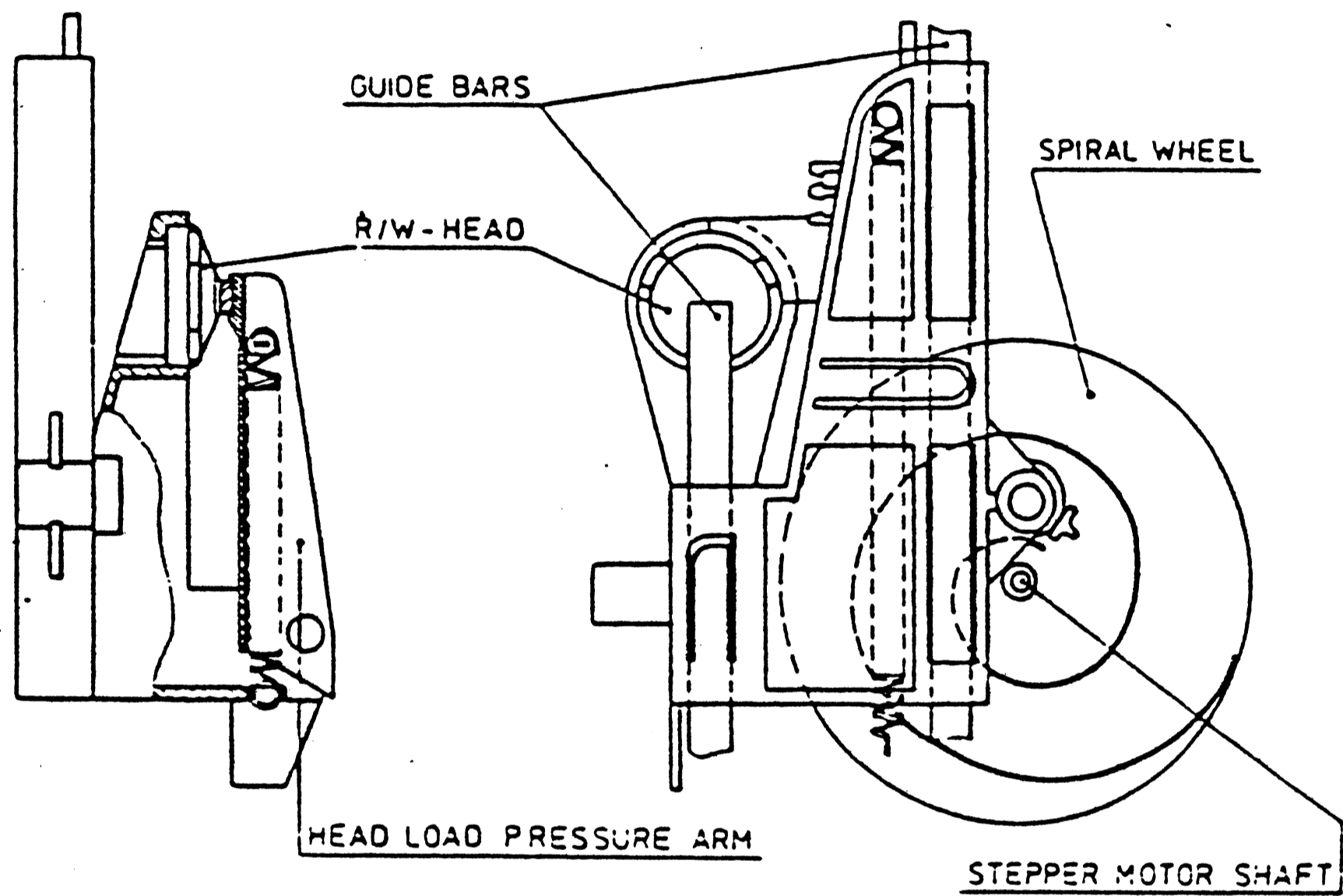
FIGURE 2 - 4 a) POSITIONING MECHANISM BASF 6106
