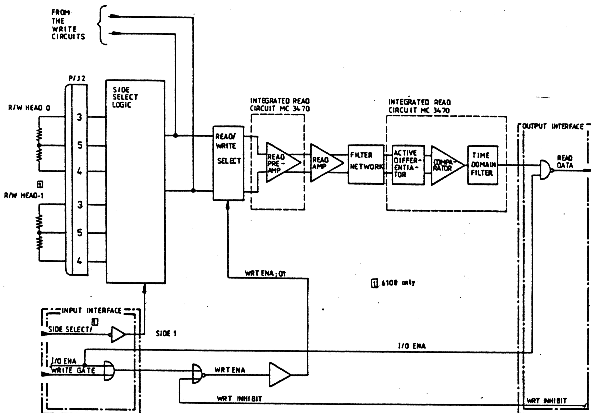
FIGURE 2 - 34 READ CIRCUITS BASF 6106/6108 (SIMPLIFIED)
