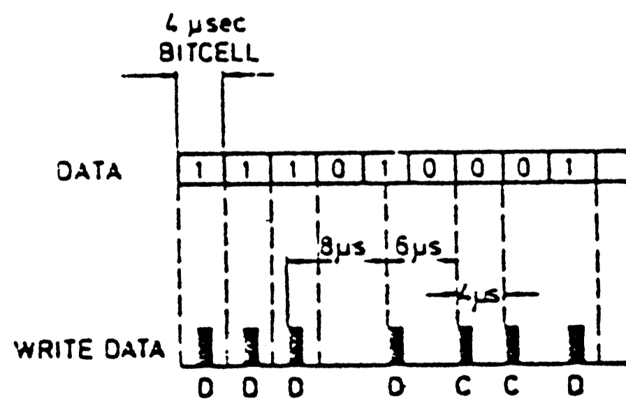
FIG. 1 - 4 MFM-ENCODING
