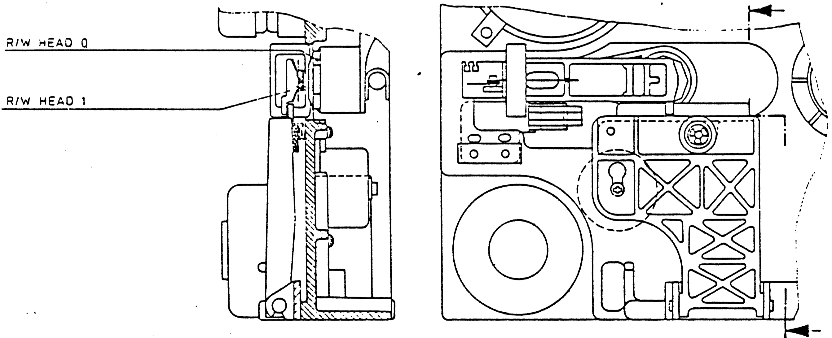
FIGURE 2 - 5b) HEAD LOAD MECHANISM BASF 6108
