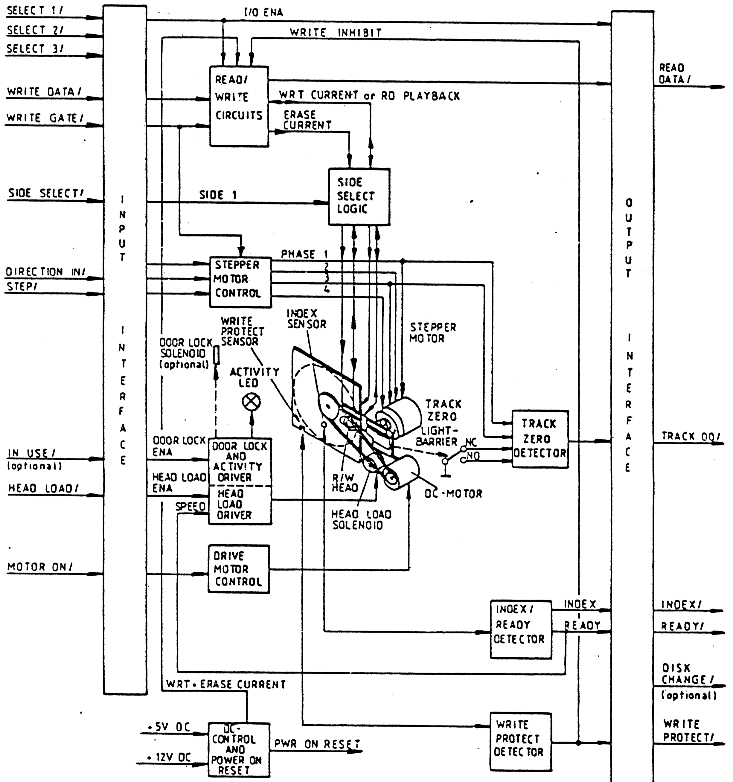
FIGURE 2 - 1 BLOCK DIAGRAM BASF 6106/6108
