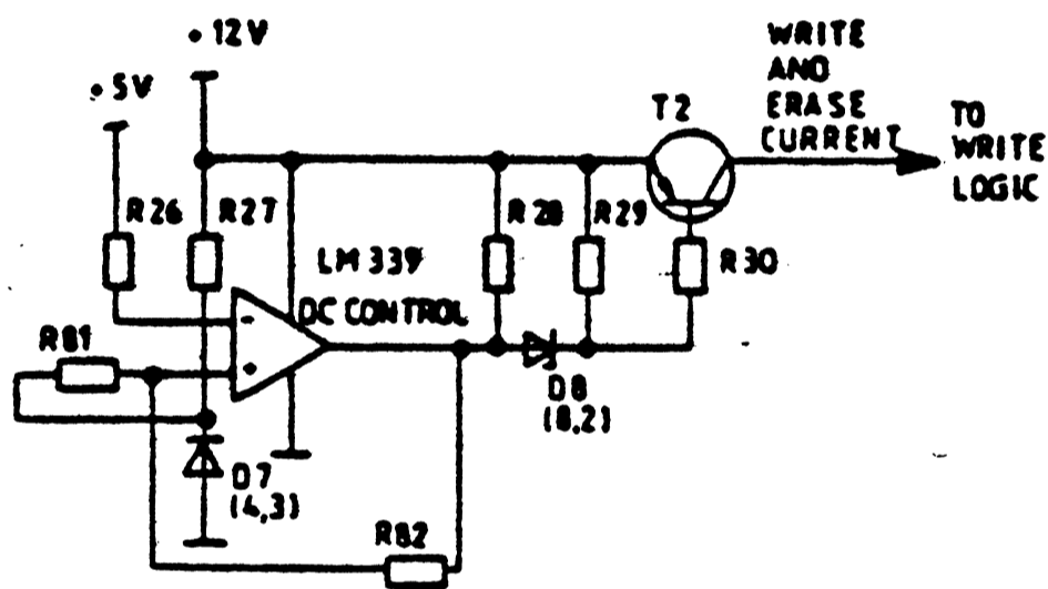
FIG. 2 - 41 DC-CONTROL LOGIC
