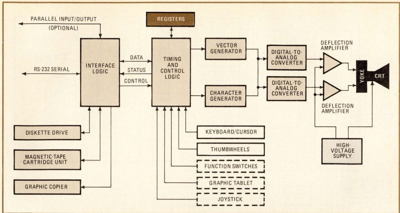
2. Storage display. In the direct-view storage CRT display, a pair of registers replaces refresh memory, while the phosphor screen is erased by flooding with secondary electrons, a relatively slow process. However, storage and random-access CRTs can handle graphics rapidly.
