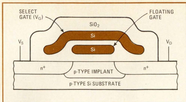
3. Stacked. By applying an n-channel two-layer process to its floating-gate avalanche MOS structures, Intel Corp. built 450-ns access time and high reliability into its 2708 UV-erasable PROM. The top gate selects, the bottom floating gate stores.
