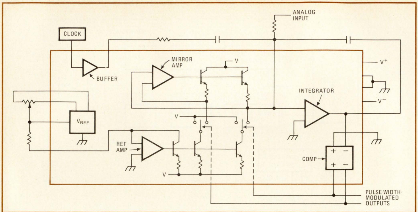
6. High resolution. With standard bipolar processing, Nippon Electric has managed to put a 4\frac{1}{2} -digit integrating a-d converter on one chip. The device delivers a pulse-width-modulated output and holds linearity error to less than 0.002%, temperature drift to 10 ppm/°C.
