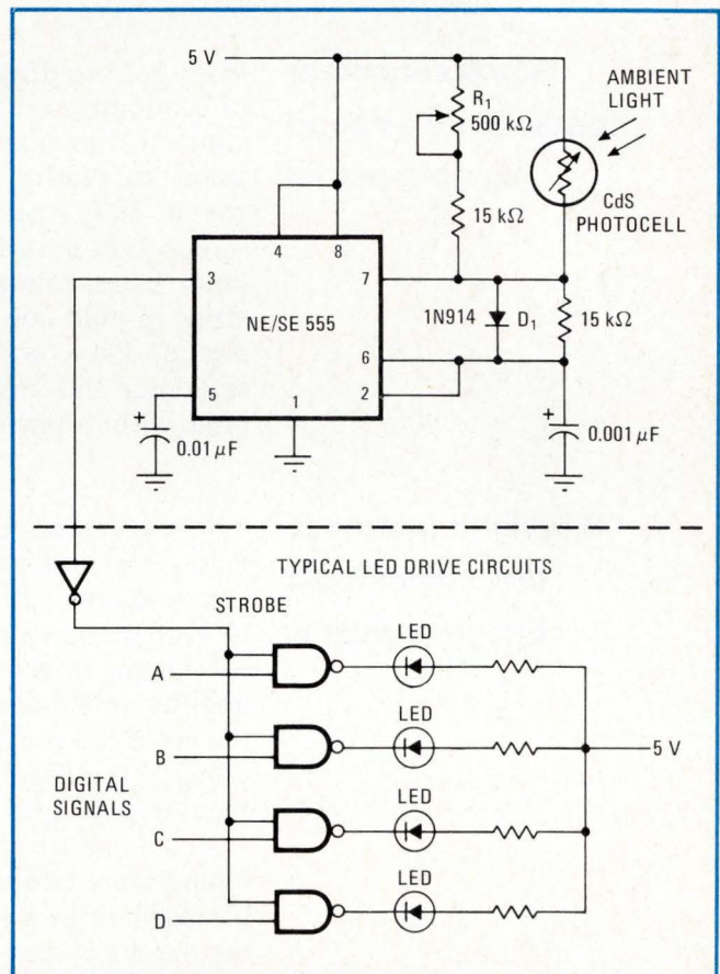
Fader. Brightness of LED display is varied by using a photocell in place of one timing resistor in a 555 timer, and bypassing the other timing resistor to boost the timer's maximum duty cycle. Result is brighter display in sunlight, fainter in the dark.
