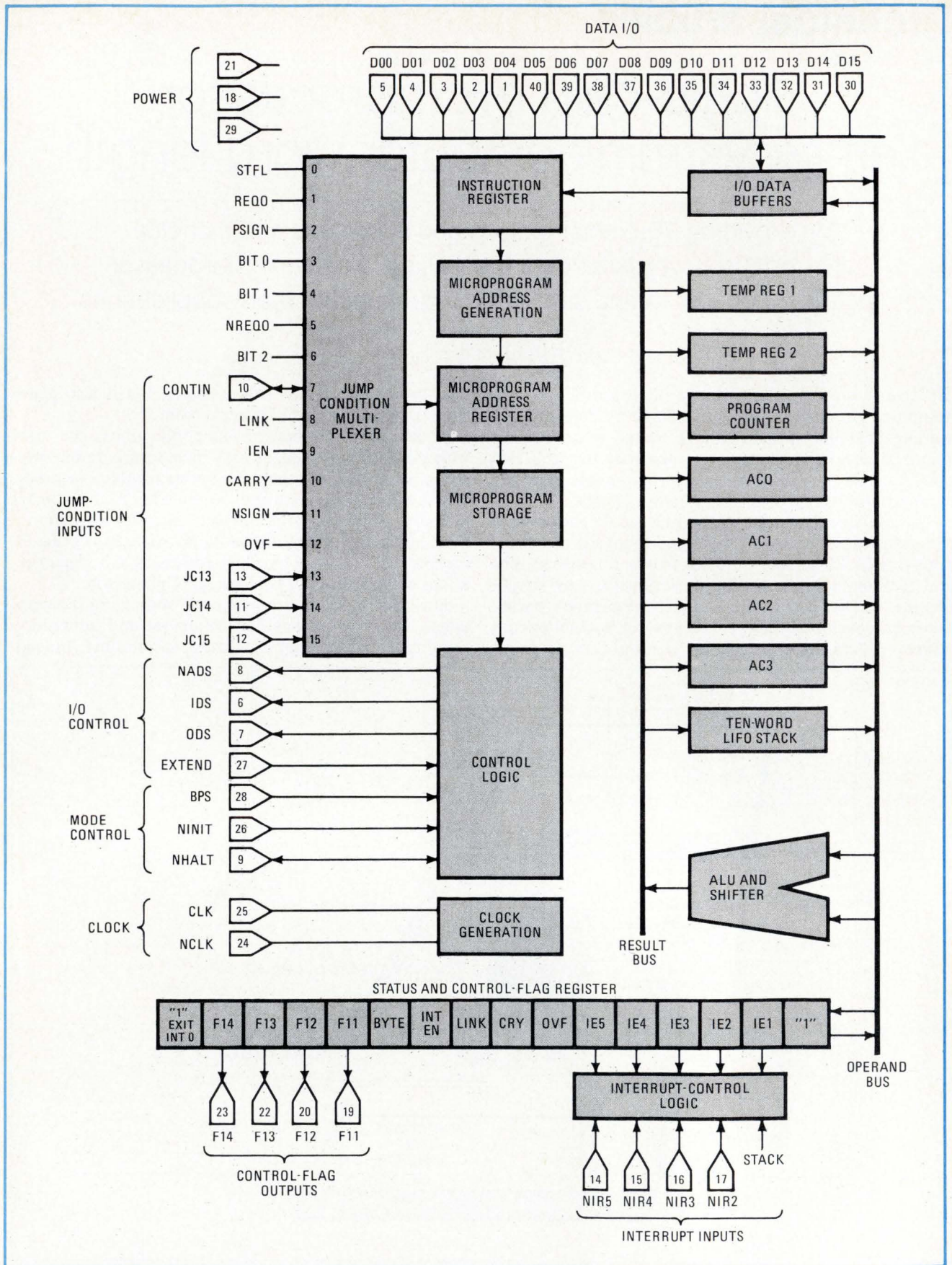
2. On the Inside. Seven 16-bit registers are included in PACE, along with a last-in, first-out stack for additional storage of up to 10 words. The status-flag register can be loaded from any accumulator. The byte flag is used to specify 8-bit or 16-bit data lengths.
