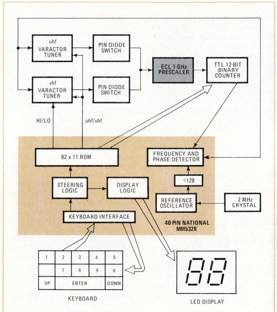
Turn-on. TV-channel synthesizer/controller section of digital tuning circuit developed jointly by National Semiconductor and Plessey Semiconductor eventually should be integrated in single 40-pin National package. Plessey is building the 1-GHz prescaler.
