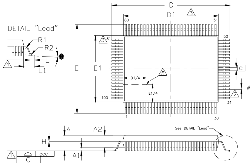
Figure 2 - 100 Pin QFP Package
