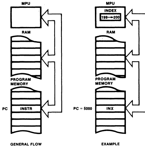
Fig. 20 Inherent Addressing
