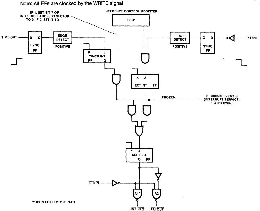
Figure 14 Conceptual Illustration of F3851 PSU Interrupt Logic
