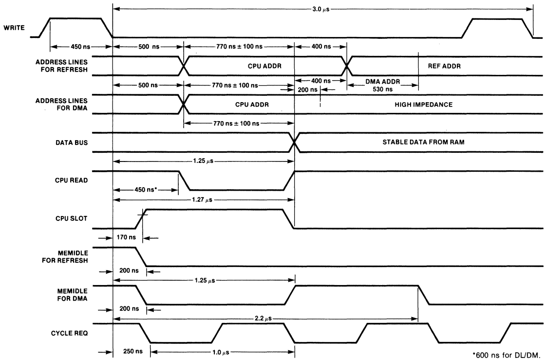
Fig. 4 Memory Refresh and DMA Timing During Long-Cycle Memory Read, with Address Out of Program Counter
