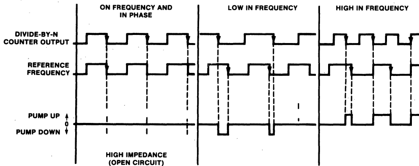
Fig. 14 Output Waveforms from Frequency/Phase Comparator
