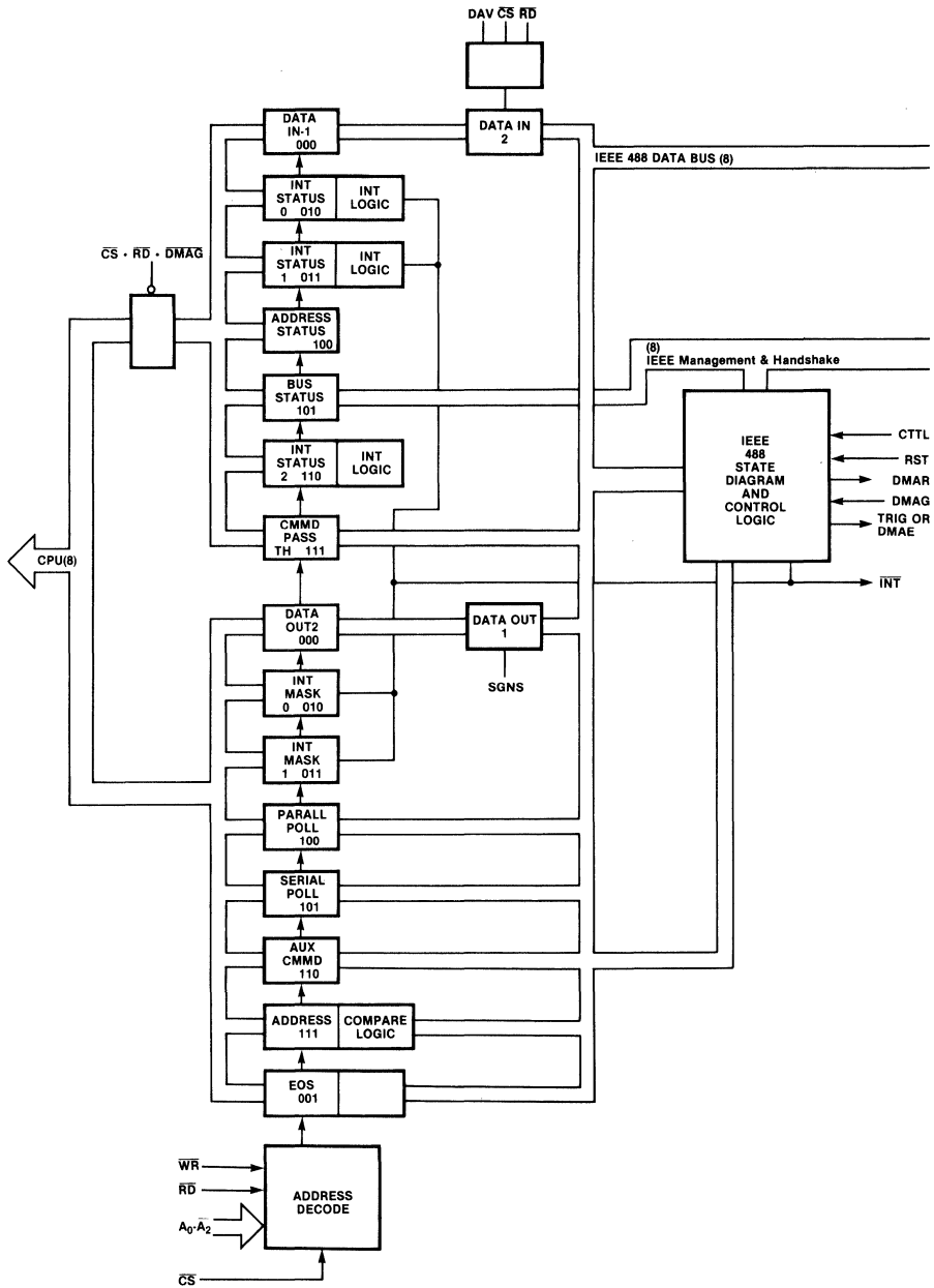
Figure 1 F16488 Block Diagram
