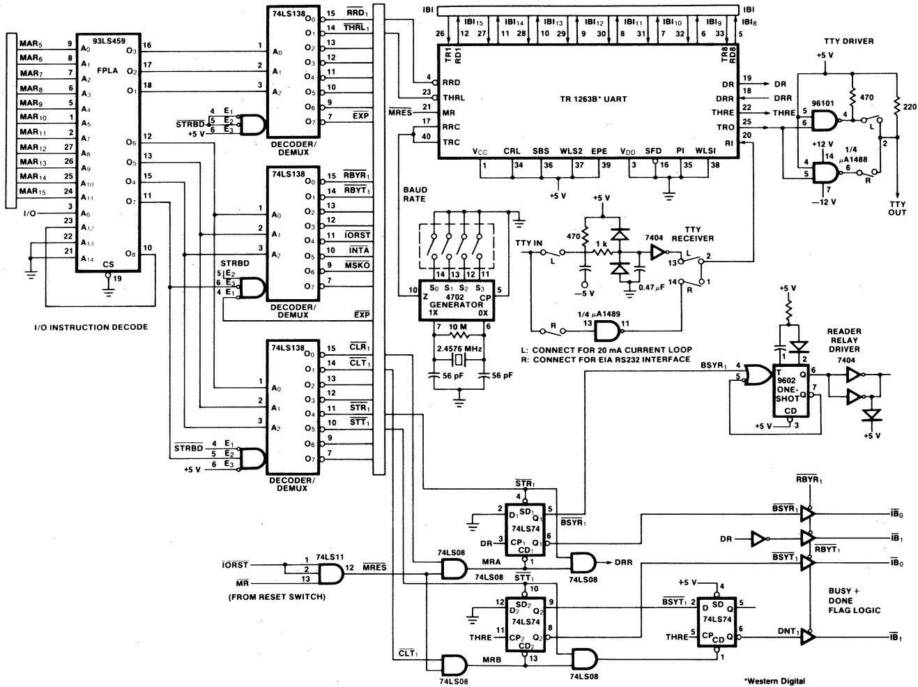
Fig. 8 F9445 Input/Output Connection Scheme (1 of 2)
