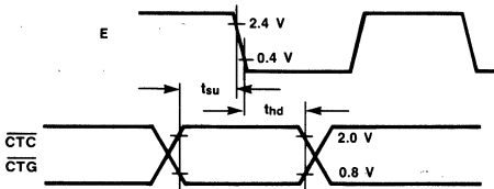
Fig. 9 Input Set-up and Hold Times
