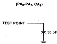
Fig. 7 CMOS Equivalent Test Load
