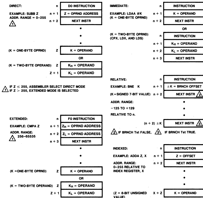
Fig. 19 Addressing Mode Summary
