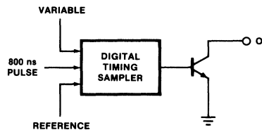
Fig. 16 Out-of-Lock Circuit
