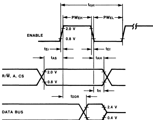
Fig. 1 Bus Read Timing (Read Information from F6848)
