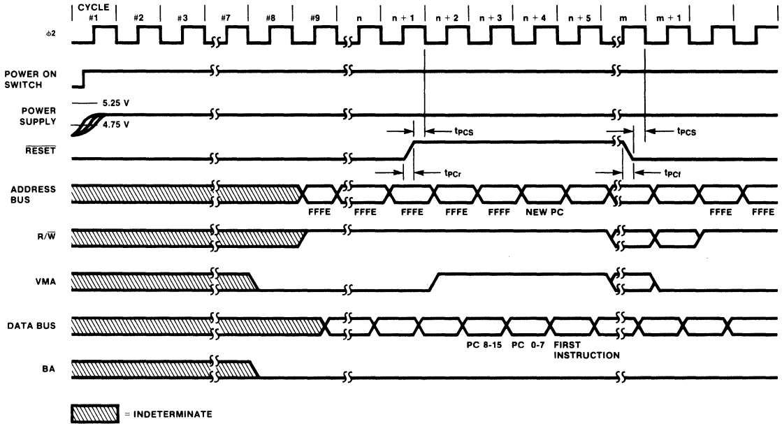
Fig. 2 Reset Timing
