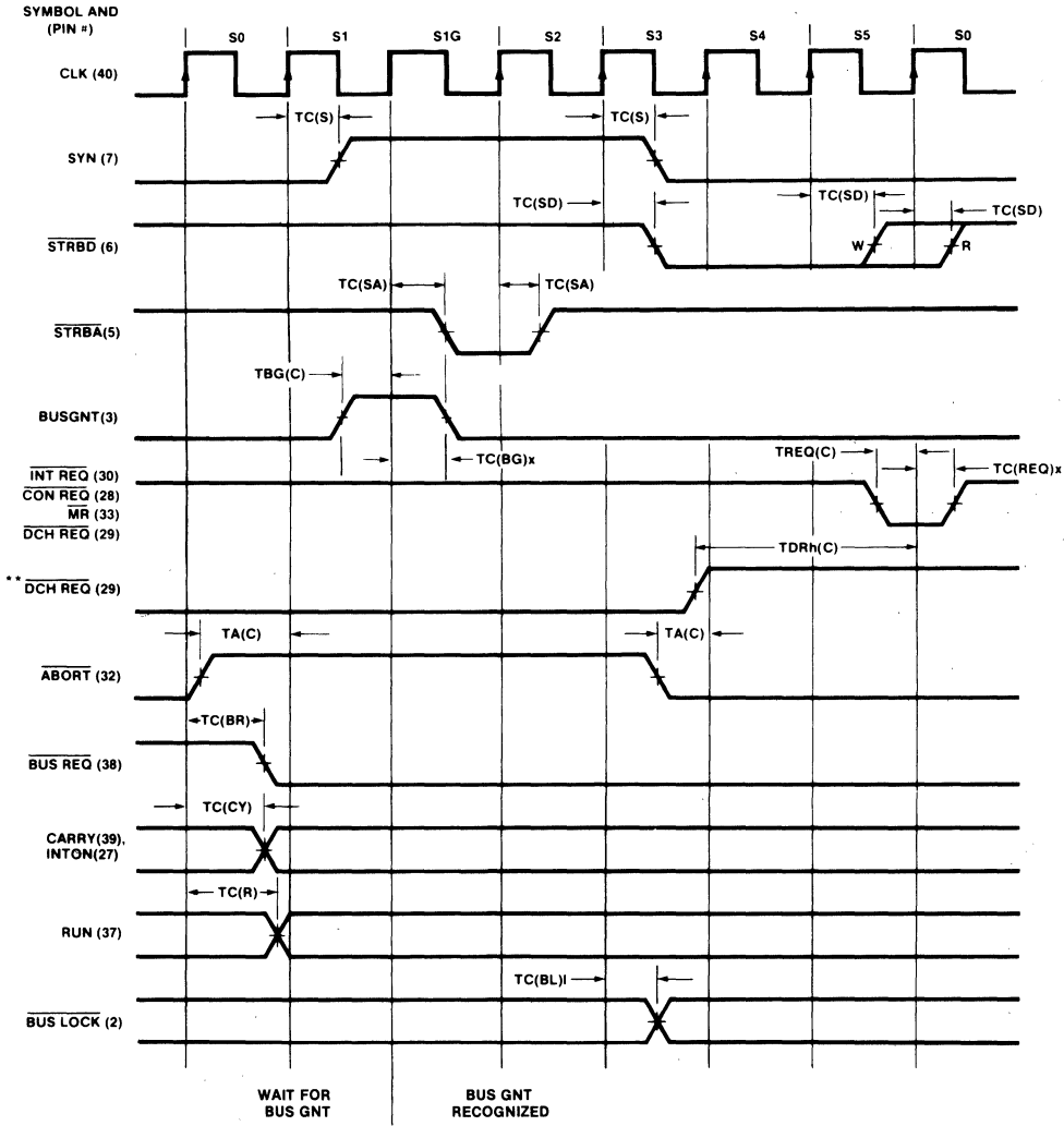
Figure 15. Bus and Status Control Timing*
