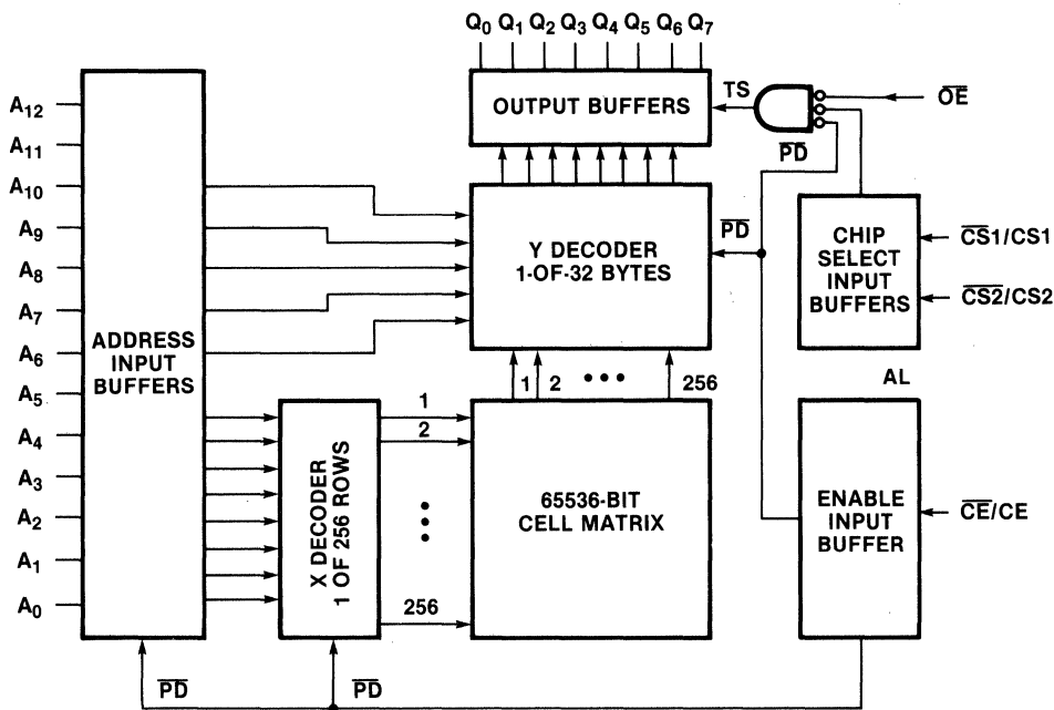
Figure 1 F3569 Block Diagram
