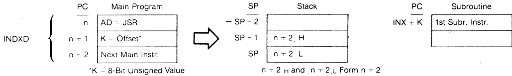
Fig. 12 Special Operations
