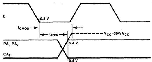
Fig. 12 Peripheral CMOS Data Delay Times (Write Mode; CRA-5 = CRA-3 = 1; CRA-4 = 0)
