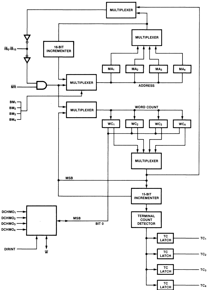
Fig. 1 F9449 Block Diagram
