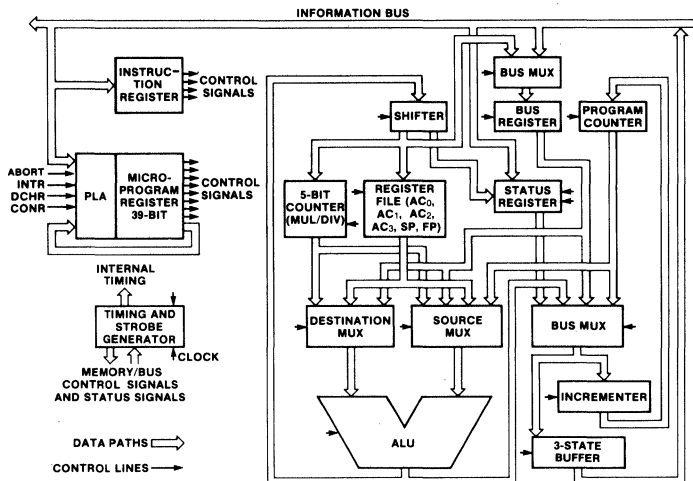
Fig. 1 F9445 Functional Diagram
