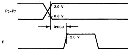
Fig. 6 Peripheral Port Set-up Time
