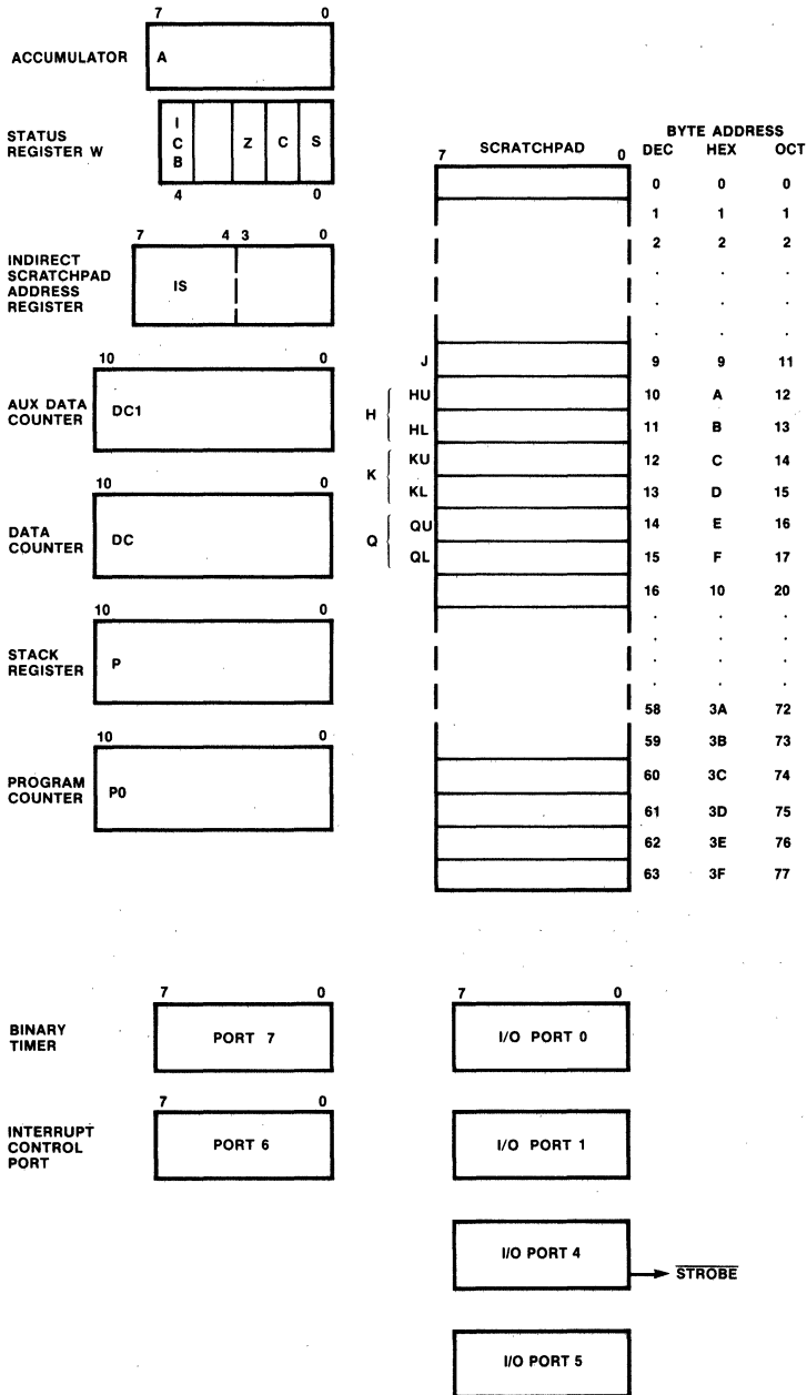
Fig. 6 Programmable Registers and Ports
