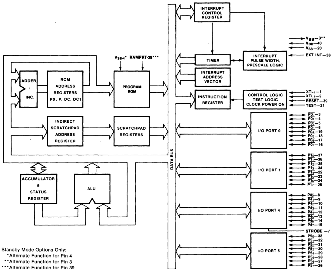
Fig. 2 F3872 Block Diagram
