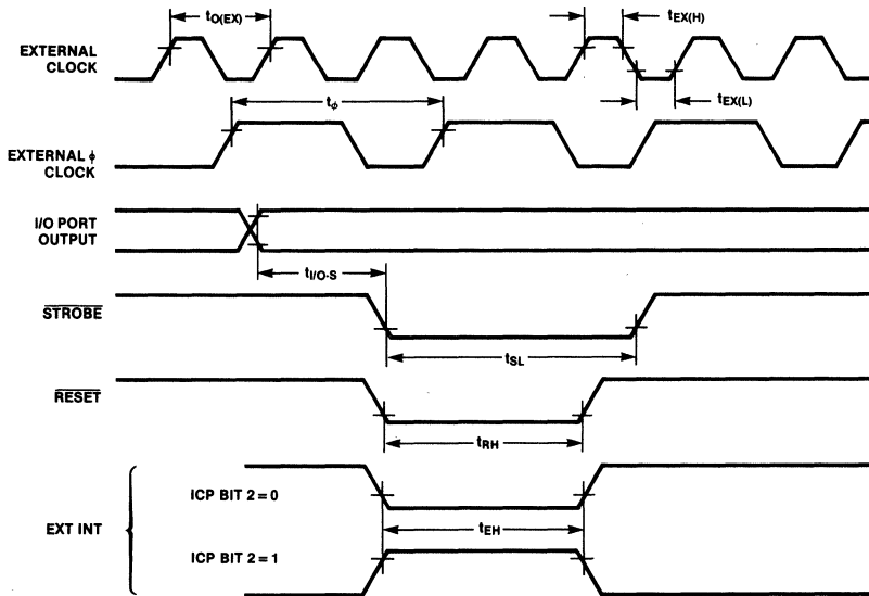
Fig. 9 Program/Verify Timing Diagrams
