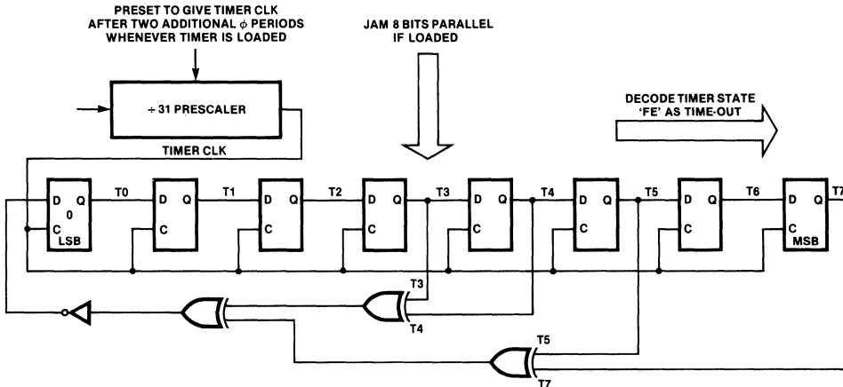
Fig. 6 Timer Block Diagram
