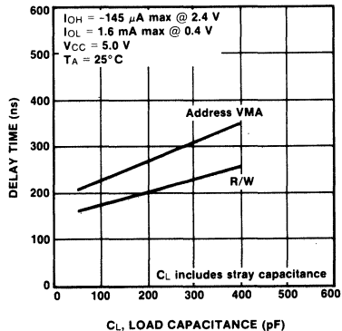
Fig. 14 Typical Read/Write, VMA and Address Output Delay vs. Capacitive Loading
