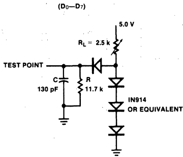
Fig. 5 Bus Timing Test Load
