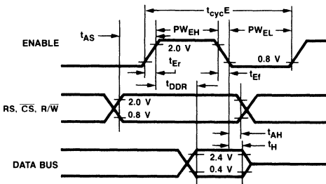
Fig. 4 Bus Read Timing Characteristics (Read Information from GPIA)
