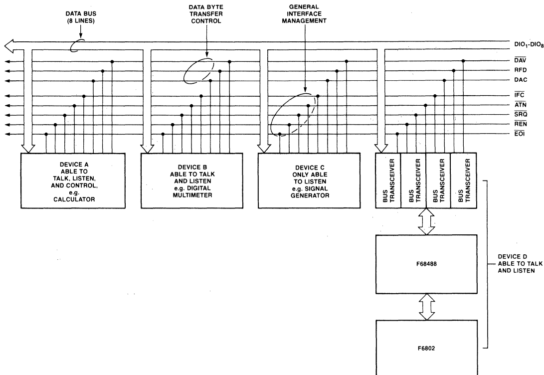
Fig. 1. Functional Diagram
