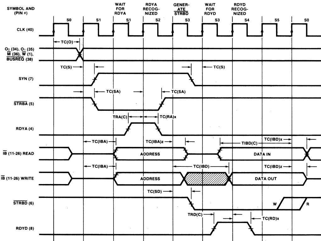
Fig. 14 Extended Memory Cycle Timing*
