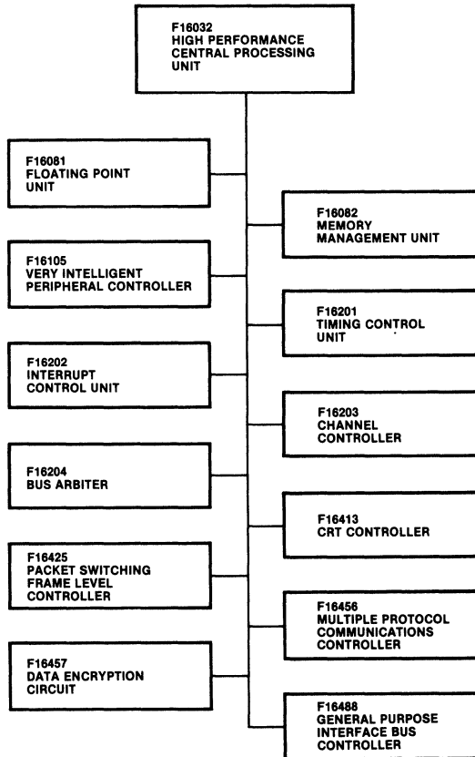
Figure 7-1 F16000 Microprocessor Family Organization
