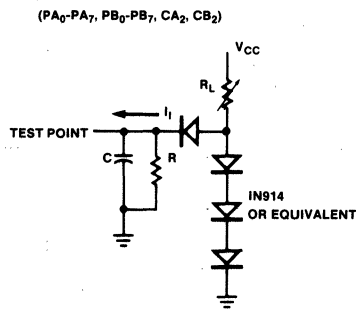
Fig. 6 TTL Equivalent Test Load
