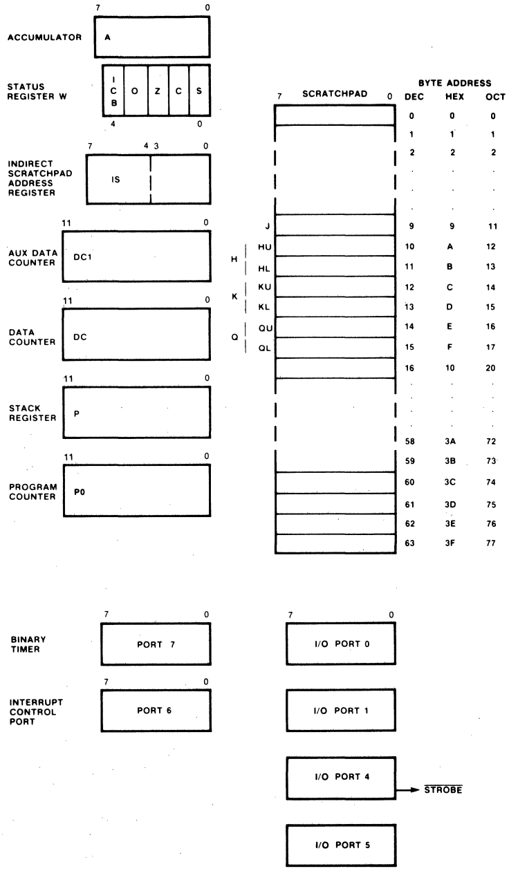
Fig. 8 Programmable Registers and Ports
