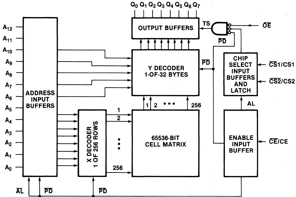
Figure 1 F3568 Block Diagram
