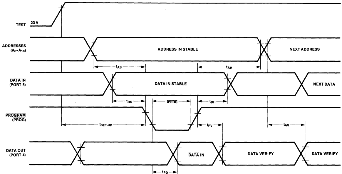
Fig. 8 Timing Diagrams
