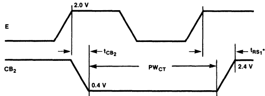
Fig. 14 CB_2 Delay Time (Write Mode; CRB-5 = CRB-3 = 1 ; CRB-4 = 0 )
