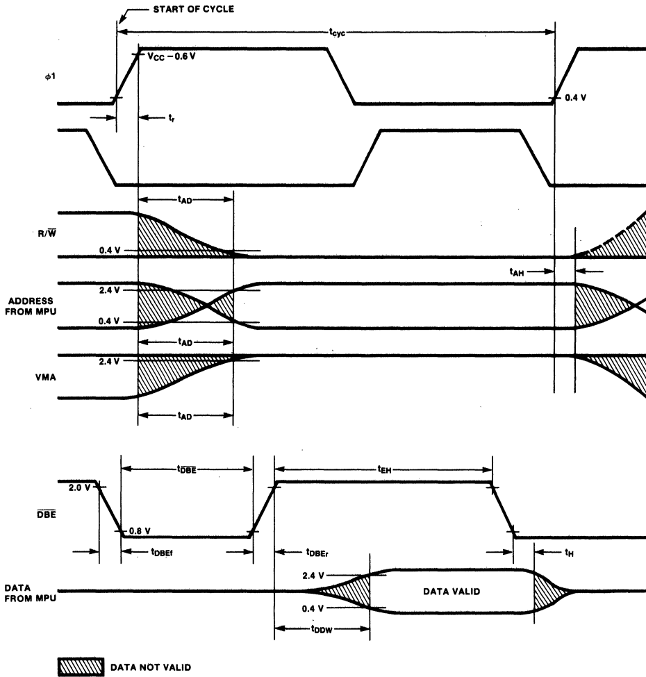
Fig. 29 Write In Memory or Peripherals
