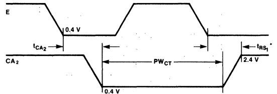
Fig. 10 CA 2 Delay Time (Read Mode; CRA-5 = CRA-3 = 1; CRA-4 = 0)
