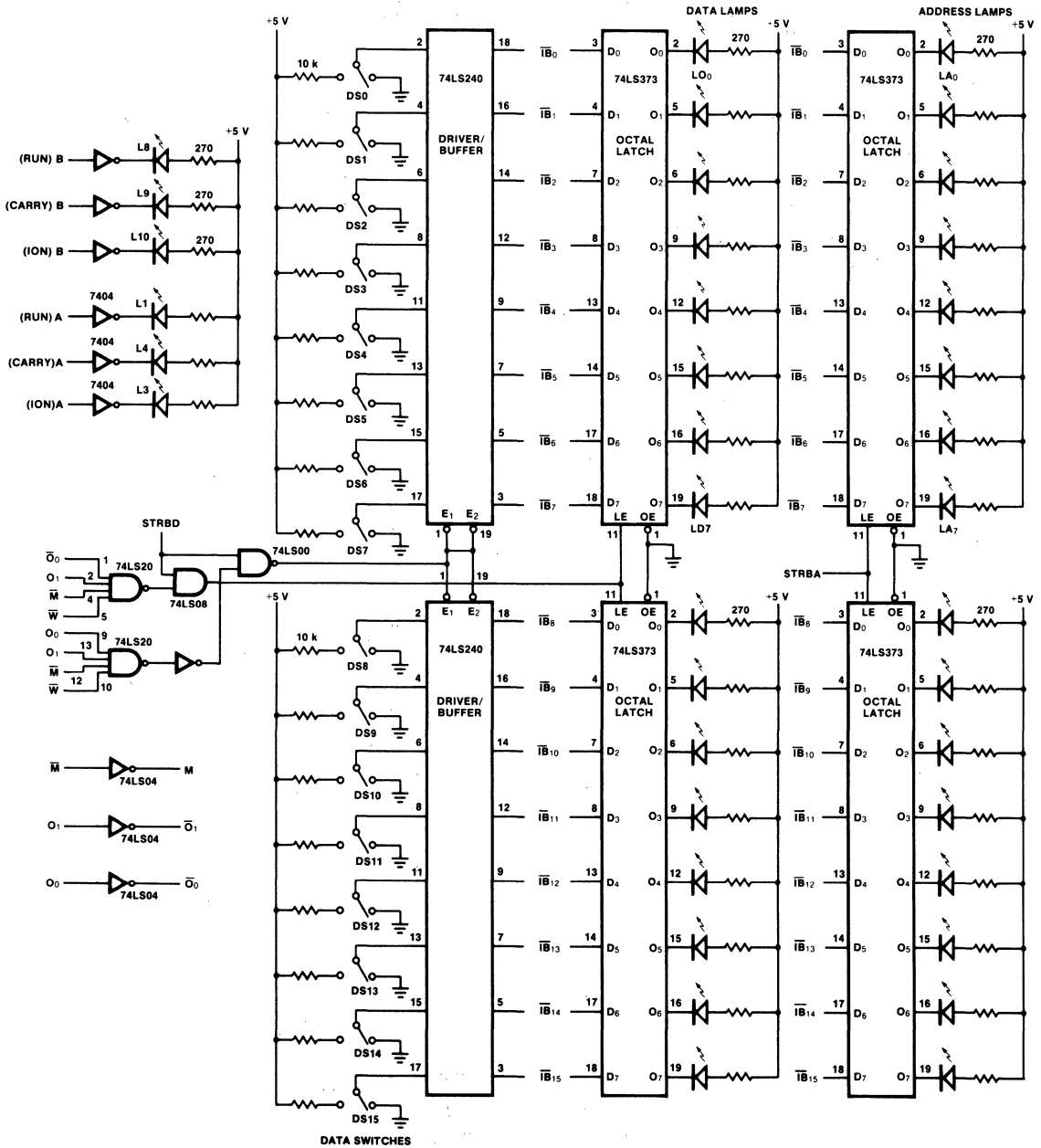
Fig. 10 F9445 Console Connection Scheme (3 of 3)
