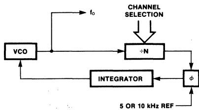
Fig. 7 Basic PLL Circuit
