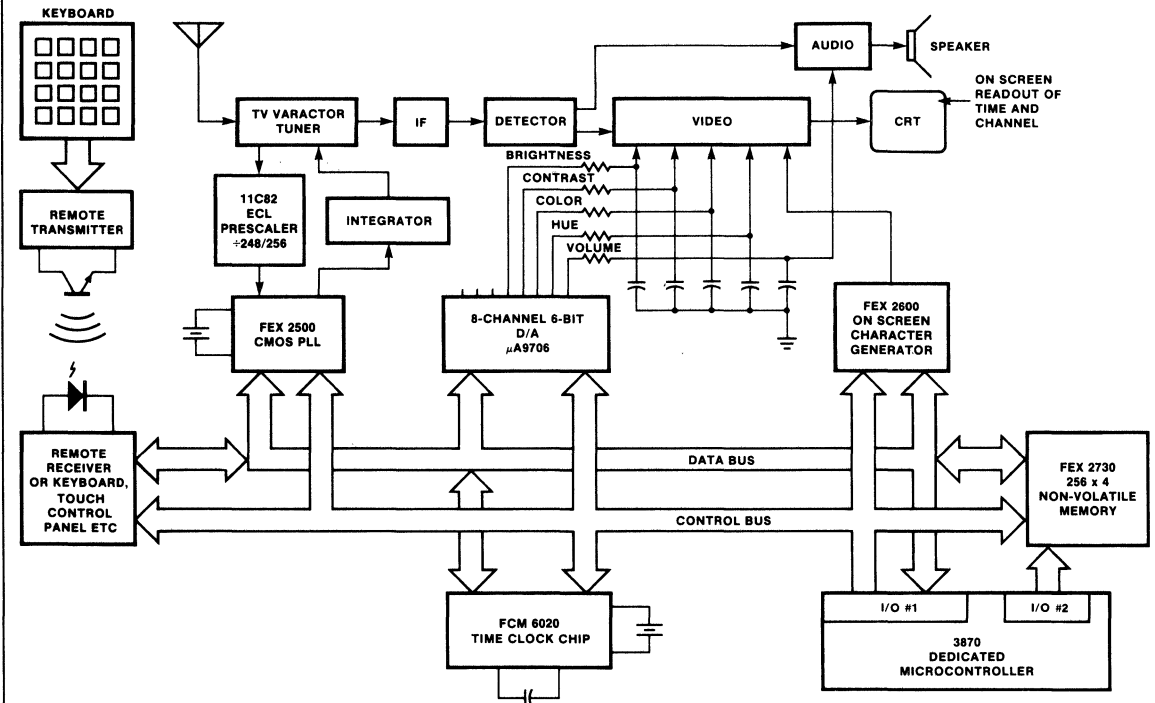
Fig. 5 Microprocessor-Controlled TV with PLL Tuning
