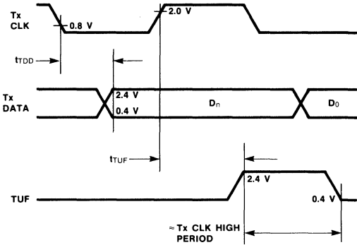
Fig. 4 Transmit Data Output Delay and Transmitter Underflow Delay Time
