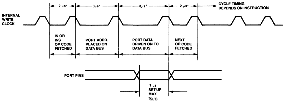
Fig. 11 Port Input/Output Timing Diagrams
