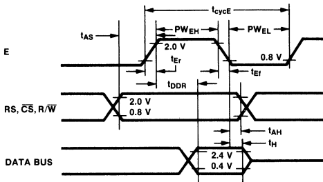
Fig. 2 Bus Read Timing Characteristics (Read Information from PTM)
