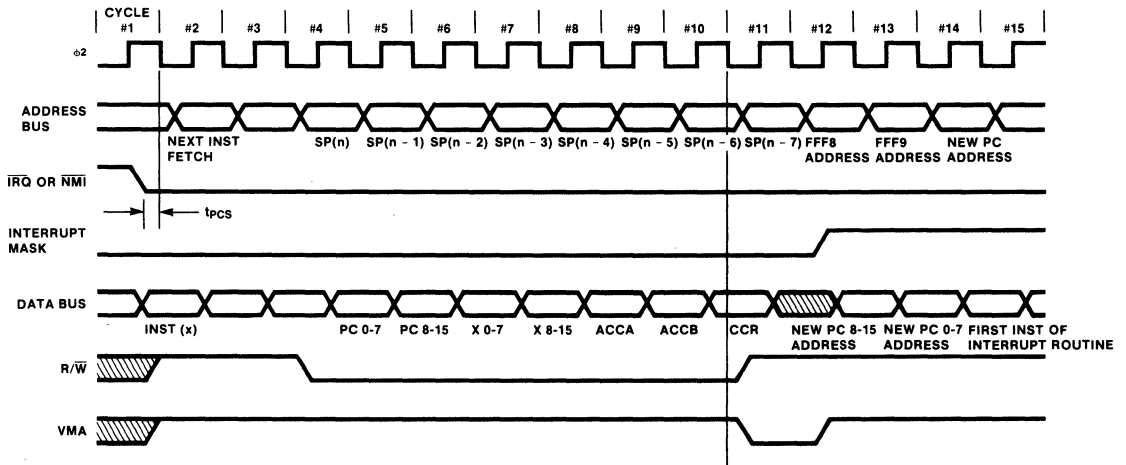
Fig. 3 Interrupt Timing
