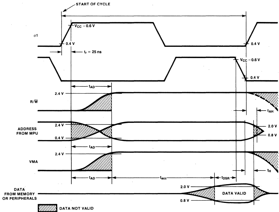
Fig. 28 Read Data From Memory or Peripherals
