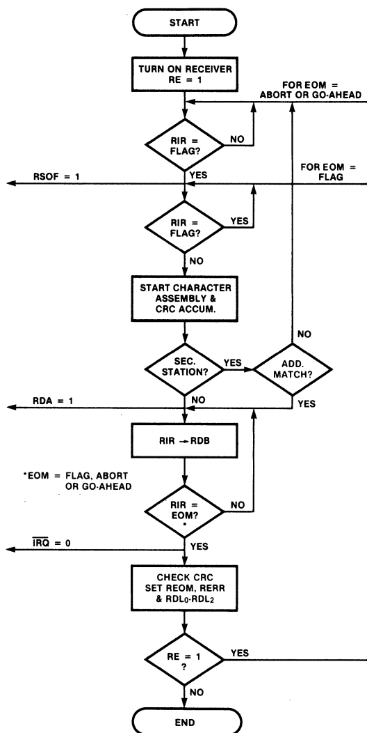
Fig. 4 BOP Receive Flow Chart
