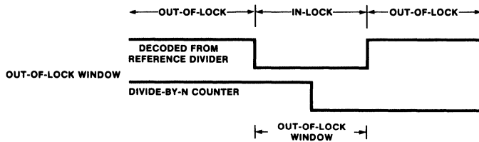
Fig. 17 Out-of-Lock Timing Diagram
