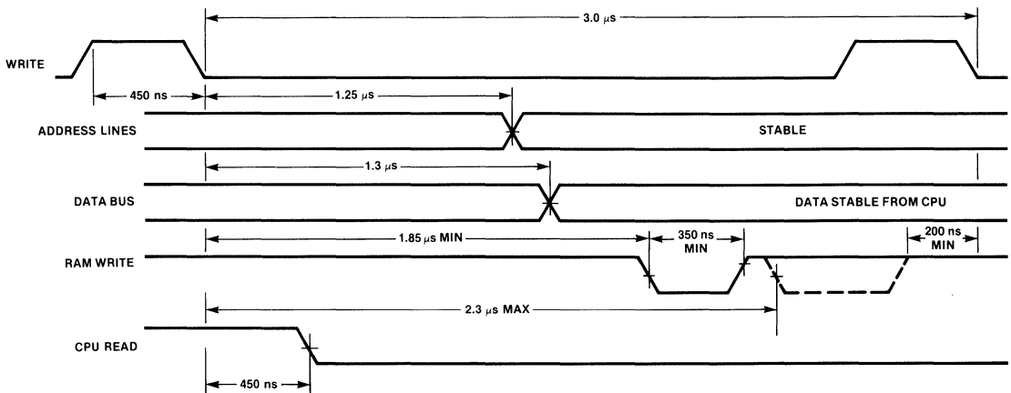
Fig. 18 SMI Timing Signals Output During a Write-to-Memory
