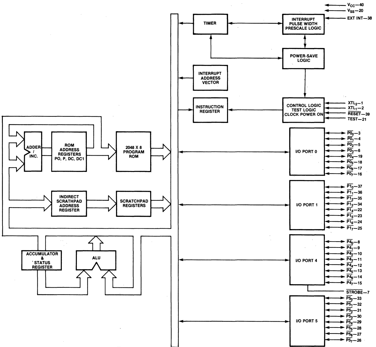
Figure 1 Block Diagram
