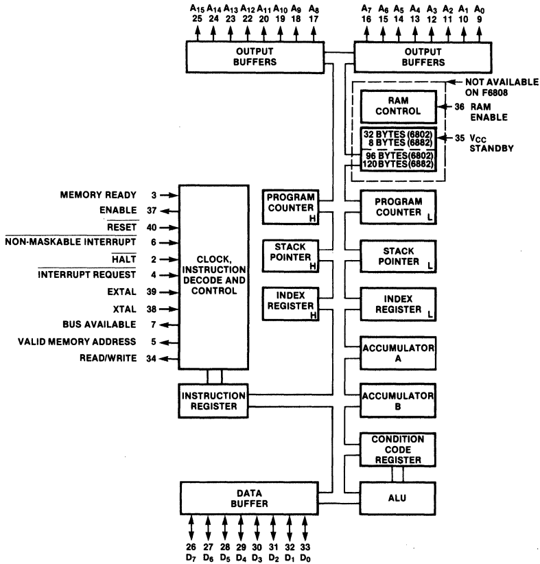
Fig. 2 F6802/F6882 Block Diagram
