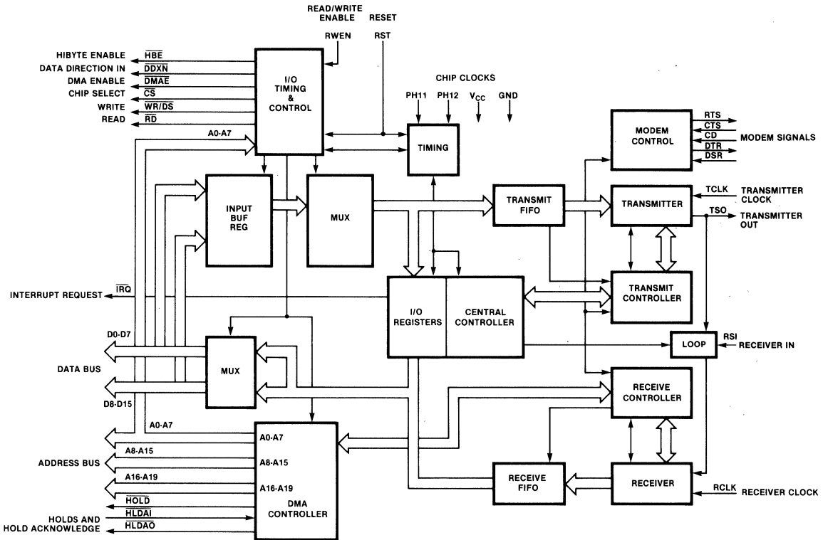
Figure 1 16425 Block Diagram
