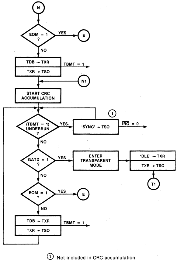
Fig. 11b BISO SYNC Transmit
