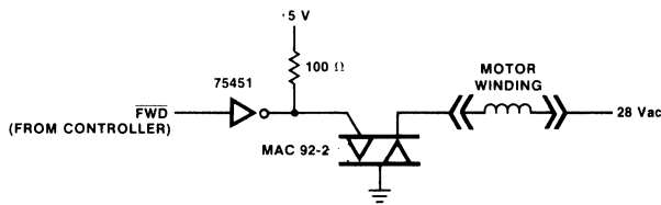
Fig. 3 Forward Triac Interface Circuit
