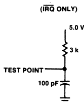
Fig. 8 NMOS Equivalent Test Load
