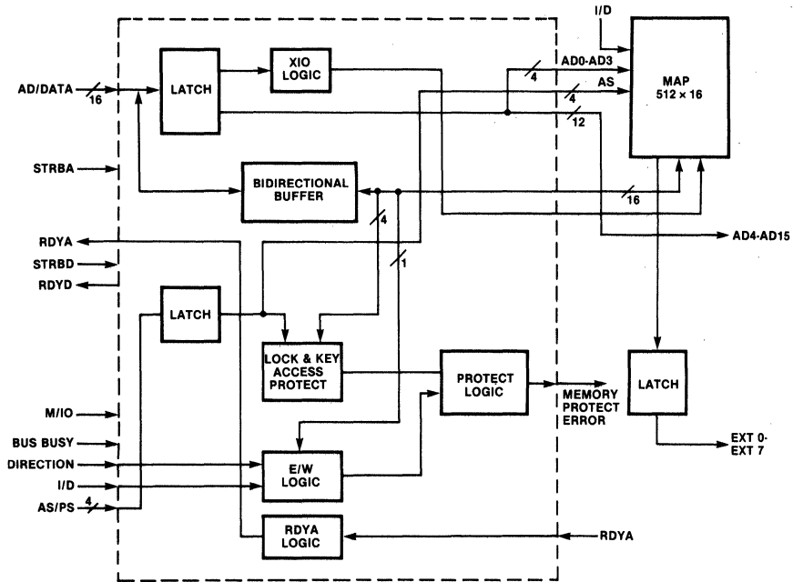
Figure 2 F9451 MMU Block Diagram
