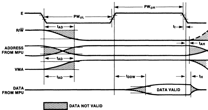
Fig. 16 Write Data in Memory or Peripherals
