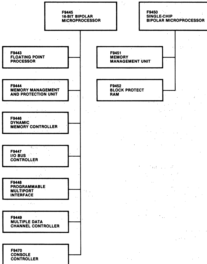
16-BIT I 3 L BIPOLAR MICROPROCESSOR FAMILY ORGANIZATION
