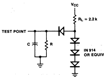
Fig. 32 Bus Timing Test Loads
