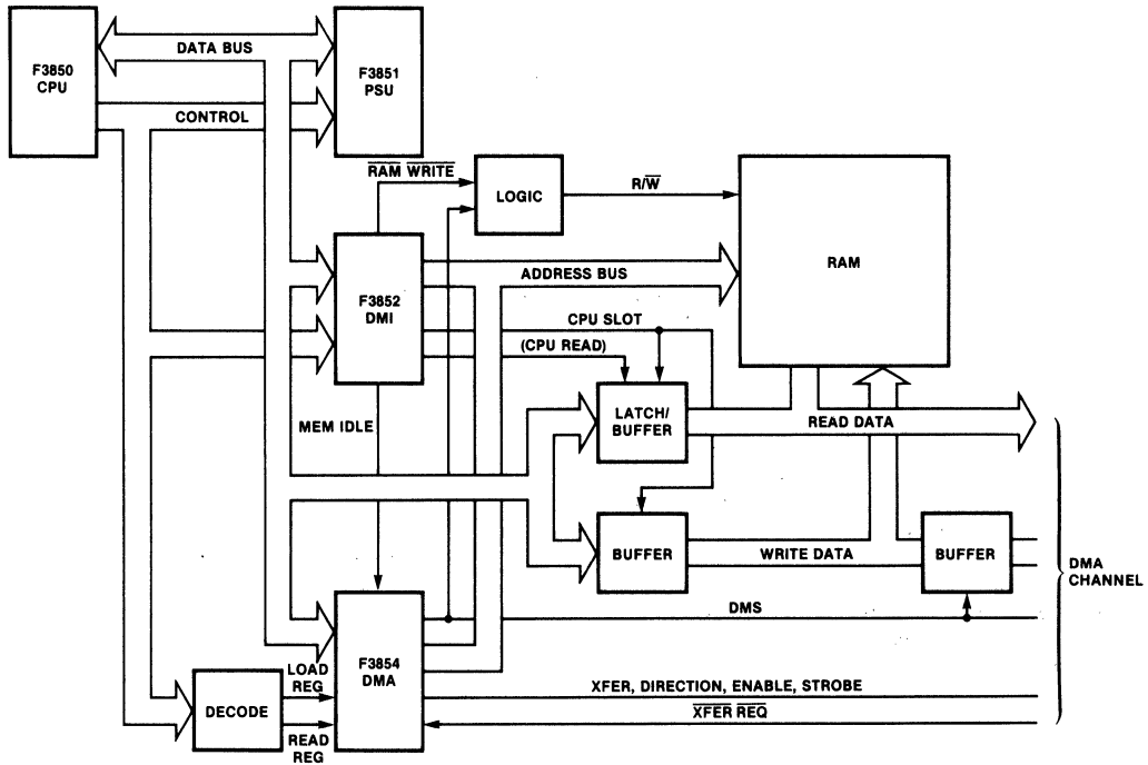
Fig. 2 Typical DMAC Configuration
