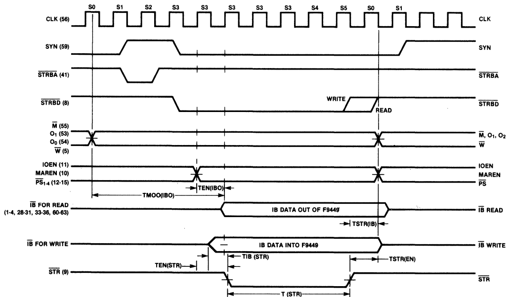
Fig. 5 Programmed I/O Timing
