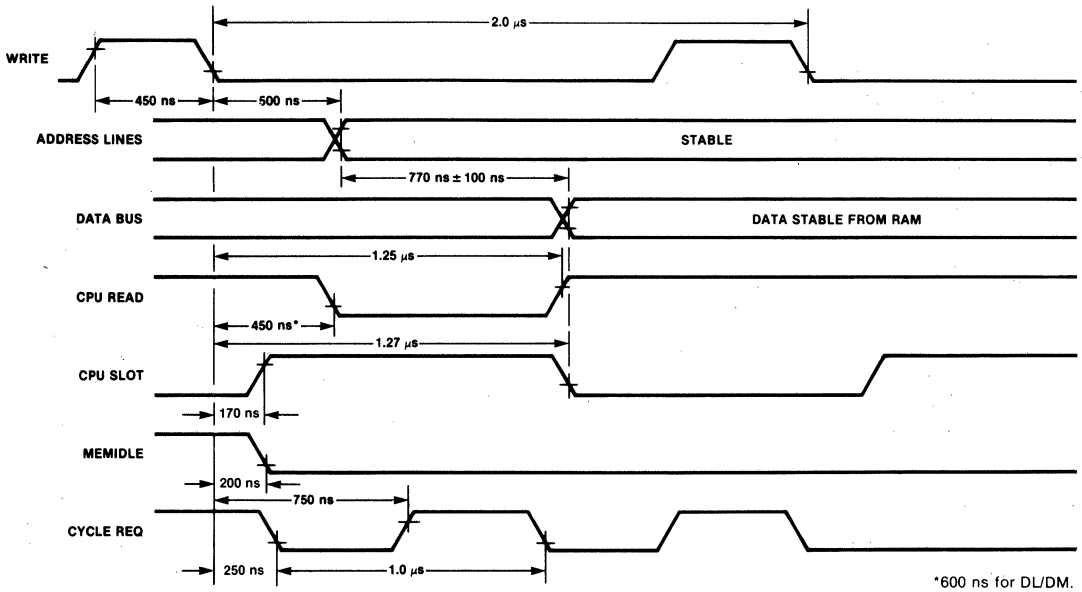
Fig. 11 DMI Timing Signals Output During Short-Cycle Memory Read, with Address from Program Counter
