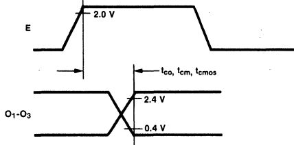
Fig. 7 Output Delay
