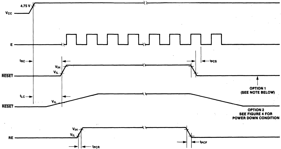
Fig. 5 Power-Up and Reset Timing
