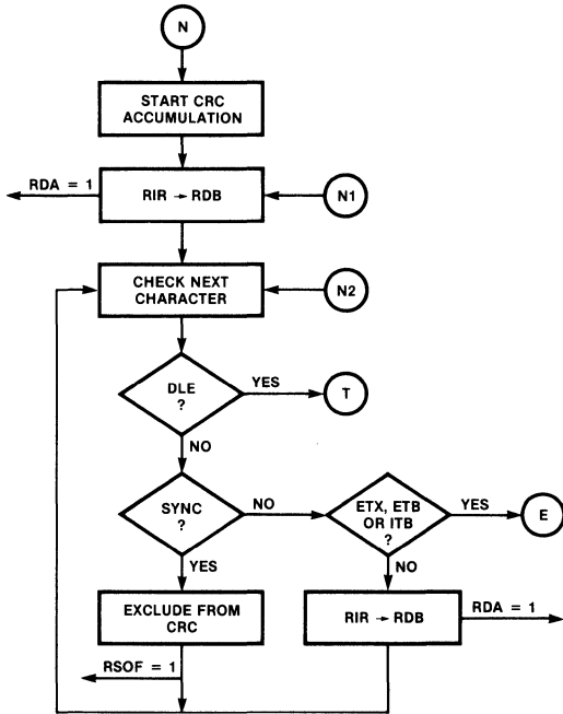
Fig. 6b BISYNC Receive
