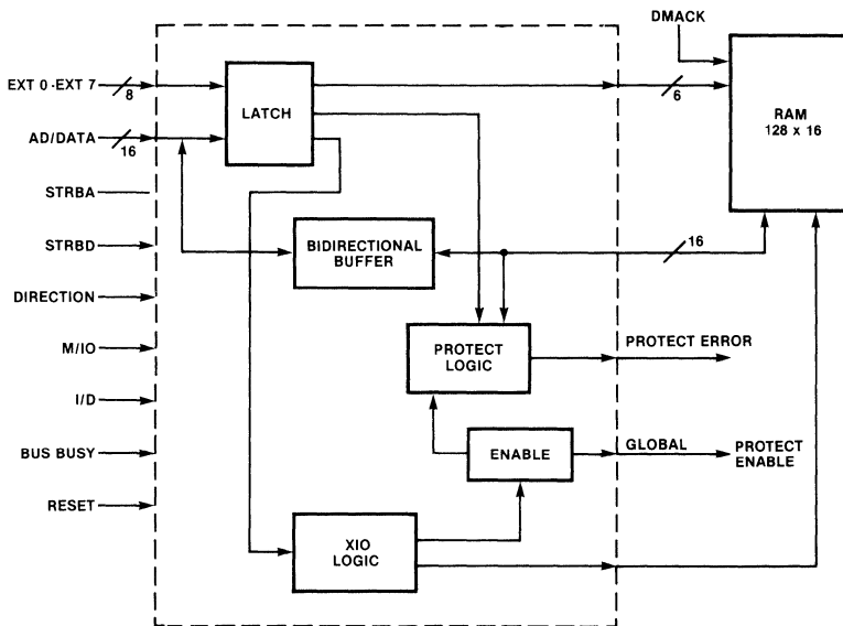
Figure 1 F9452 Block Diagram
