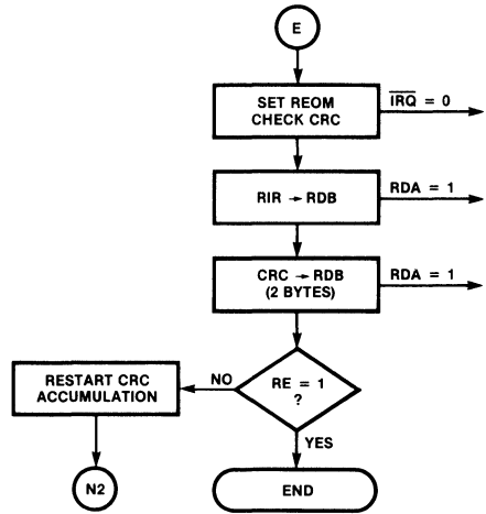
Fig. 6c BISYNC Receive
