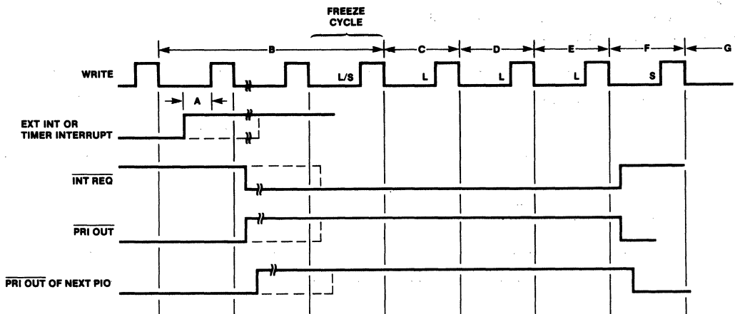
Figure 5 Interrupt Sequence
