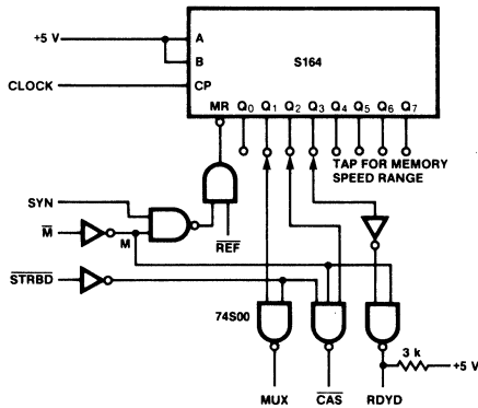
Fig. 9 F9445 Dynamic Memory Connection Scheme
