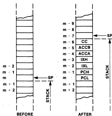
Fig. 4 Saving the Status of the Microprocessor in the Stack
