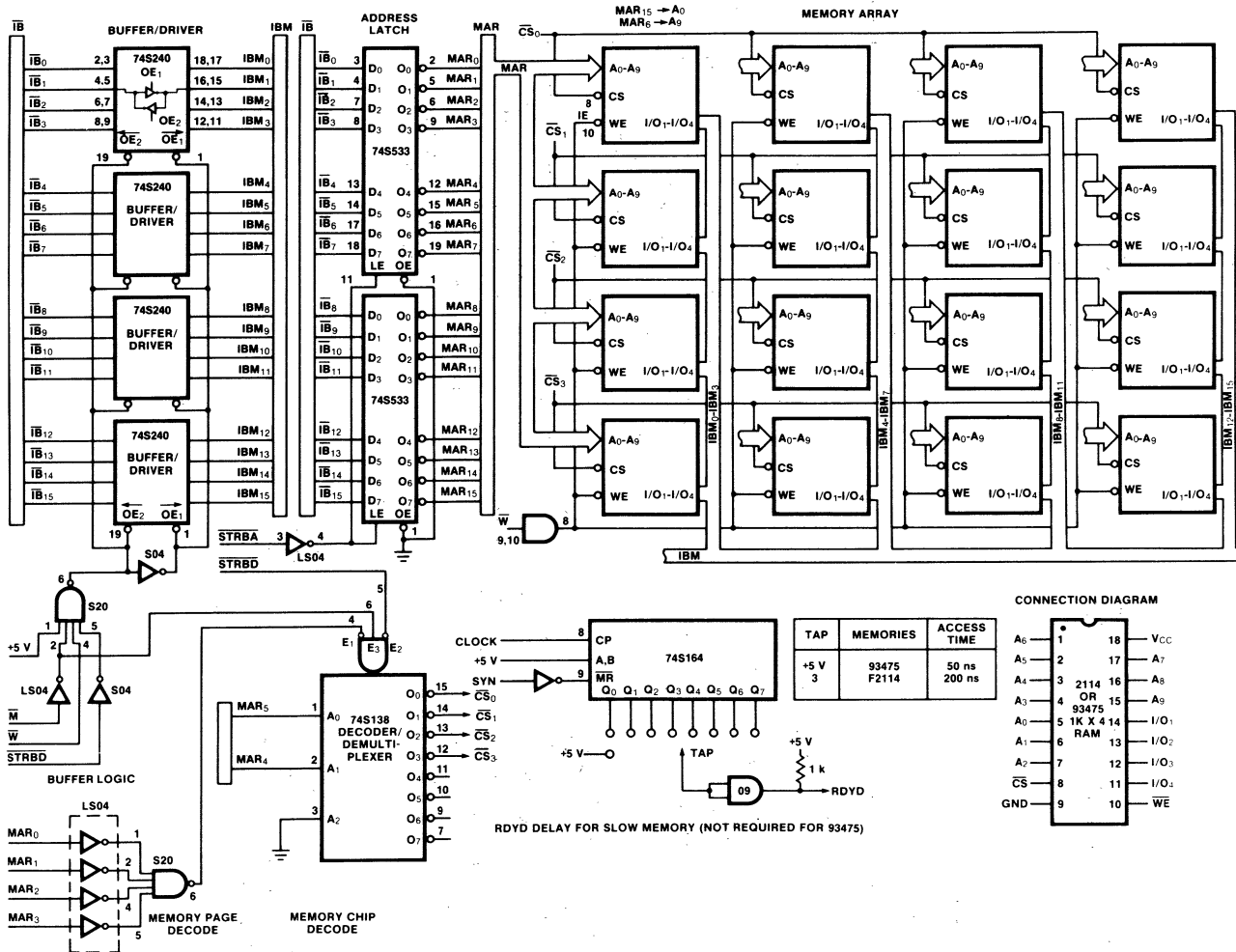
Fig. 7 Static Memory Connection Scheme
