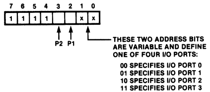
Fig. 4 DMAC I/O Port Address
