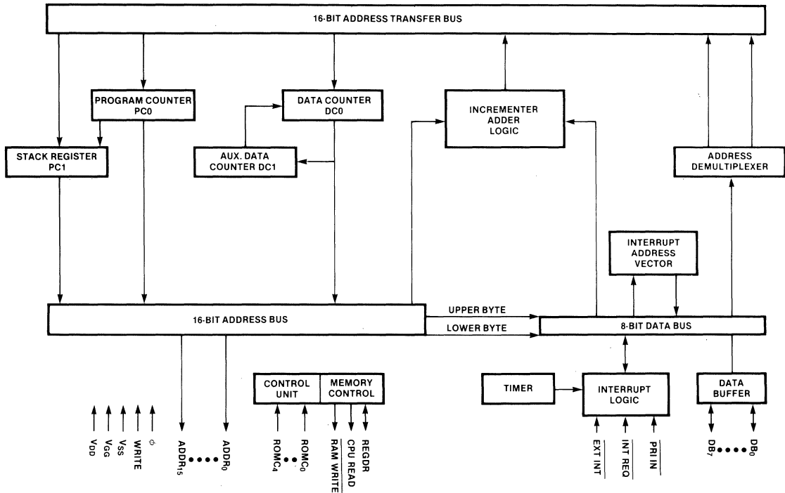
Fig. 2 F3853 SMI Logic Organization
