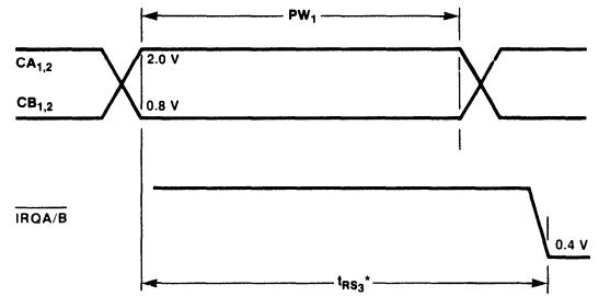
Fig. 16 Interrupt Pulse Width and \overline{IRQ} Response
