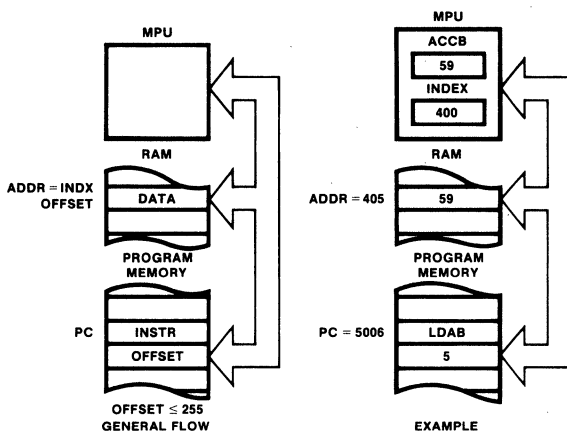
Fig. 26 Indexed Addressing Mode
