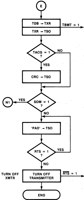
Fig. 11d BISYNC Transmit
