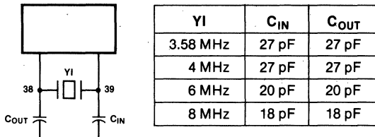
Fig. 8 Crystal Specification
