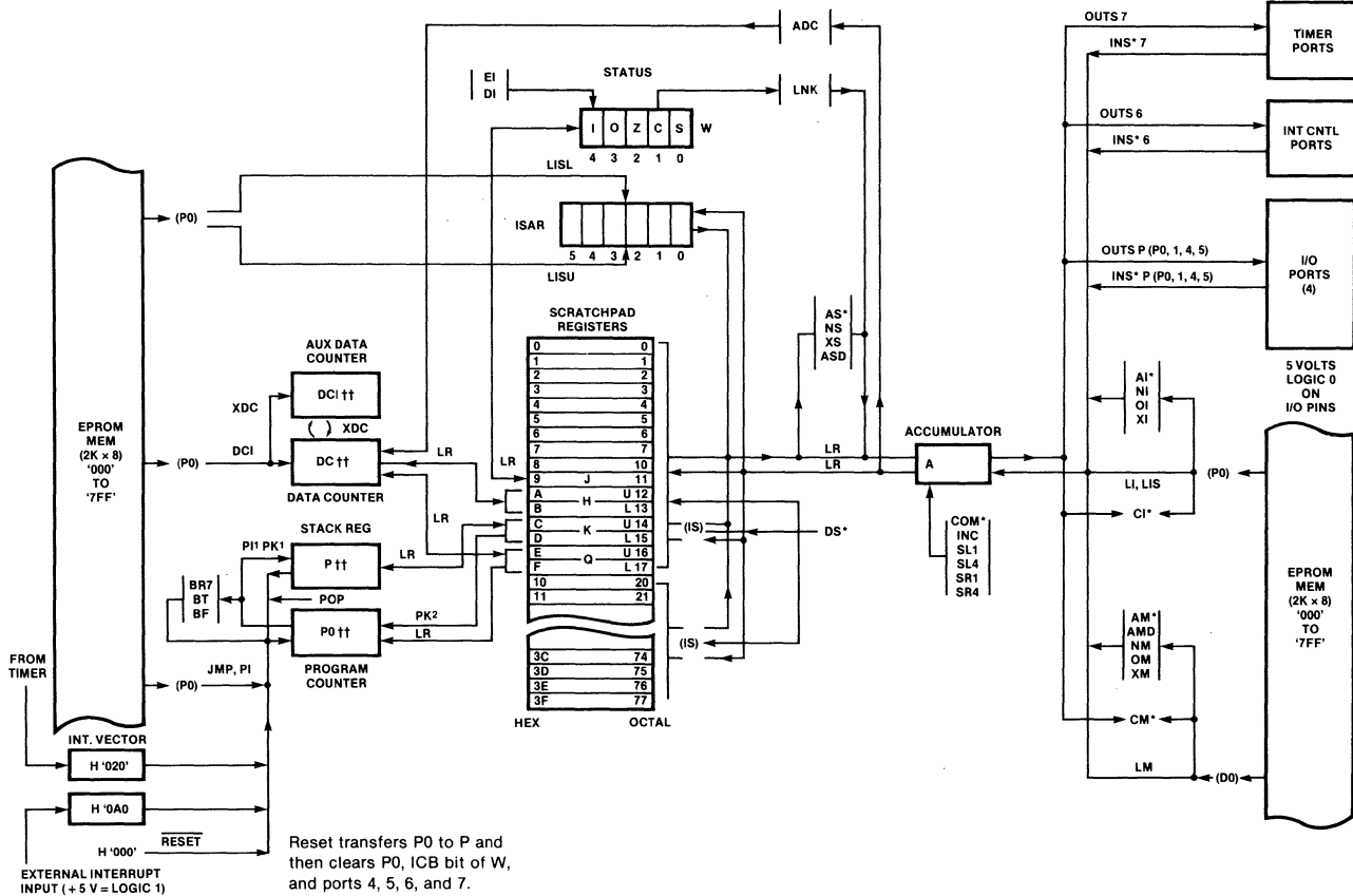
Fig. 7 Programming Model
