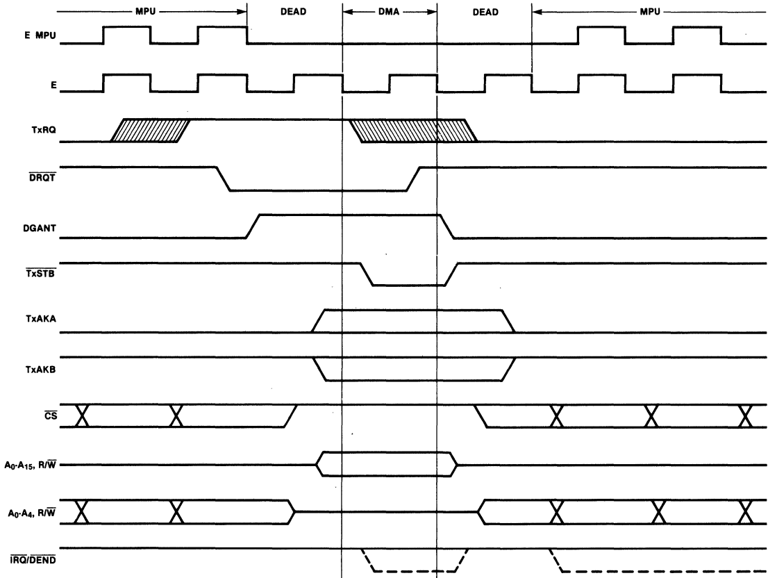
Fig. 2 TSC Steal Mode Timing
