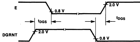
Fig. 11 DGRNT Input Timing
