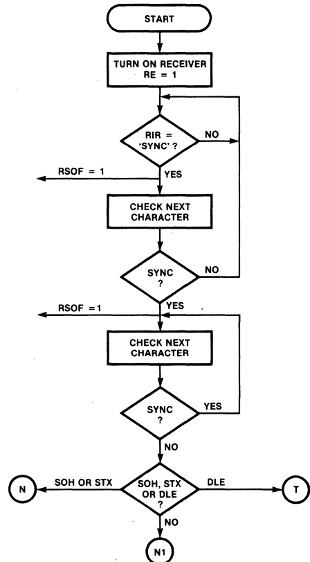
Fig. 6a BISO SYNC Receive
