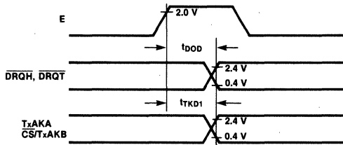
Fig. 12 DRQH, DRQT, TxAK Output Timing
