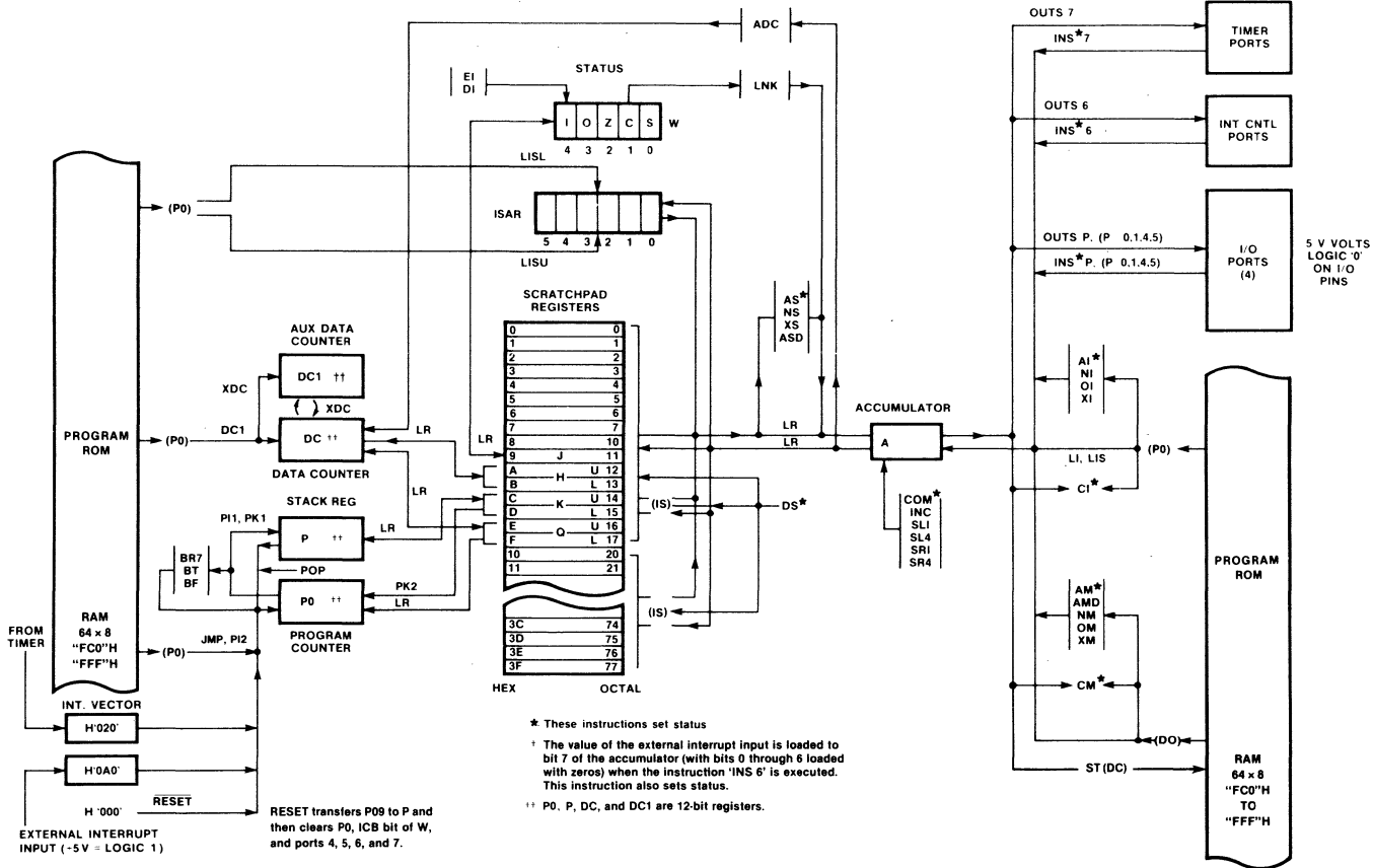
Fig. 9 Programming Model
