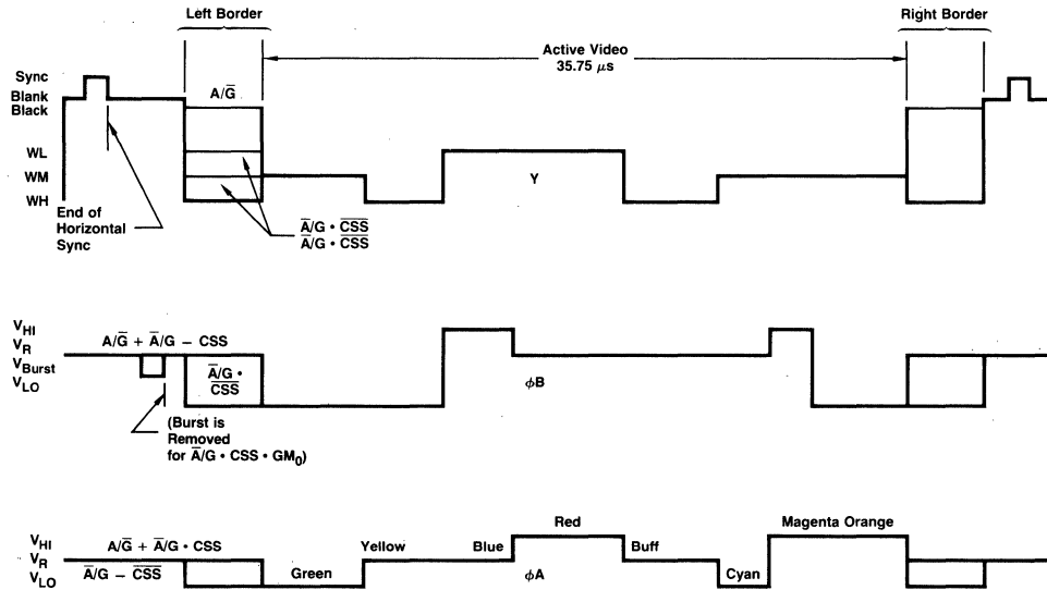
Fig. 3 Timing Diagrams
