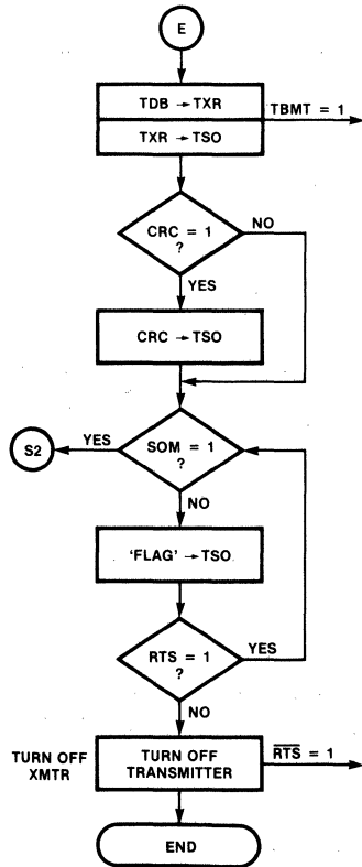
Fig. 10c BOP Transmit
