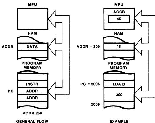
Fig. 24 Extended Addressing Mode
