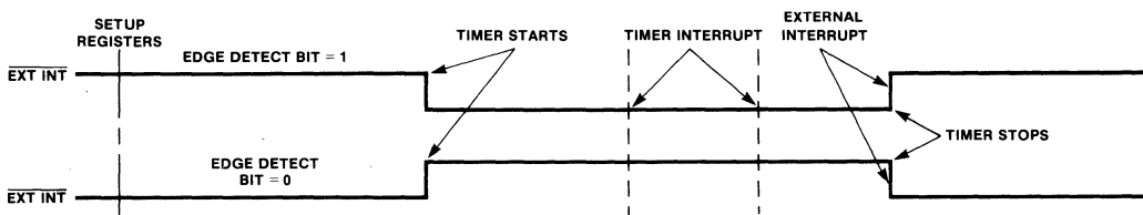
Figure 12 F3856 Pulse Width Measurement
