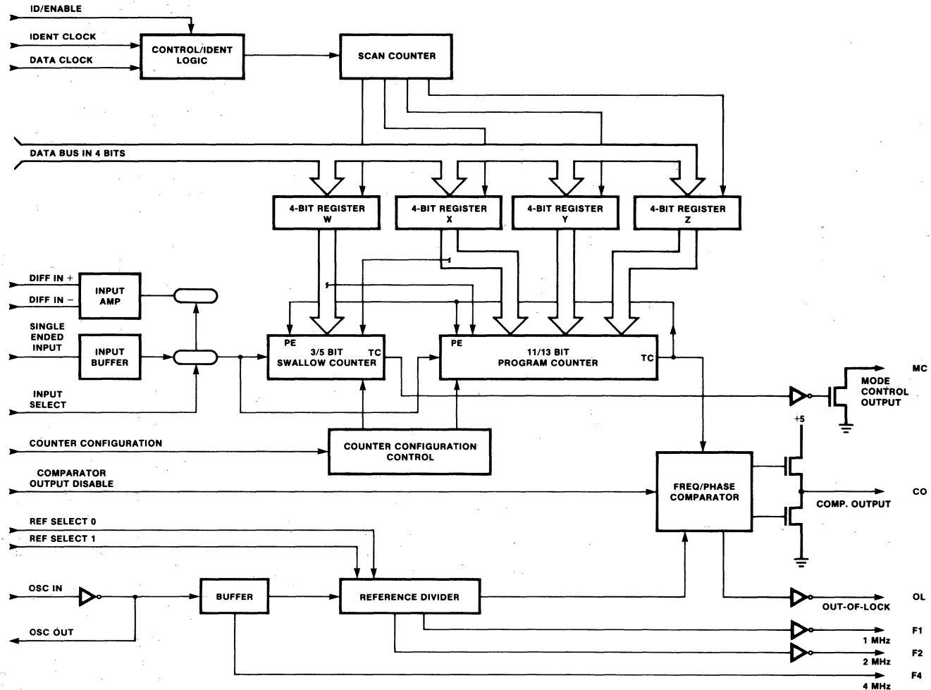
Fig. 12 FEX2500 PLL Block Diagram
