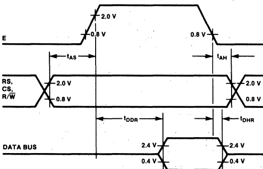
Fig. 3 Bus Timing Characteristics (Read from PIA)
