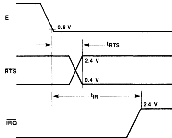
Fig. 6 Request-to-Send Delay and Interrupt Request Release Times
