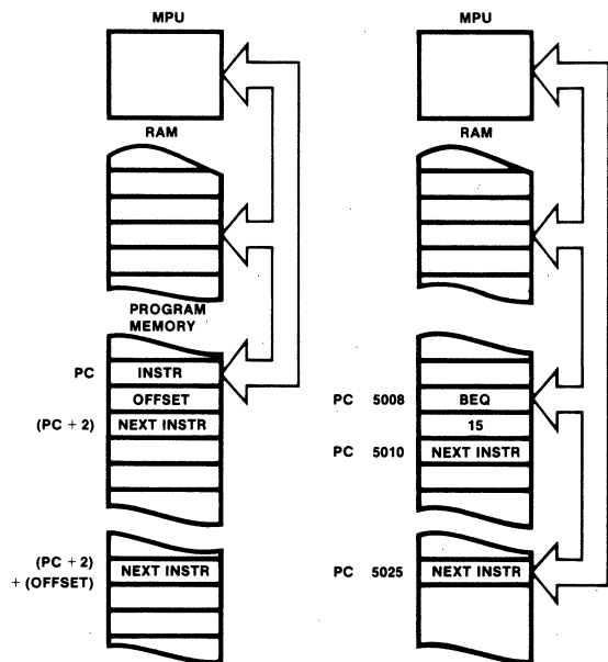
Fig. 25 Relative Addressing Mode
