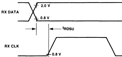
Fig. 4 Receive Data Set-up Time ( \div 1 Mode)
