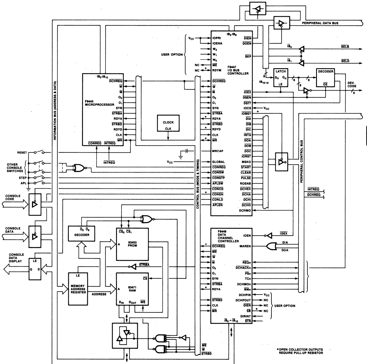
Fig. 3 F9449/F9447 Configuration
