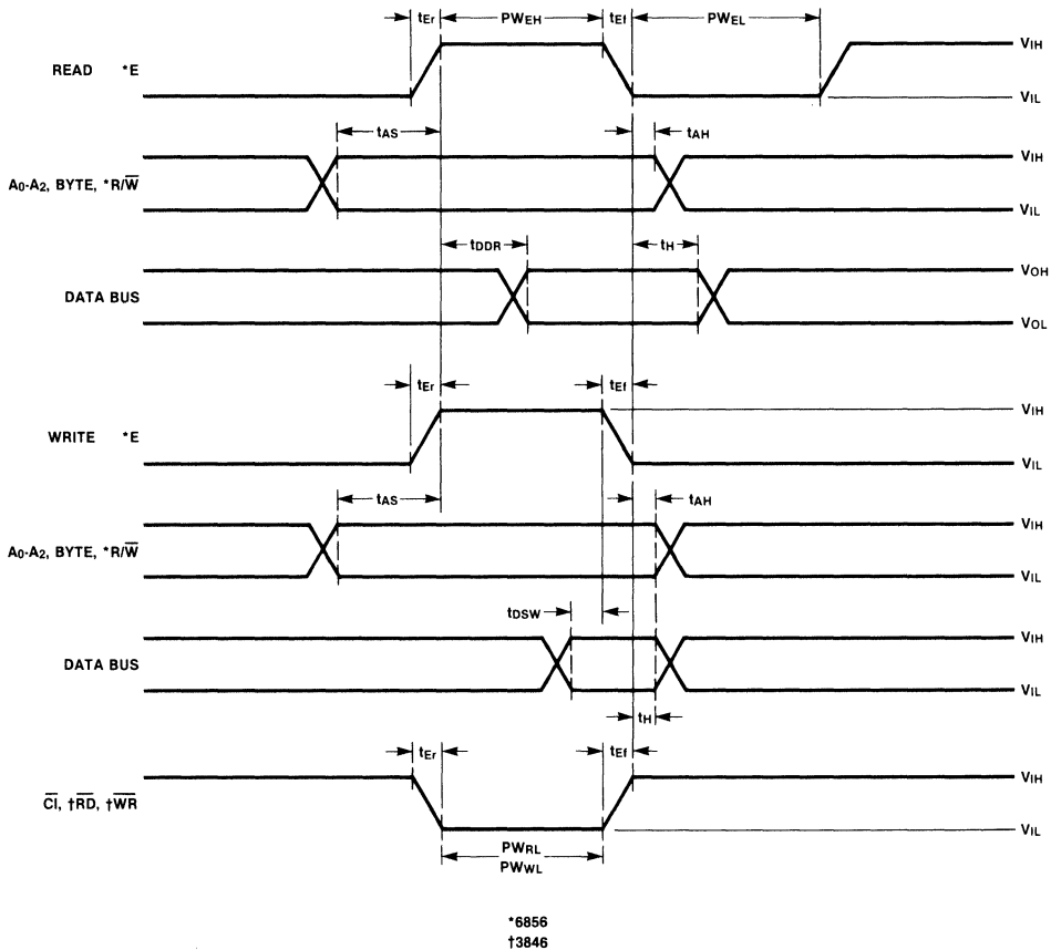
Fig. 14 Read/Write Timing Diagram
