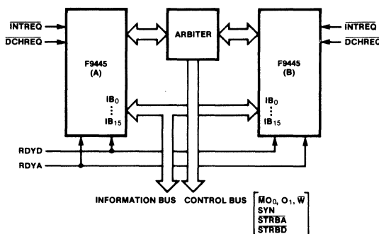
Fig. 11 A Possible General Multiprocessor Scheme
