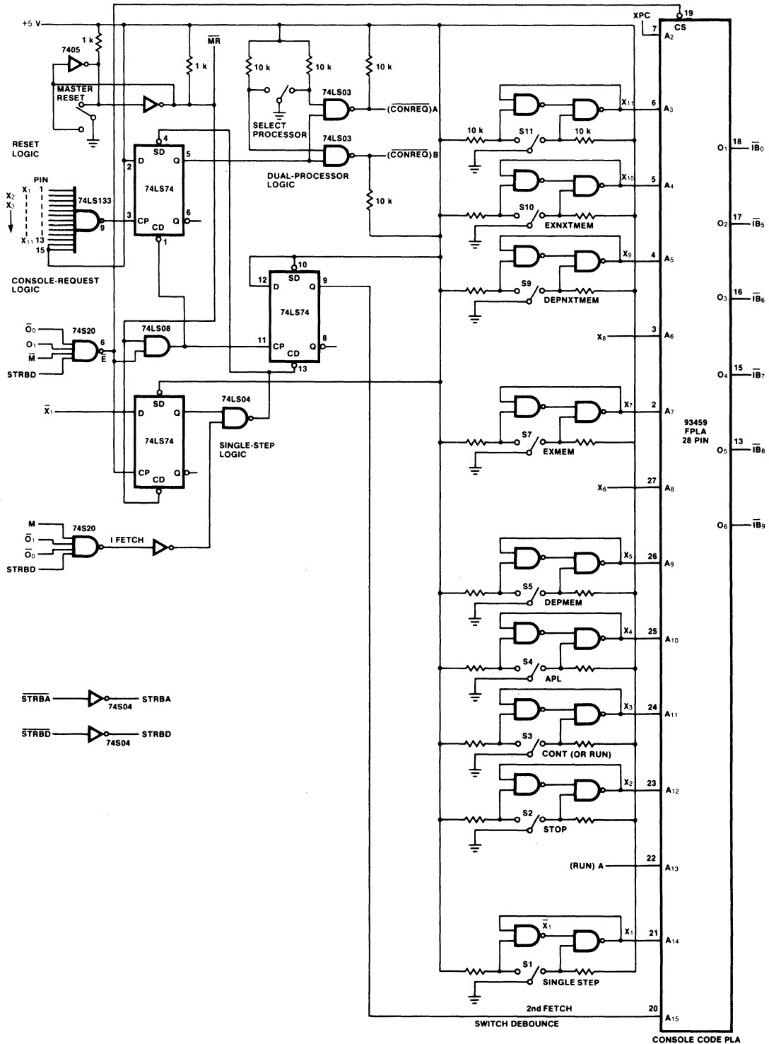
Fig. 10 F9445 Console Connection Scheme (2 of 3)
