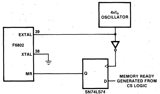
Fig. 10 Memory Ready Synchronization
