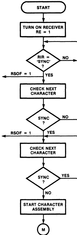
Fig. 8a BCP Receive
