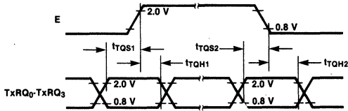
Fig. 10 TxRQ Input Timing
