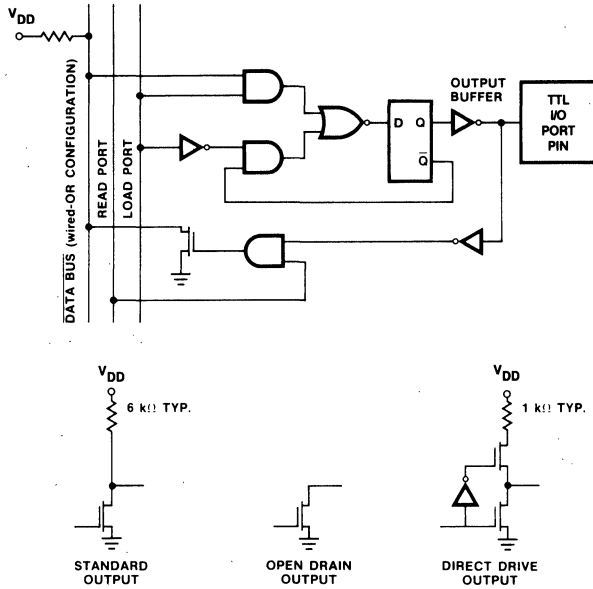
Figure 2 F3871 I/O Pin Diagram with Output Buffer Options
