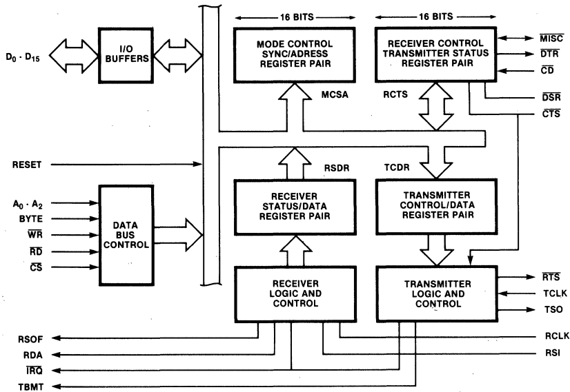
Figure 1 F16456 Block Diagram
