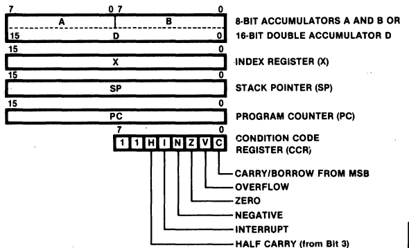
Figure 5-3 F6801/F6803 Programming Model
