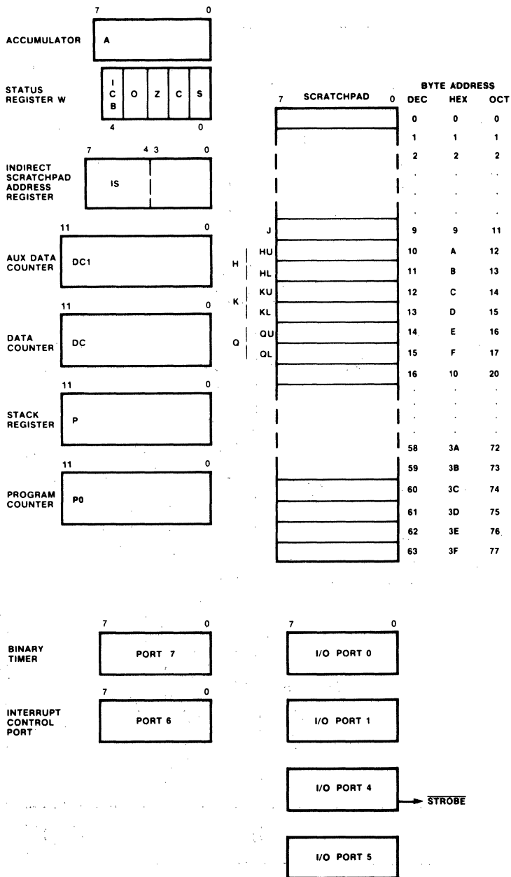
Fig. 7 Programmable Registers and Ports
