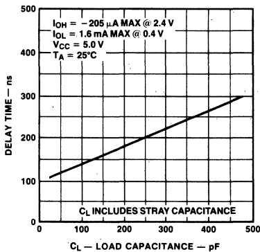
Fig. 30 Typical Data Bus Output Delay vs Capacitive Loading ( t_{BDW} )
