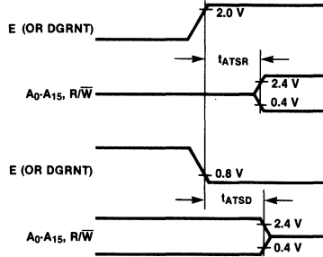
Fig. 14 Address Three-state Timing
