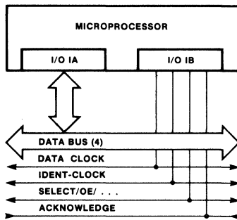
Fig. 4 Standardized Bus System
