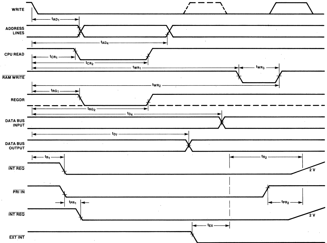
Fig. 10 F3853 SMI Timing Signals
