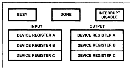
Fig. 4 I/O Device Model
