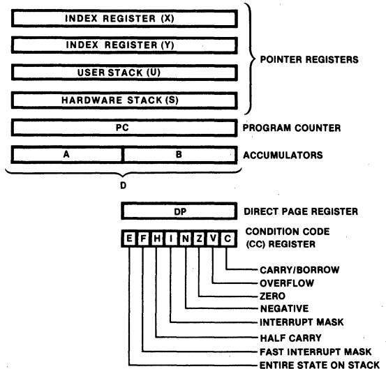
Figure 5-4 F6809 Programming Model
