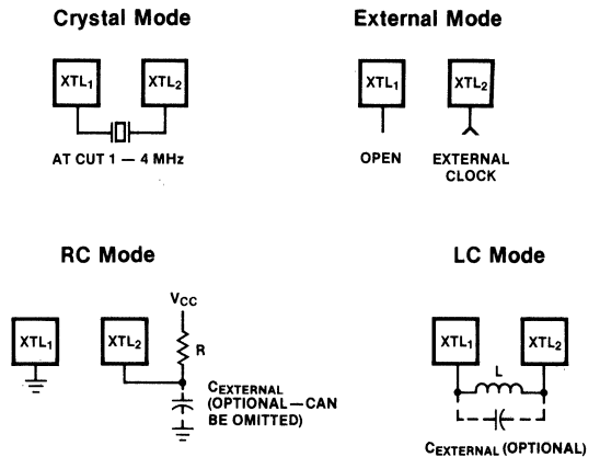
Fig. 5 Clock Configurations
