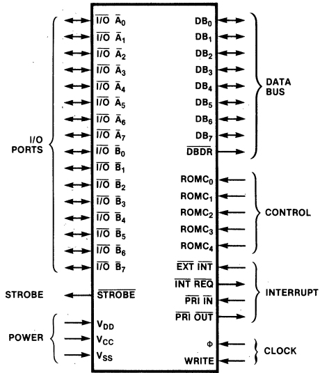
Figure 1 F3871 Block Diagram
