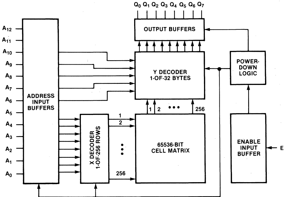
Figure 1 F3565 Block Diagram
