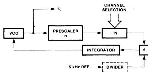
Fig. 8 High-Frequency Loop Using Fixed Prescaler
