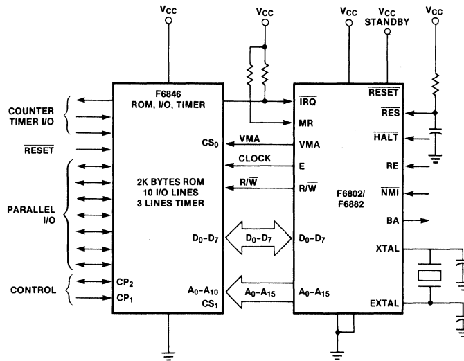
Fig. 1 Typical Microcomputer Block Diagram
