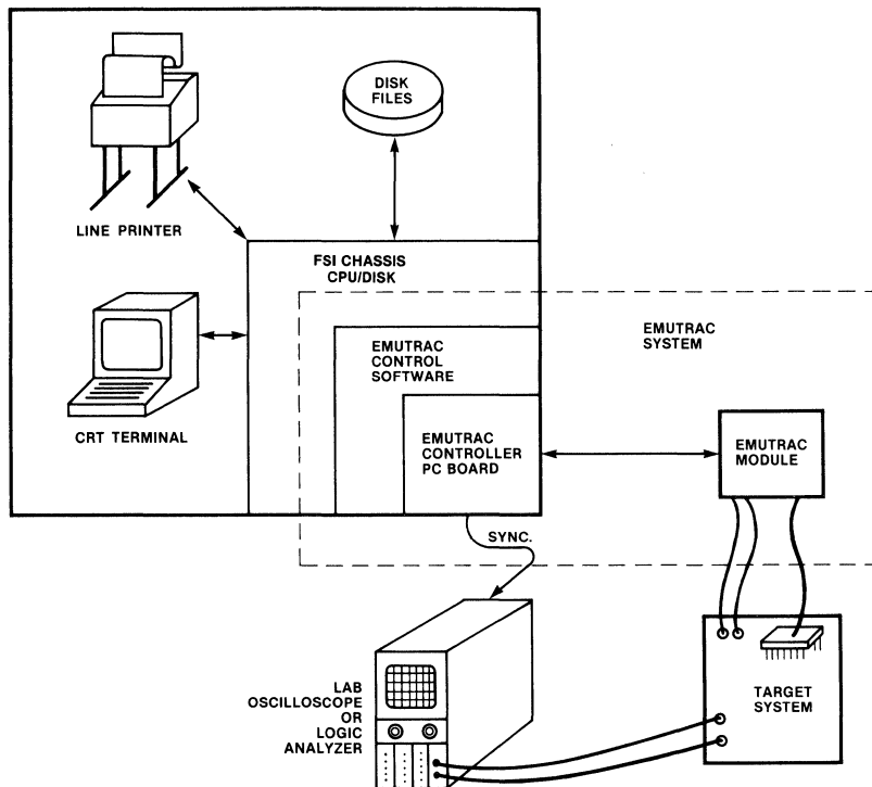
Figure 1 EMUTRAC System
