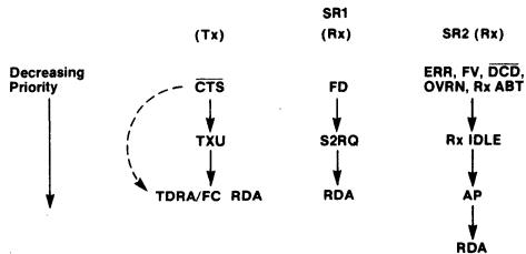
Fig. 3 Status Register Priority Tree (PSE = 1)
