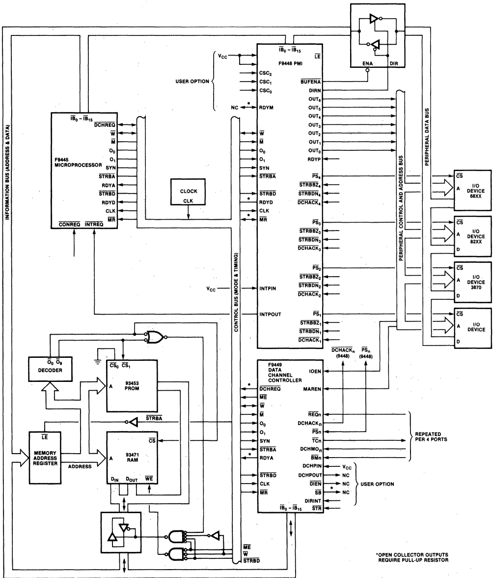
Fig. 4 F9449/F9448 Configuration
