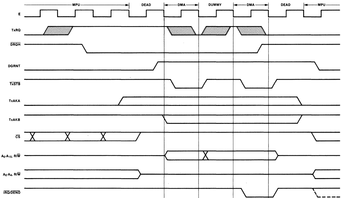
Fig. 4 Halt Burst Mode Timing
