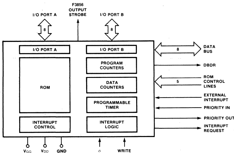
Figure 1 PSU Simplified Block Diagram
