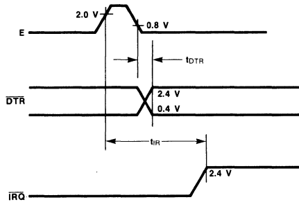
Fig. 5 Data Terminal Ready and Interrupt Request Release Times
