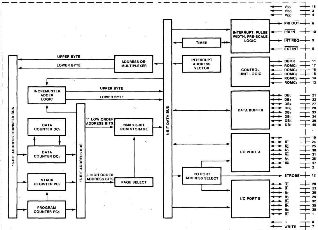
Figure 2 F38T56 Block Diagram
