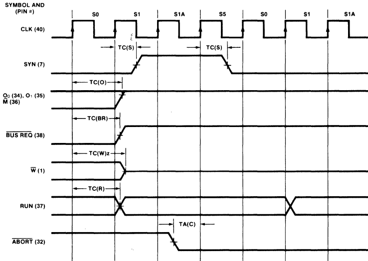
Fig. 13 Minimum Memory Cycle Timing*
