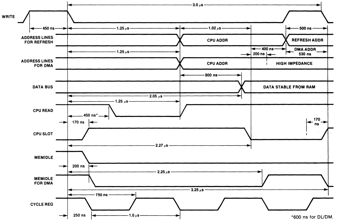
Fig. 5 Memory Refresh and DMA Timing During Long-Cycle Memory Read, with Address Out of Data Counter
