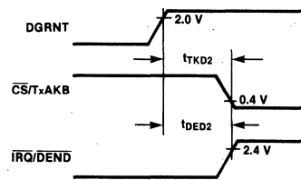
Fig. 15 TxAKB, IRQ/DEND Output Timing from DGRNT Input
