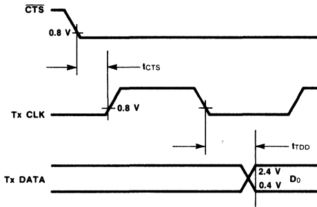
Fig. 6 Clear-to-Send Set-up Time
