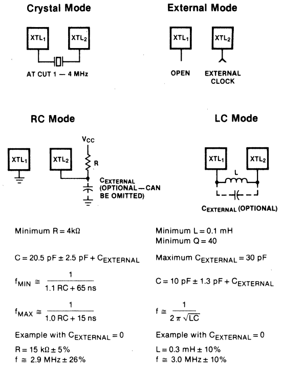
Fig. 7 F3872 Clock Configurations
