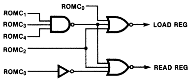
Fig. 3 DMAC ROMC State Response
