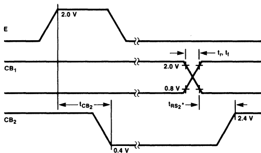
Fig. 15 CB_2 Delay Time (Write Mode; CRB-5 = 1 ; CRB-3 = CRB-4 = 0 )
