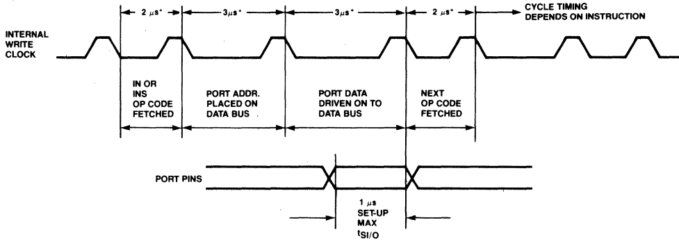
Fig. 10 Port Input/Output Timing Diagrams
