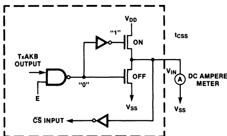
Fig. 17 \overline{CS}/TxAKB Source Current Test Circuit
