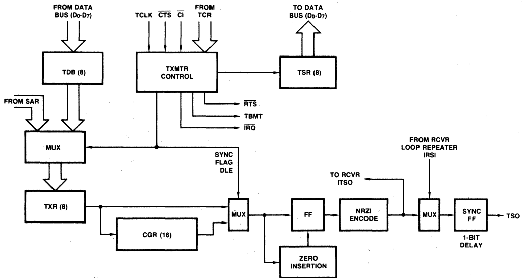
Fig. 3 Transmitter Data Path
