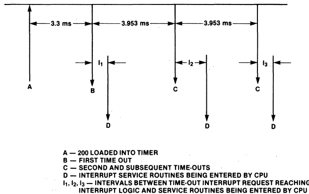
Figure 10 Time-Out and Interrupt Request Timing
