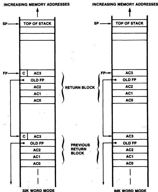
Fig. 3 Data Organization in a Stack (LIFO)
