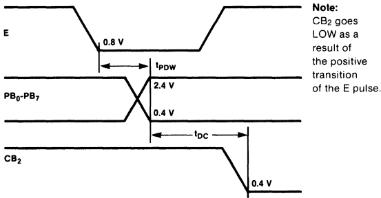
Fig. 13 Peripheral Data and CB_2 Delay Times (Write Mode; CRB-5 = CRB-3 = 1 ; CRB-4 = 0 )
