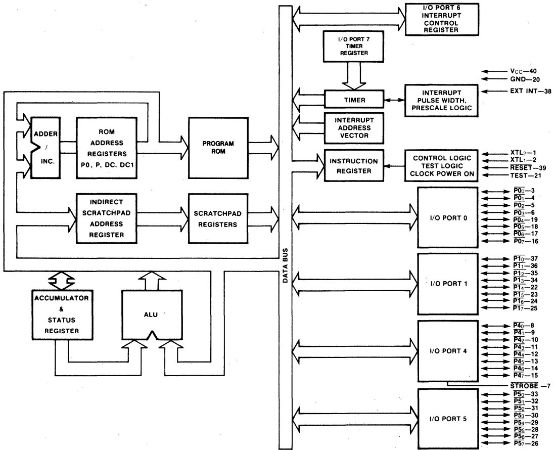
Fig. 2 F3870 Block Diagram
