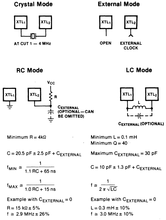
Fig. 6 F3870 Clock Configurations
