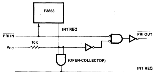
Fig. 8 PRI OUT Signal Generation
