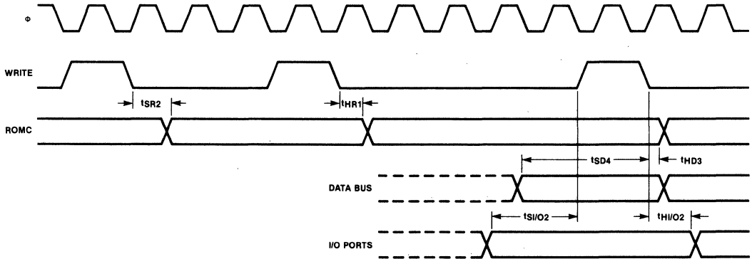
Figure 8 F3871 Input Timing
