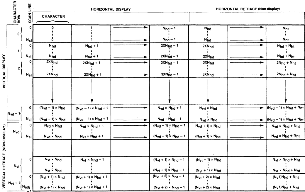
Figure 15 Refresh Memory Addressing (MA 0 – MA 13 ) Timing Diagram
