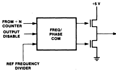
Fig. 18 Frequency/Phase Comparator Output
