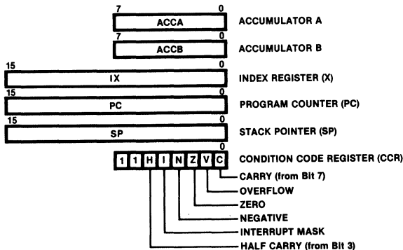
Figure 5-2 F6800/F6802/F6808/F6882 Programming Model
