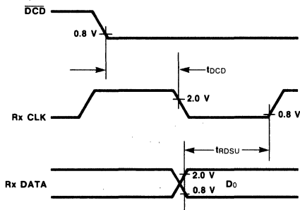
Fig. 7 Data Carrier Detect Set-up Time
