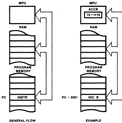
Fig. 21 Accumulator Addressing
