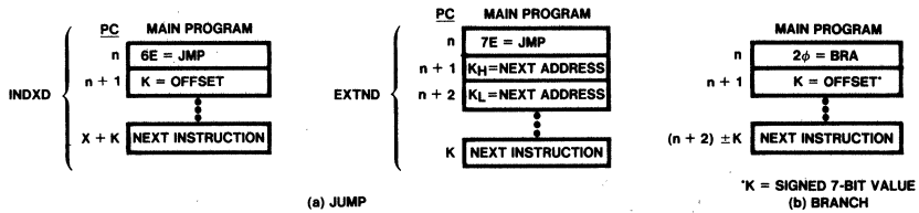
Fig. 10 Program Flow for Jump and Branch Instructions
