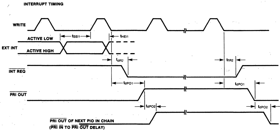
Figure 10 F3871 Interrupt Timing
