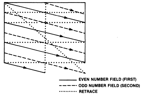
Figure 2 Interlace Raster Scan System
