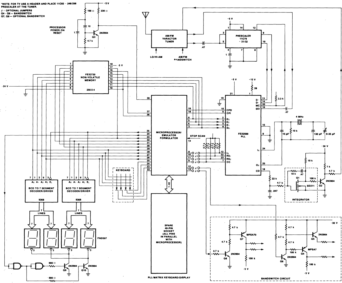
Fig. 20 Advanced AM/FM Radio Application
