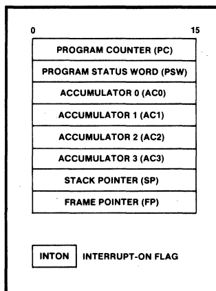
Fig. 2 F9445 Register Model
