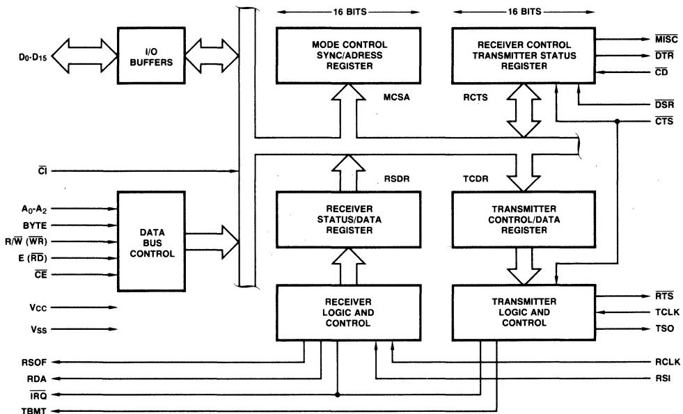
Fig. 1 Block Diagram
