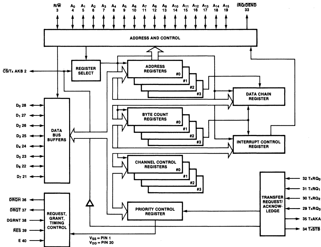
Fig. 1 Block Diagram
