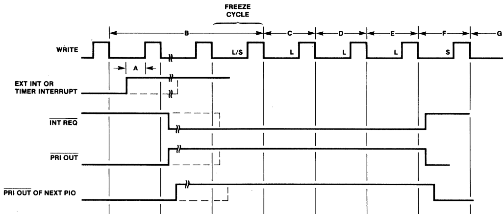
Figure 5 F3871 Interrupt Sequence
