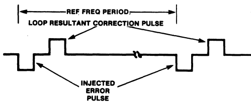
Fig. 15 Output of Frequency/Phase Detector with Anti-Backlash Circuit
