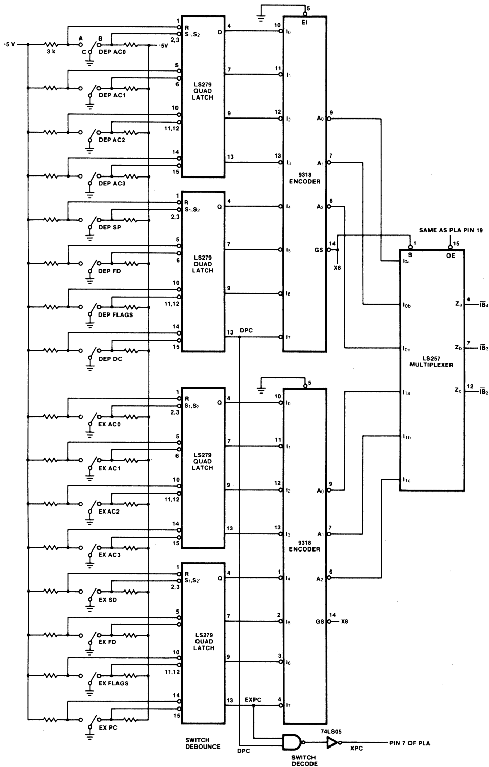
Fig. 10 F9445 Console Connection Scheme (1 of 3)
