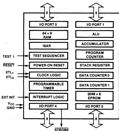
Fig. 1 F3870 Architecture
