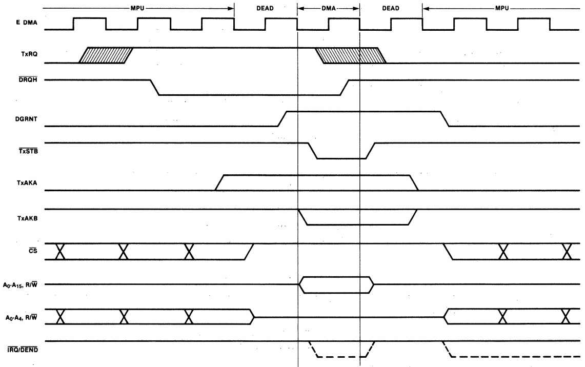
Fig. 3 Halt Steal Mode Timing
