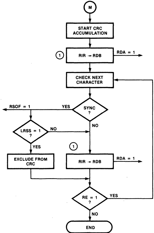
Fig. 8b BCP Receive
