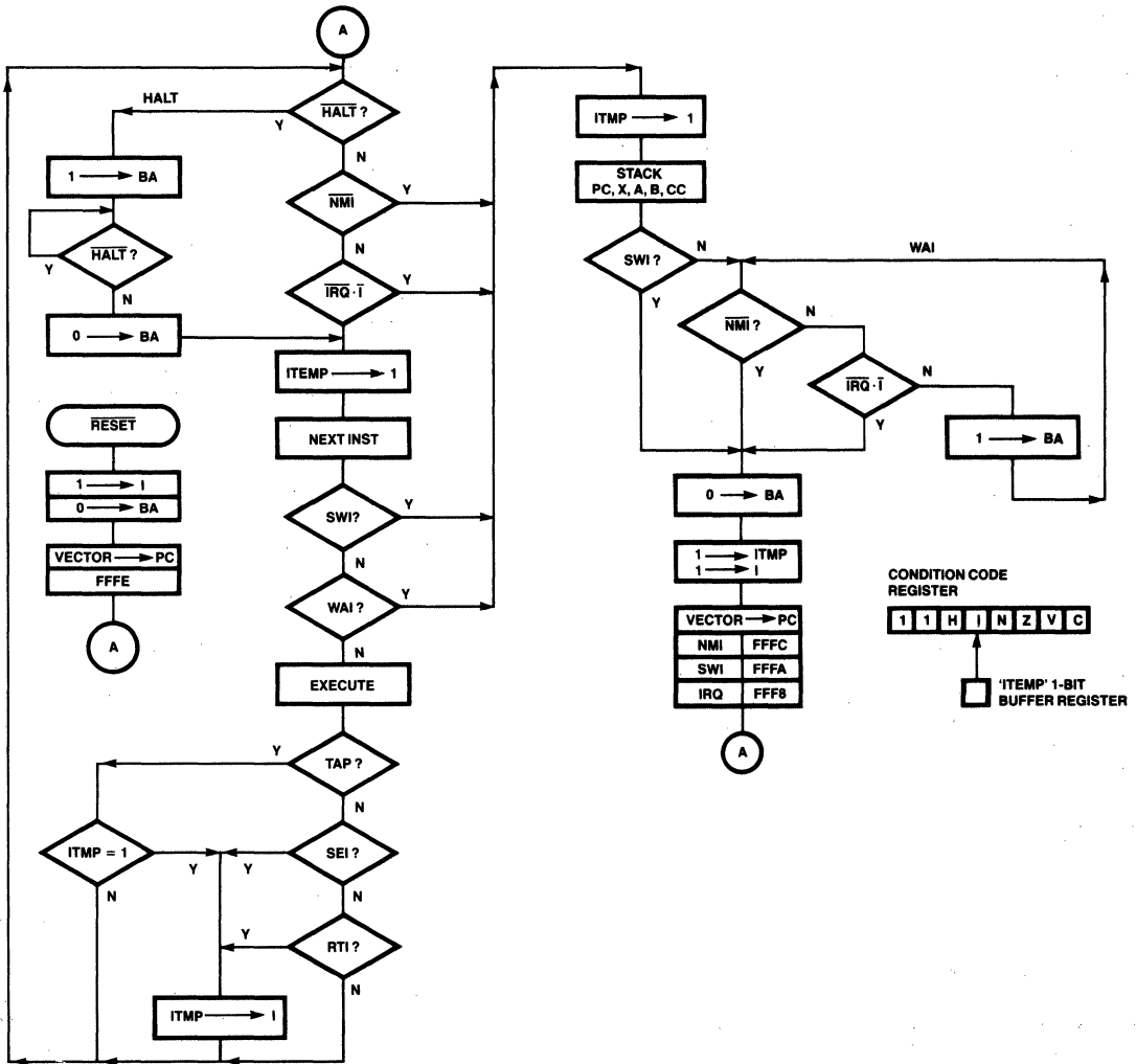
Fig. 1 MPU Flow Chart
