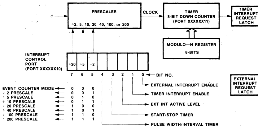
Fig. 3 Timer and Interrupt Control Port Block Diagram
