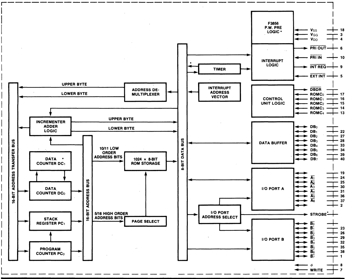
Figure 2 PSU Functional Diagram
