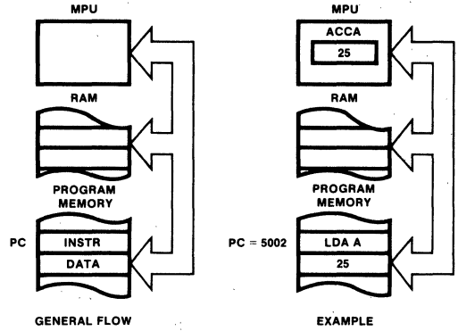
Fig. 22 Immediate Addressing Mode
