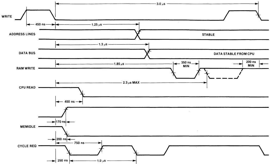
Fig. 17 DMI Timing Signals Output During a Write-to-Memory
