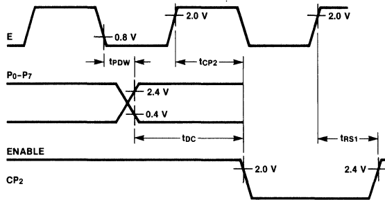
Fig. 4 Peripheral Data and CP2 Delay (Control Mode PCR5 = H, PCR4 = L, PCR3 = H)
