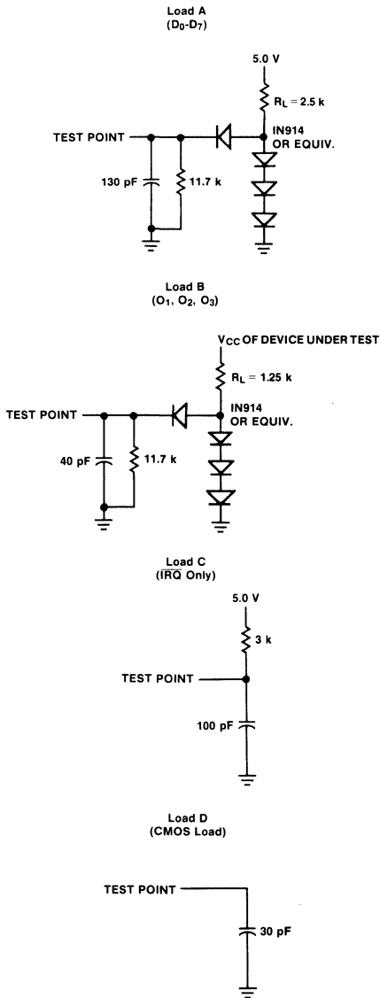
Fig. 9 Bus Timing Test Loads
