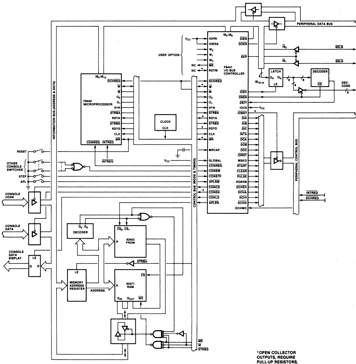
Figure 2 System Configuration
