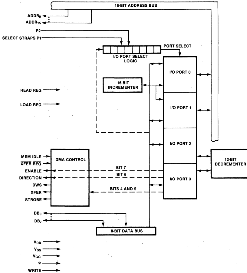
Fig. 1 F3854 Logic Organization
