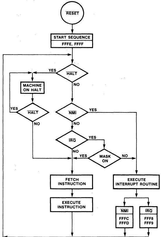
Fig. 7 MPU Flow Chart
