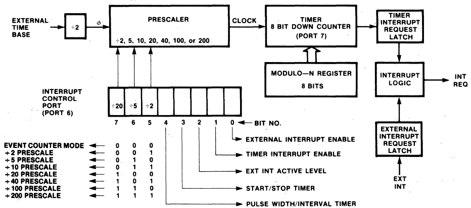
Fig. 4 Timer and Interrupt Control Port Block Diagram
