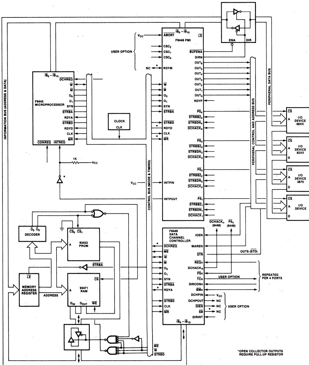
Figure 1 System Configuration
