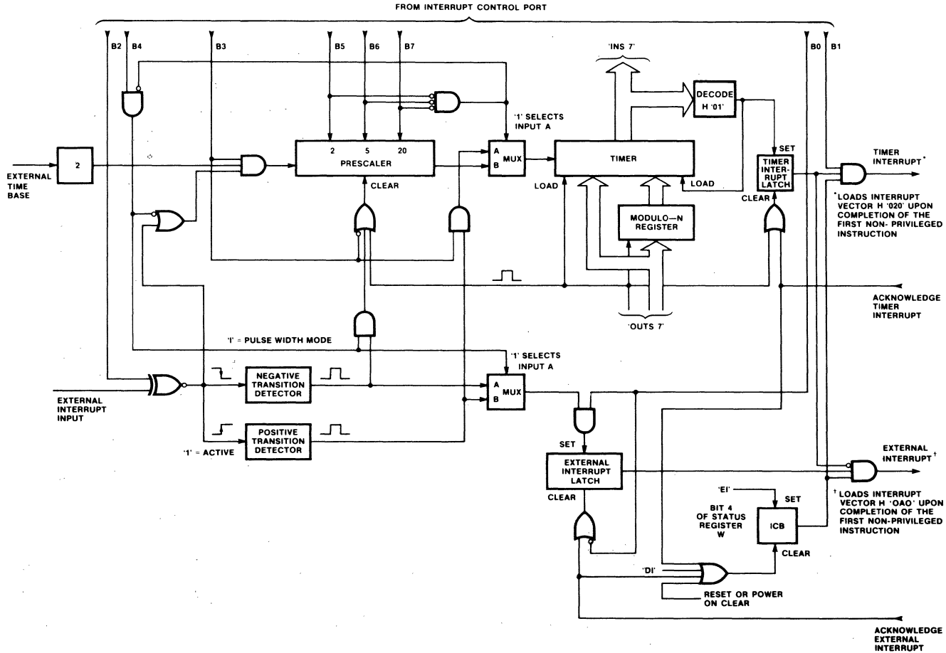
Fig. 5 Timer/Interrupt Functional Diagram
