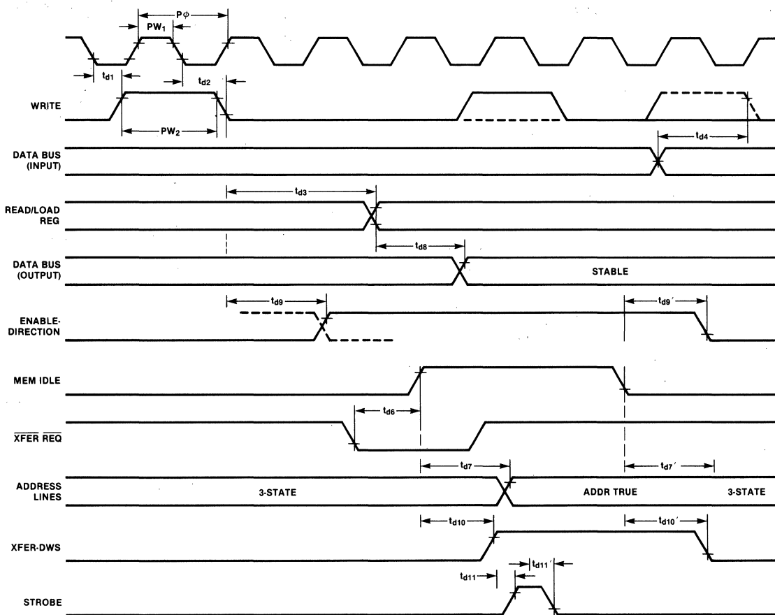
Fig. 6 F3854 DMAC Timing Characteristics
