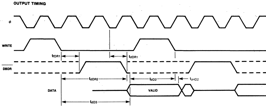
Figure 9 F3871 Output Timing
