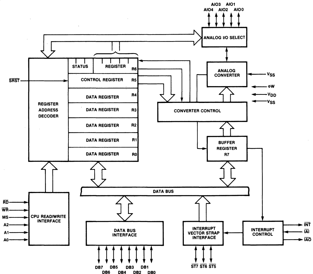
Figure 1 38752 Block Diagram
