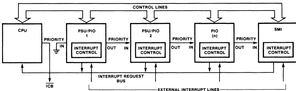
Fig. 4 F8 Interrupt Interconnection
