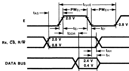
Fig. 8 Bus Read Timing Characteristics (Read information from SSDA)
