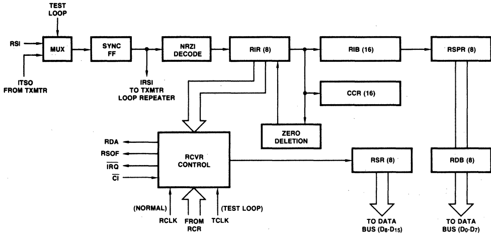
Fig. 2 Receiver Data Path
