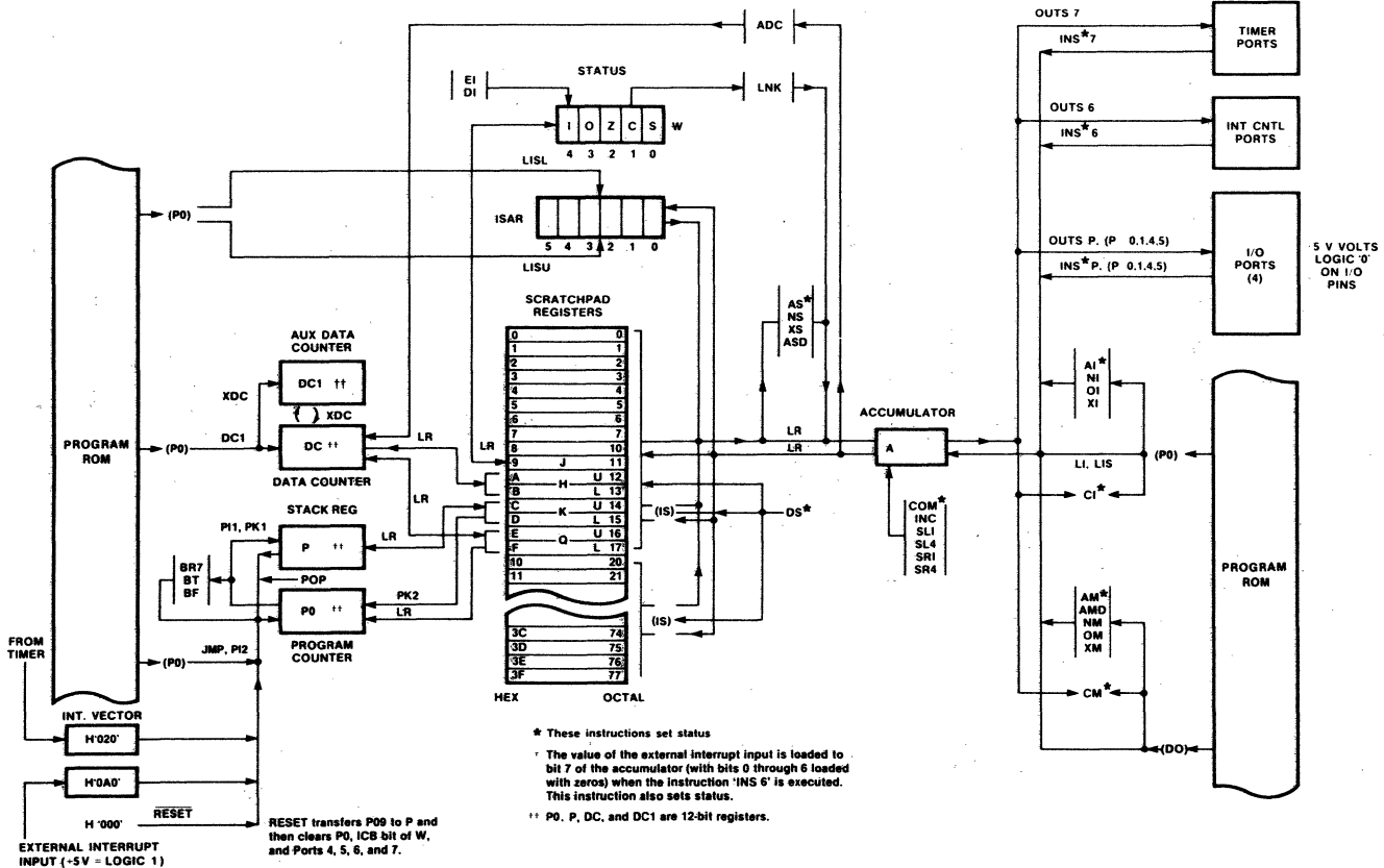
Fig. 8 Programming Model
