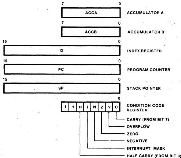
Fig. 7 Programming Model of The Microprocessing Unit
