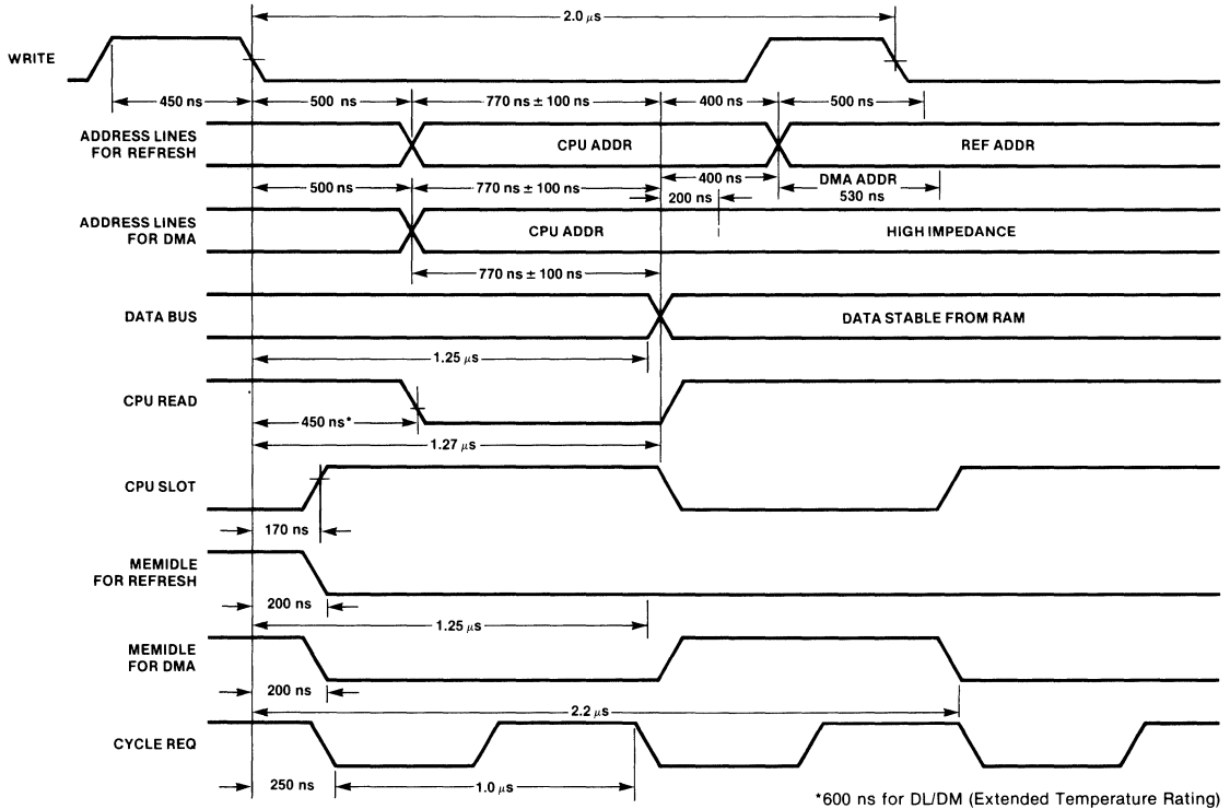
Fig. 3 Memory Refresh and DMA Timing During Short-Cycle Memory Read, with Address Out of Program Counter
