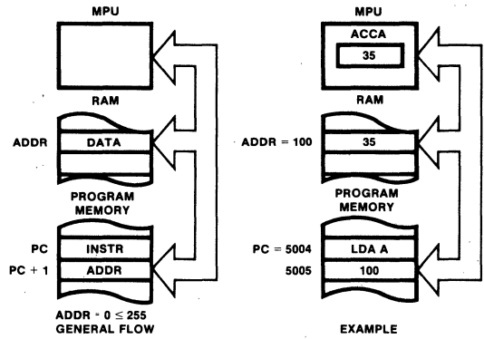
Fig. 23 Direct Addressing Mode
