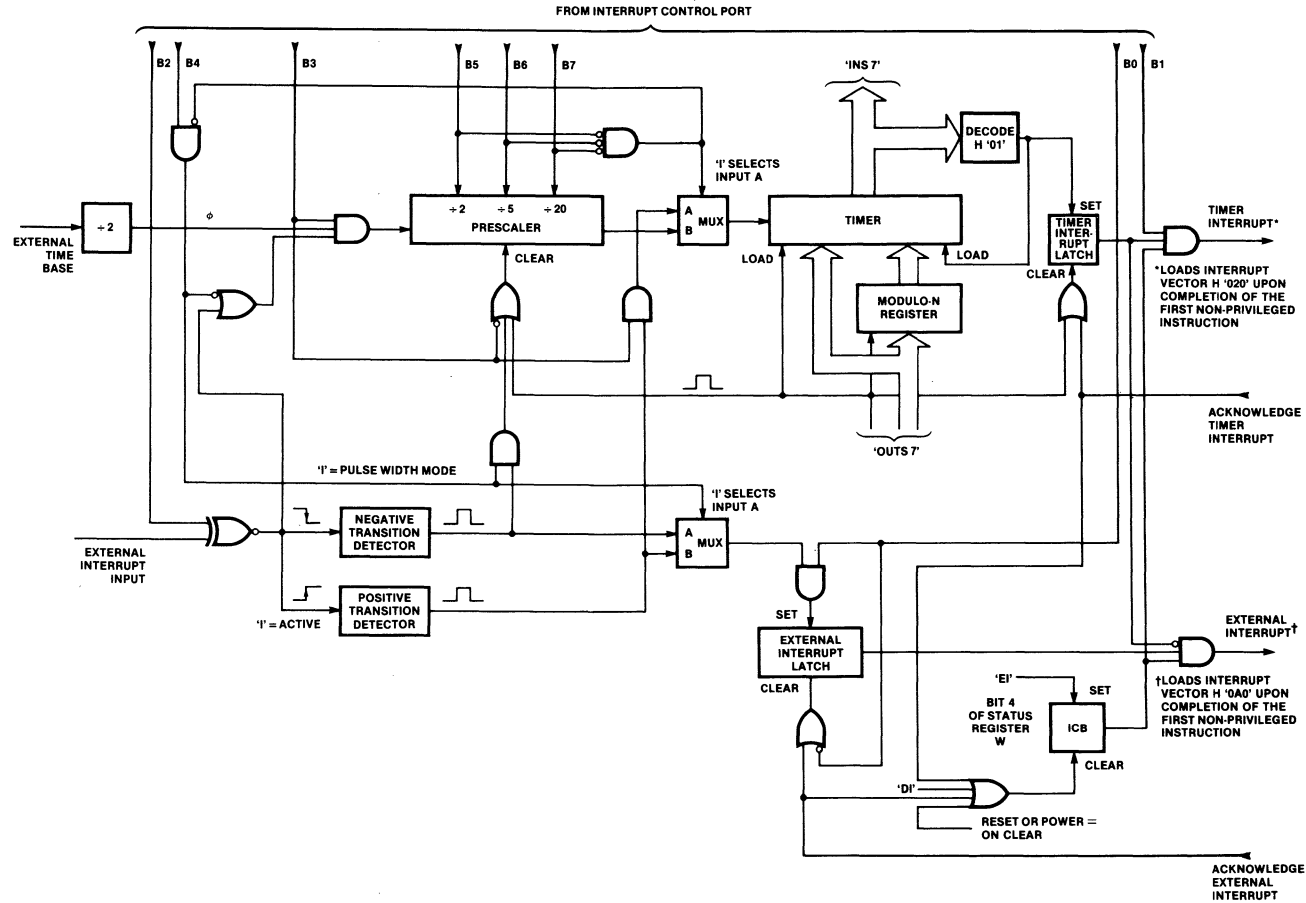
Fig. 4 Timer/Interrupt Functional Diagram
