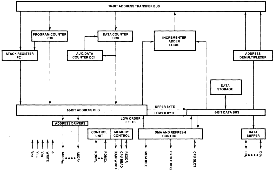
Fig. 1 F3852 DMI Logic Organization
