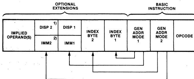
Figure 3 F16032 General Instruction Format
