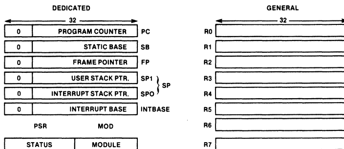
Figure 2 F16032 Dedicated and General Storage Registers
