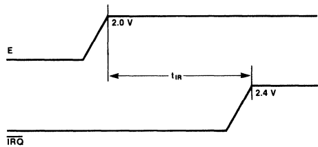
Fig. 17 \overline{IRQ} Release Time
