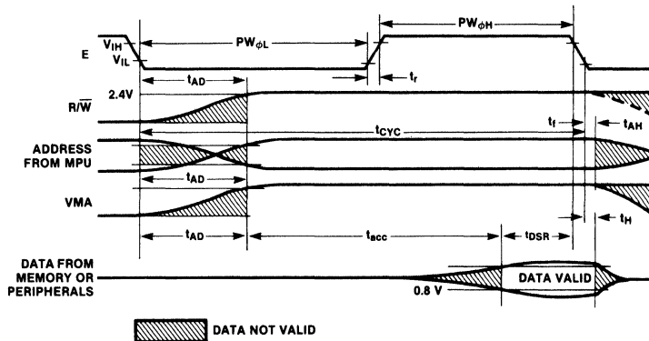
Fig. 15 Read Data from Memory or Peripherals
