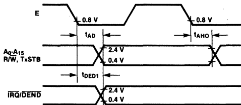
Fig. 13 Address, IRQ/DEND Output Timing
