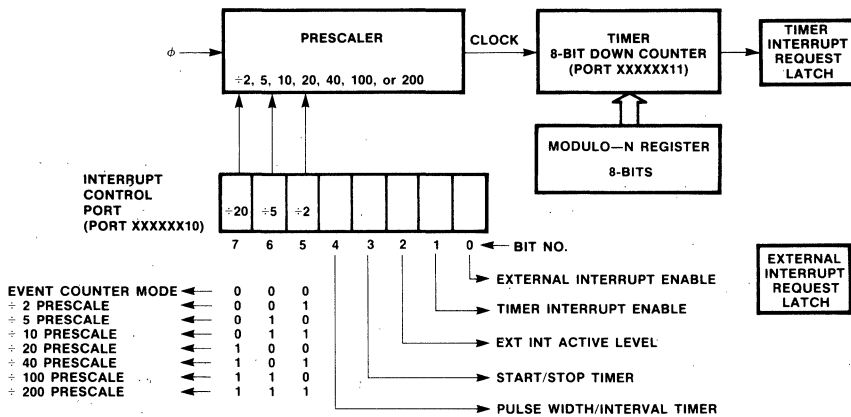
Figure 3 F3871 Timer and Interrupt Control Port Block Diagram
