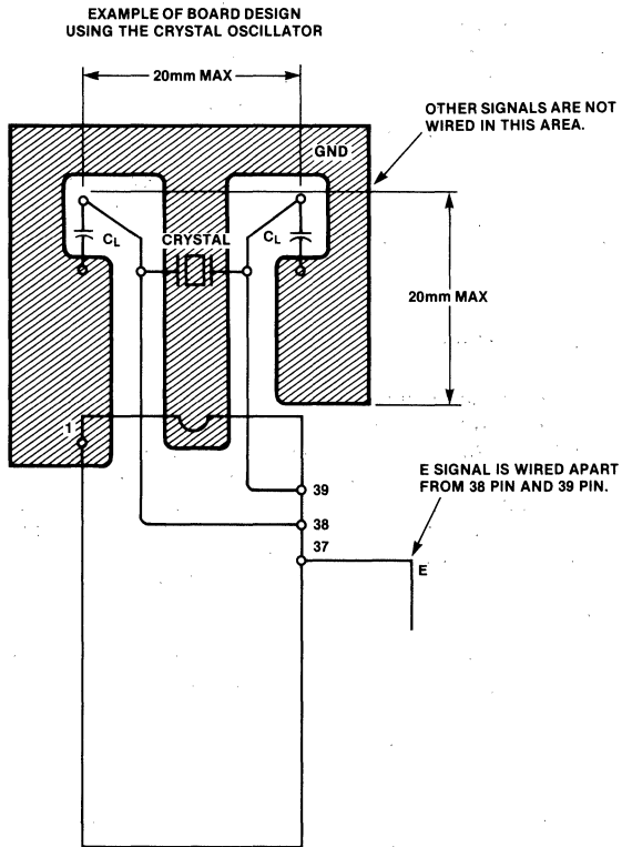
Fig. 9 Suggested PC Board Layout
