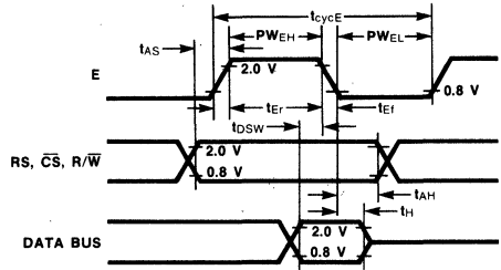
Fig. 9 Bus Write Timing Characteristics (Write information into SSDA)
