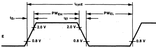
Fig. 2 Enable Signal Timing Characteristics
