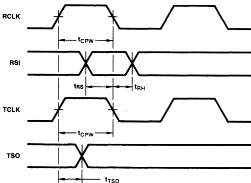
Fig. 13 Clock and Serial Data
