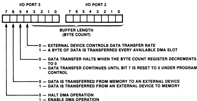
Fig. 5 I/O Port 2 and I/O Port 3 Organization
