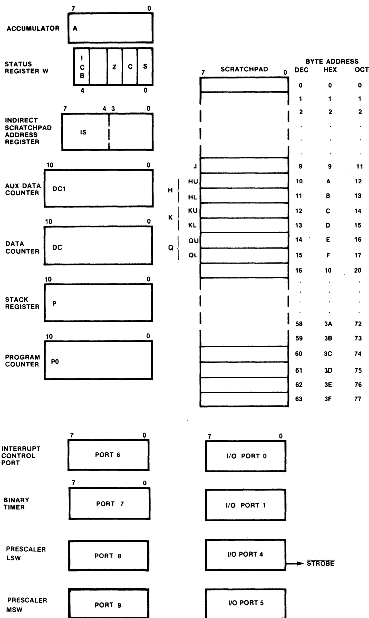
Figure 4 F38C70 Programmable Registers and Ports
