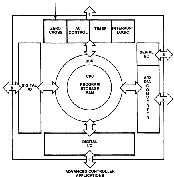
Figure 4-2 F38701 Functional Diagram
