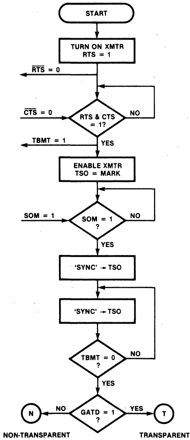
Fig. 11a BISO SYNC Transmit
