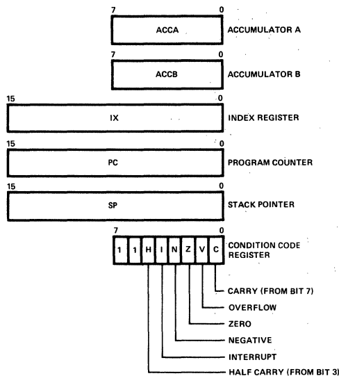
Fig. 3 Programming Model of the Microprocessing Unit
