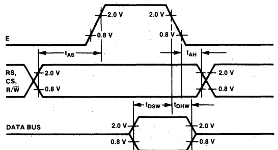
Fig. 4 Bus Timing Characteristics (Write to PIA)
