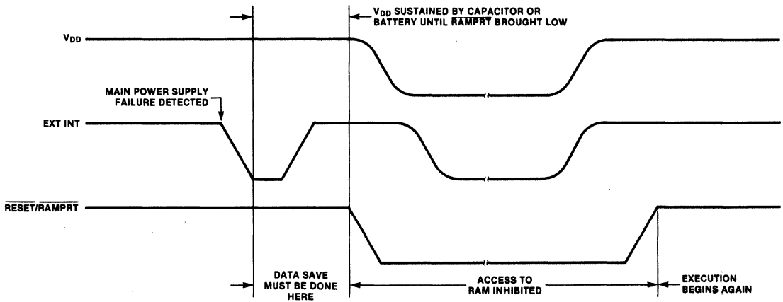
Fig. 6 Standby Power Option Modes
