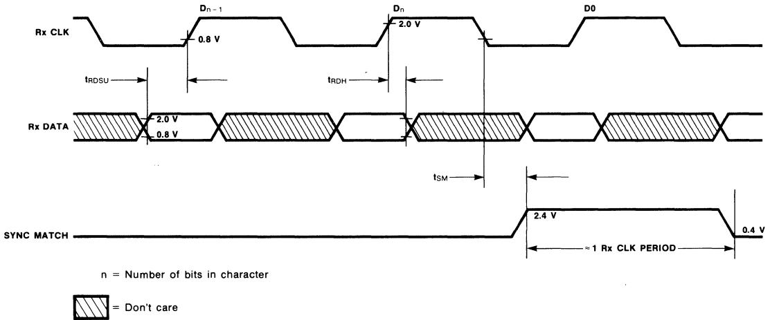
Fig. 3 Receive Data Set-up and Hold Times and Sync Match Delay Time
