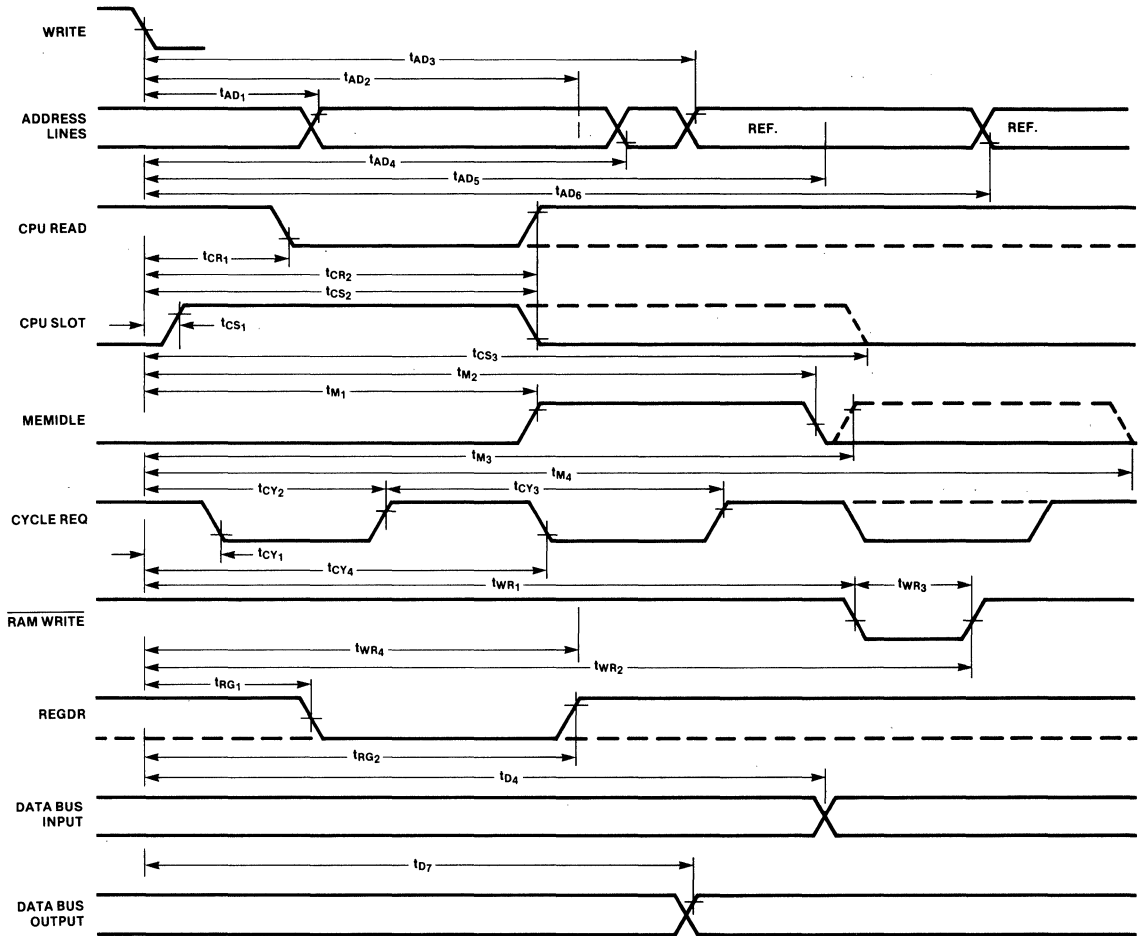
Fig. 9 F3852 DMI Timing Signals
