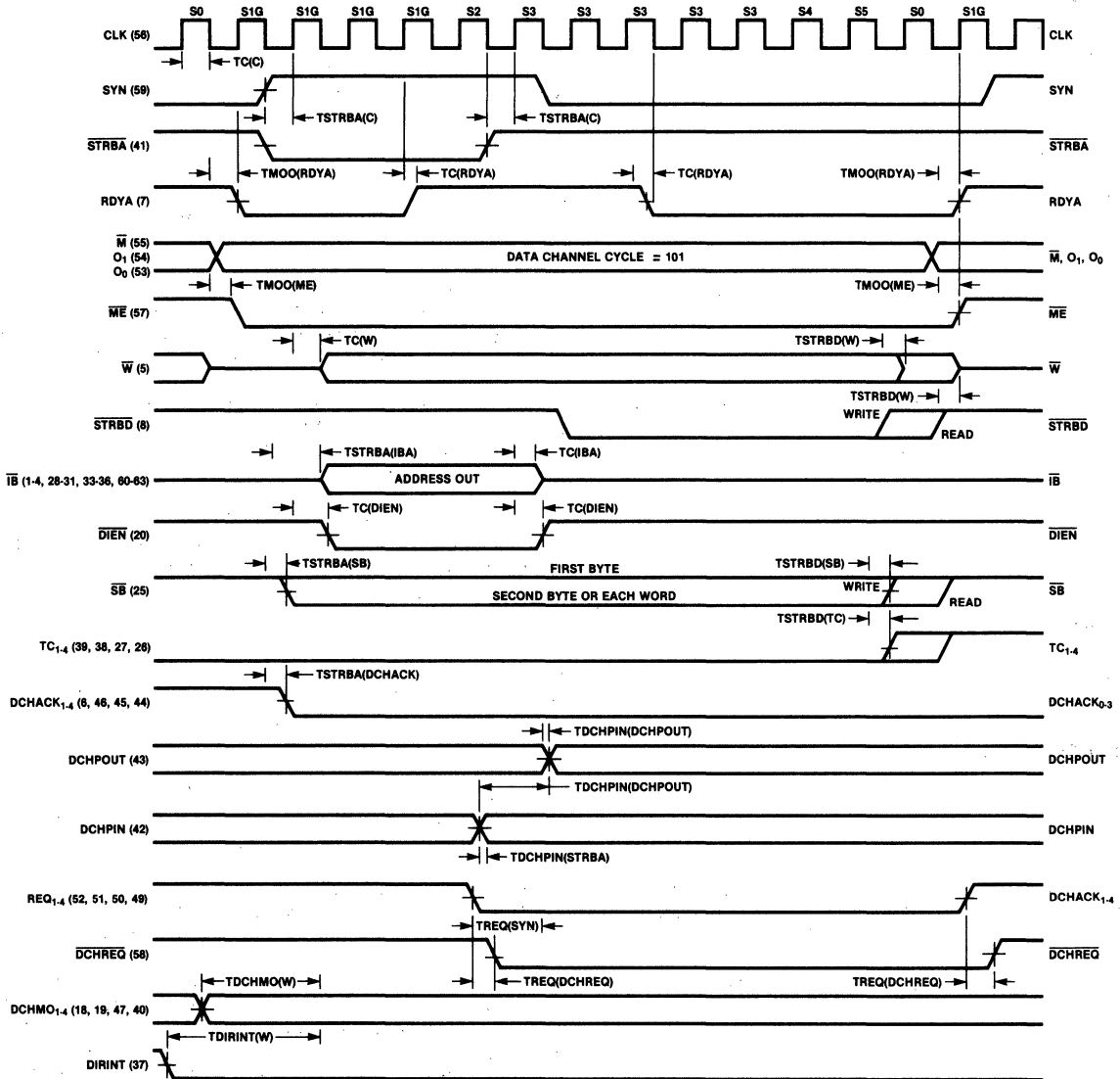
Figure 6 Data Channel Cycle Timing
