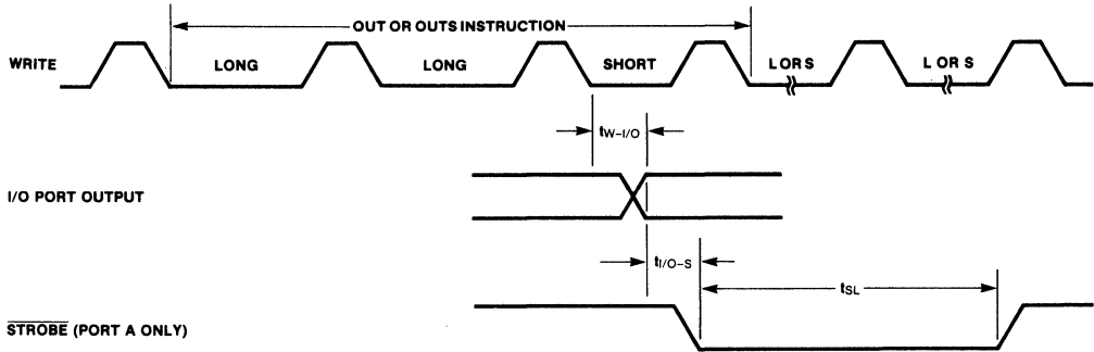
Figure 7 F3871 Strobe Timing
