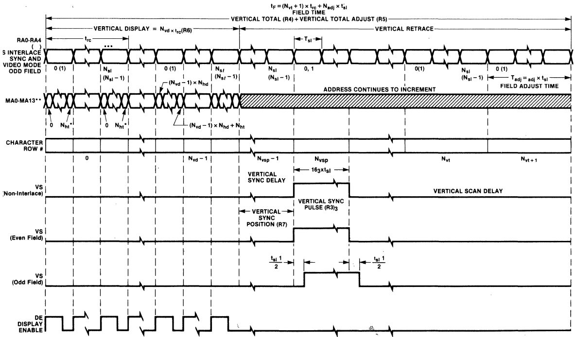
Figure 9 CRTC Vertical Timing
