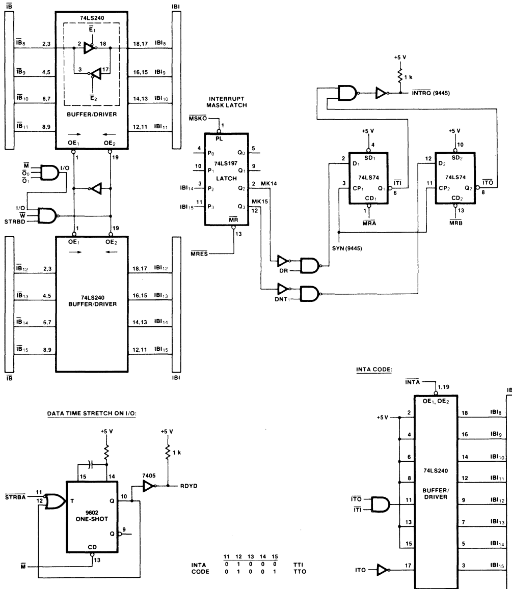
Fig. 8 F9445 Input/Output Connection Scheme (2 of 2)
