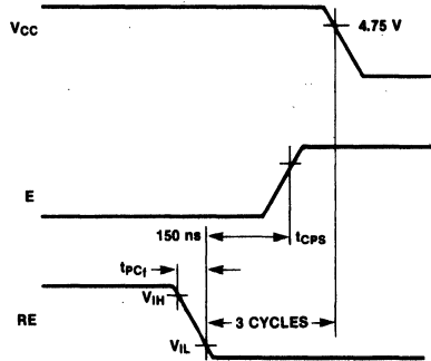
Fig. 6 Power-Down Sequence
