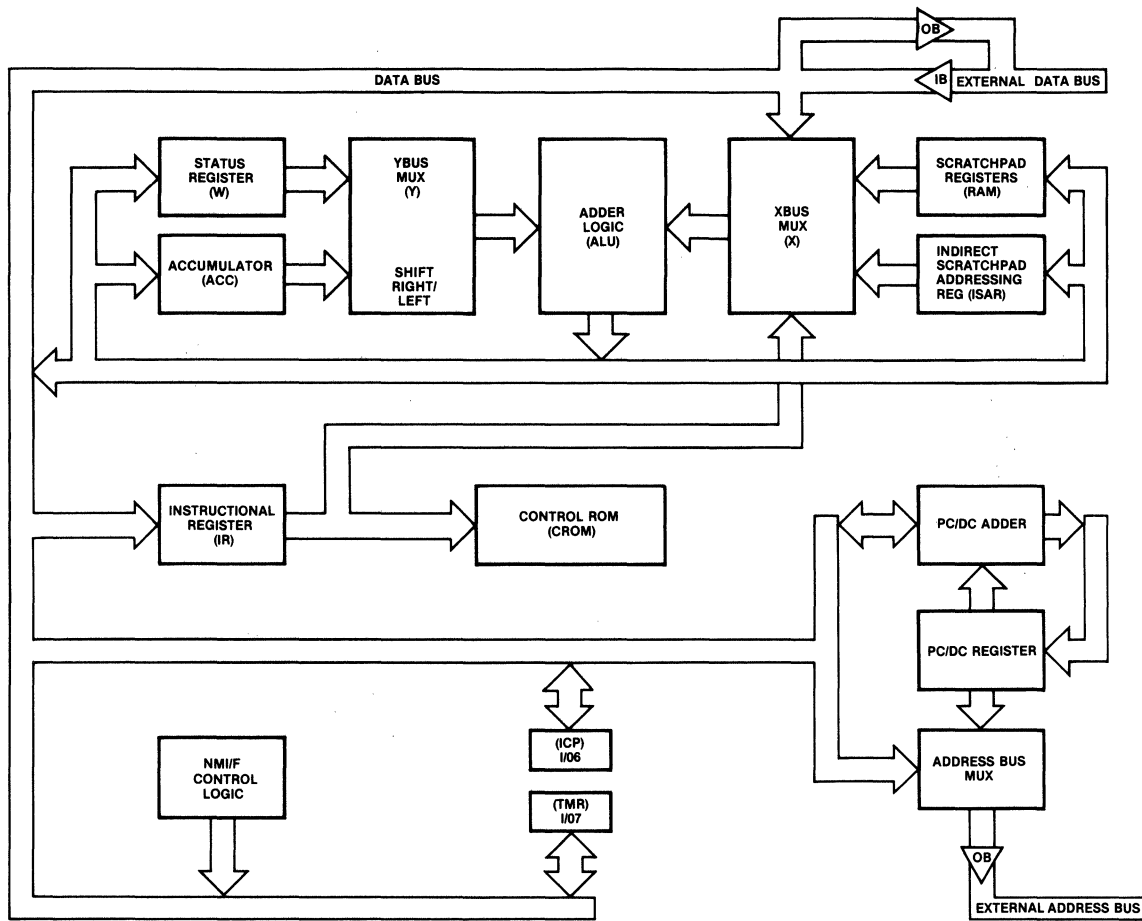
Figure 1 F38700 Block Diagram
