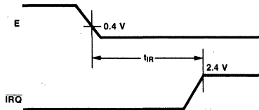
Fig. 8 \overline{IRQ} Release Time
