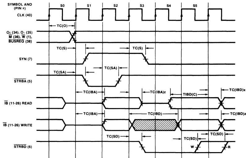
Fig. 13 Minimum Memory Cycle Timing*
