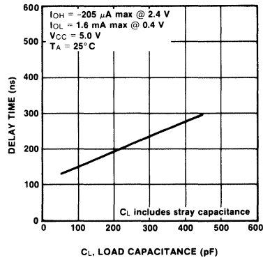
Fig. 13 Typical Data Bus Output Delay vs. Capacitive Loading
