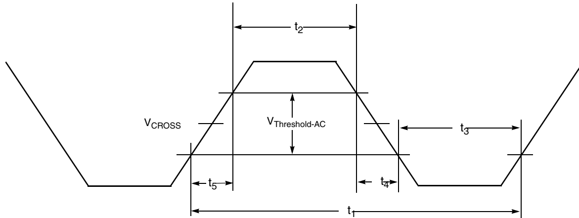
Figure 5-3. SYSCLK Waveform
