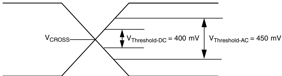
Figure 5-2. SYSCLK and SYSCLK# Differential Clock Signals
