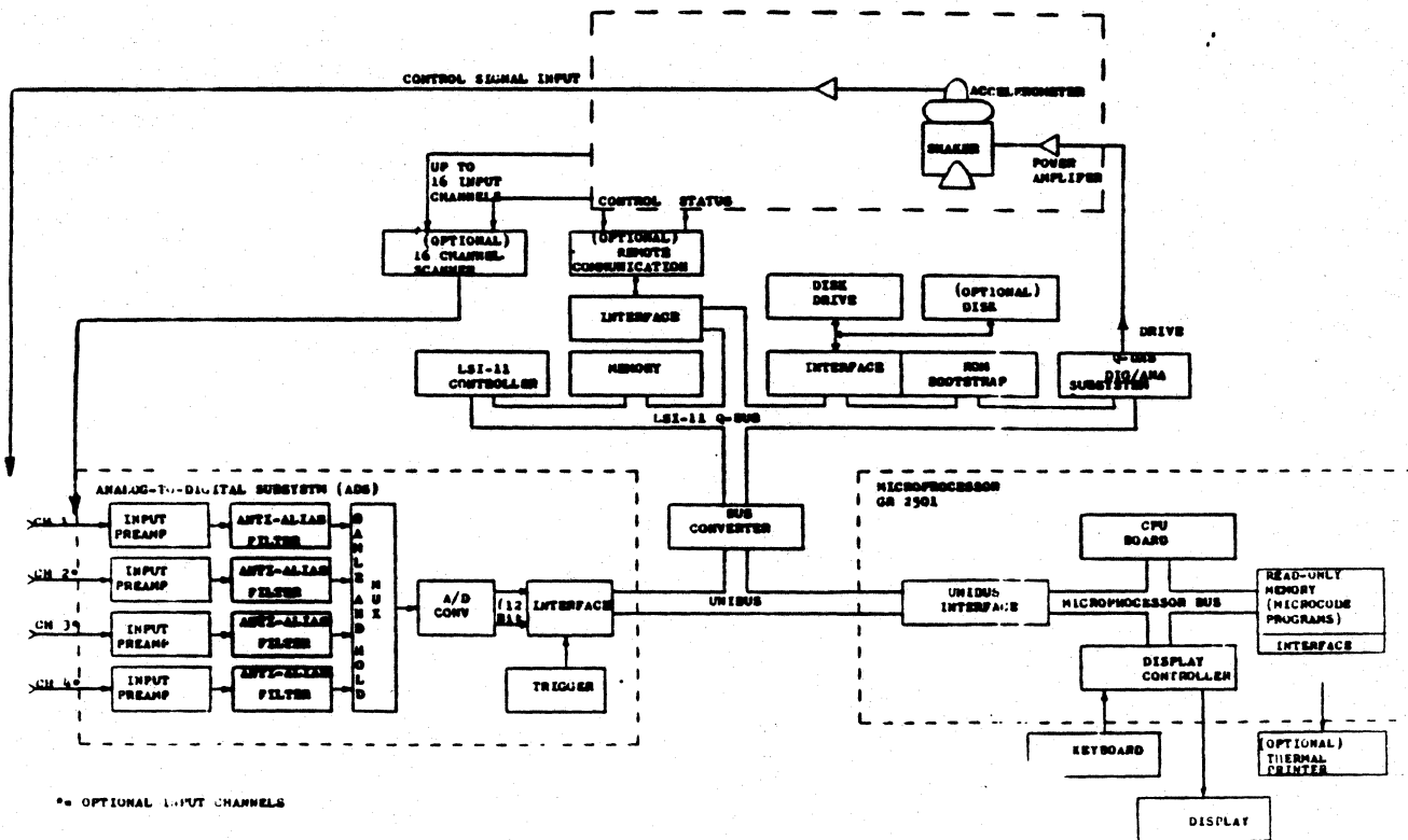
Figure 1-2. Functional Block Diagram
