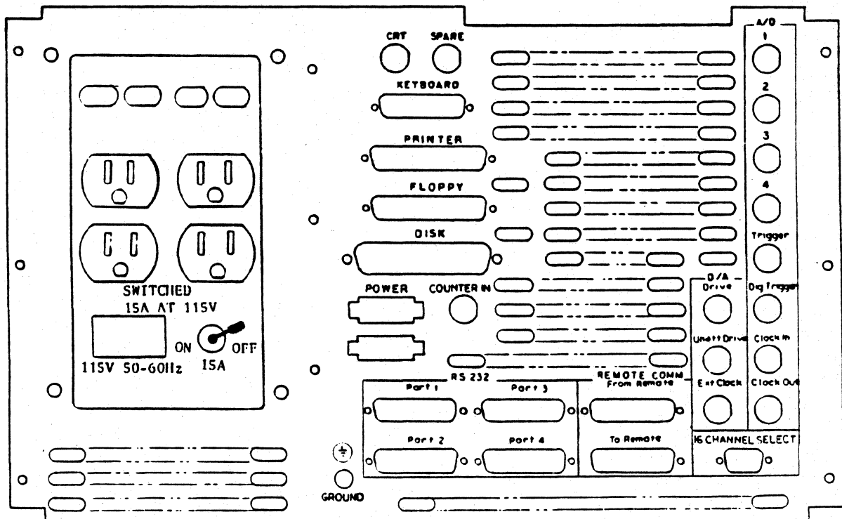
Figure 1-5. 2511/2514 System Unit
