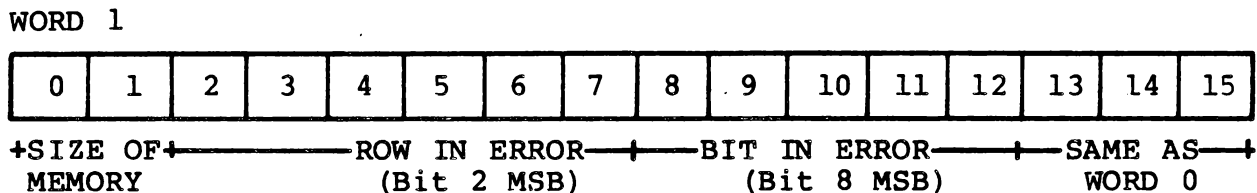
Figure 4-5. Error Log Input Bit Assignment — Word 1
