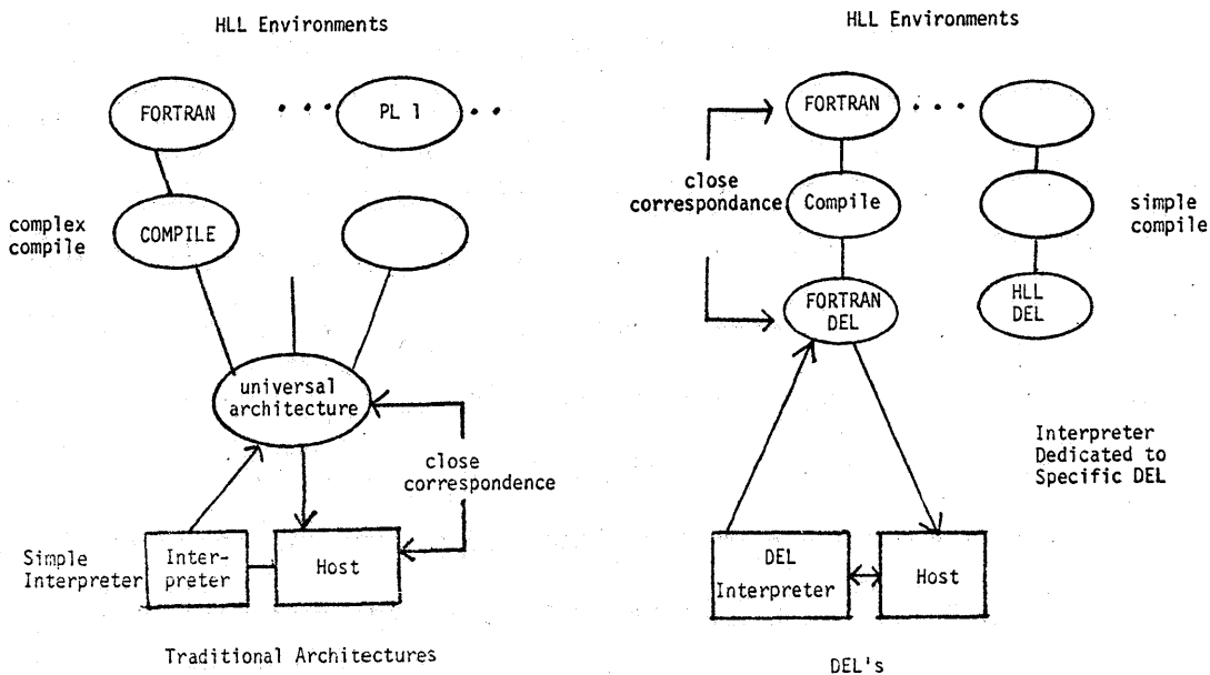
Figure 1: Directly Executed Languages
