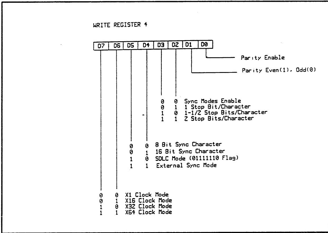
Figure 3. Write Register 4 Bit Functions
