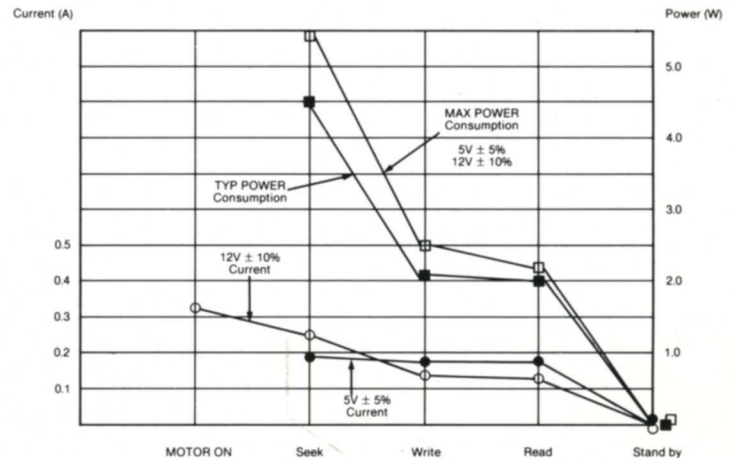
DC POWER PROFILE
