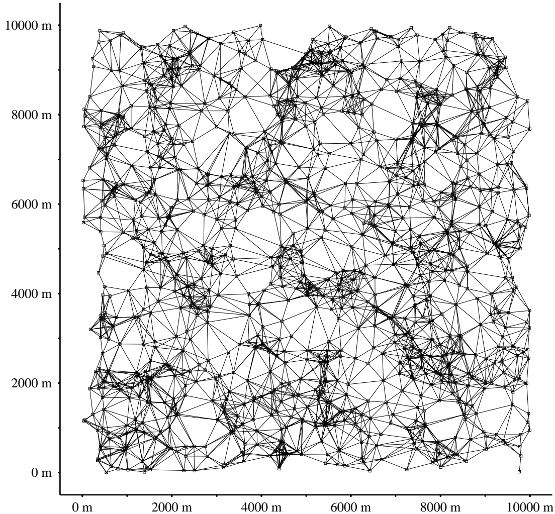
Figure 5.4: Map of the 1,000-station network showing single hops used by routes produced by a modification to minimum-energy routing. Here the cost of a route is a linear combination of the energy and the number of hops. The weightings were ad hoc and chosen to have a moderate effect on the routes.
