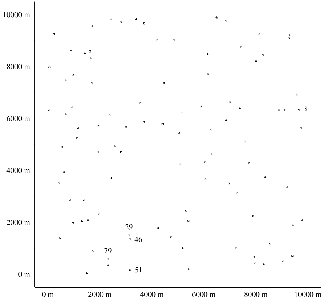
Figure 4.1: 100 stations randomly placed in a 10km by 10km square. (Four of the stations are labeled by station number as they will be referenced in the text.)
