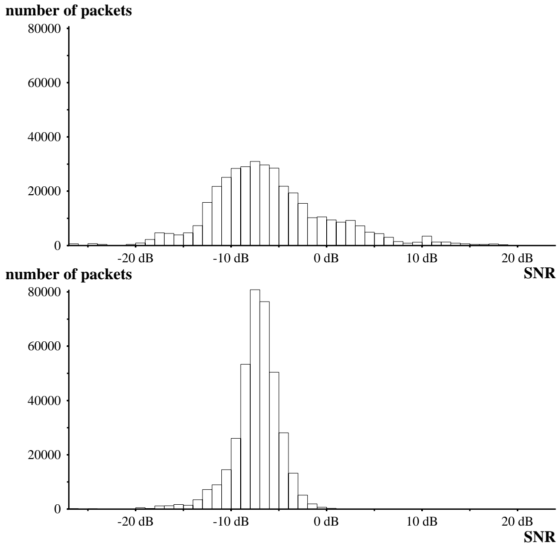
Figure 4.5: Distribution of worst signal-to-noise ratio during reception of each packet. Top plot is without power control and bottom plot is with power control.
