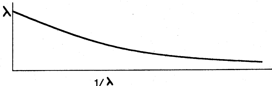
Figure 7-1: Exponential density function
