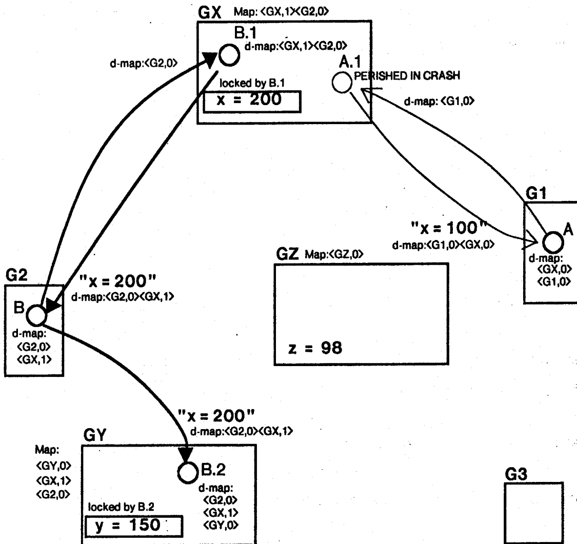
Figure 8-2: Counter-example snapshot two
