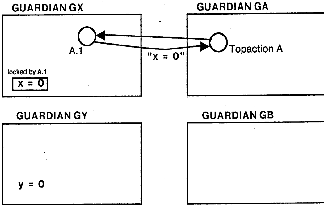
Figure 3-5: Crash-orphan example snapshot one
