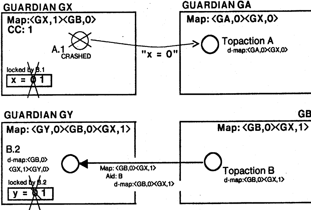
Figure 4-7: Crash-orphan detection example snapshot three
