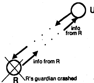
Figure 3-8: Uprooted-action created by crash of committed descendant
