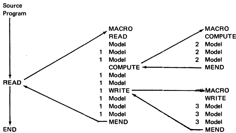
The numbers to the left of the statements indicate the value of &SYSNDX at that particular point in the program.
