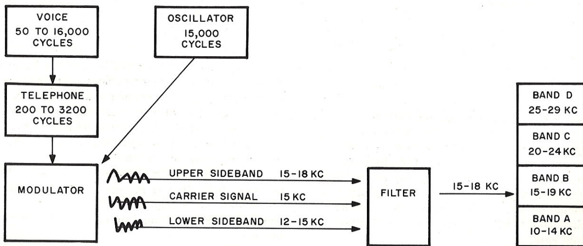
Figure 8. Modulation and filtering
