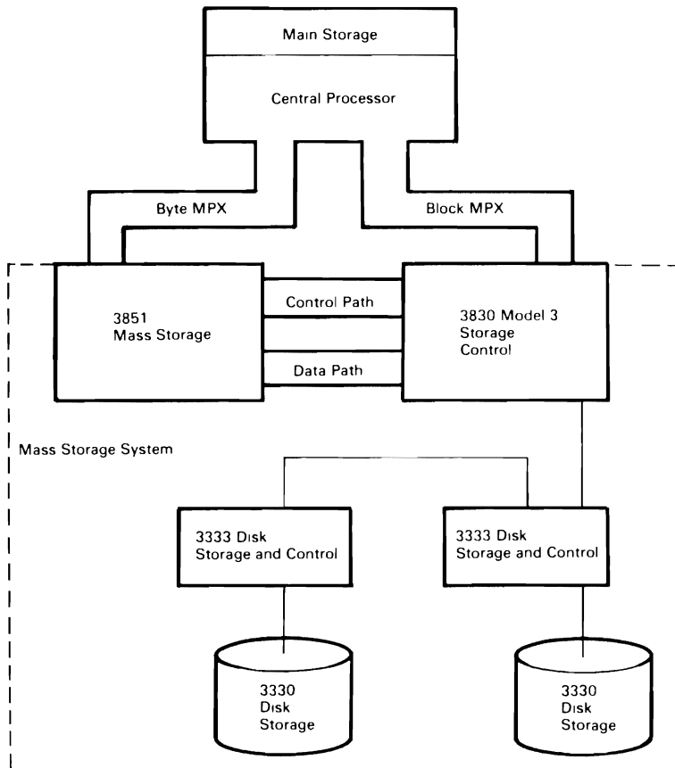
Figure 4.4 Mass Storage System Configuration
