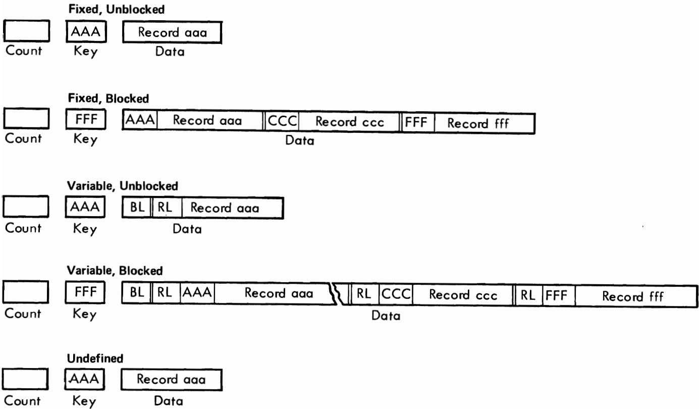
Figure 3.5 Record formats
