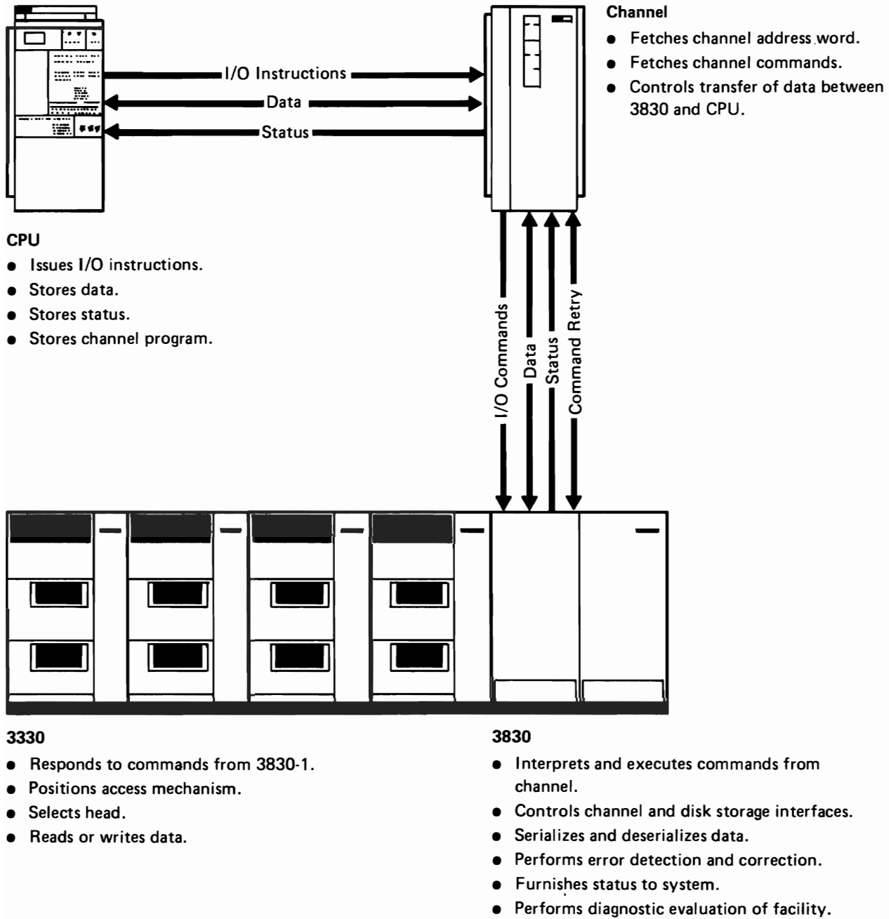
Figure 3.1 Functional Description
