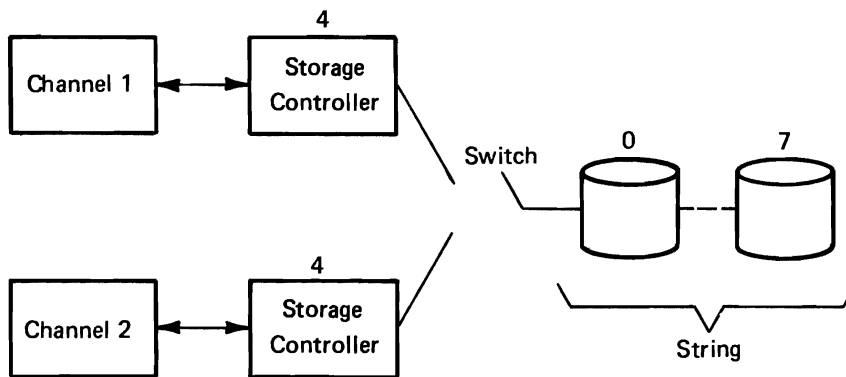
Figure 3.10 String switch
