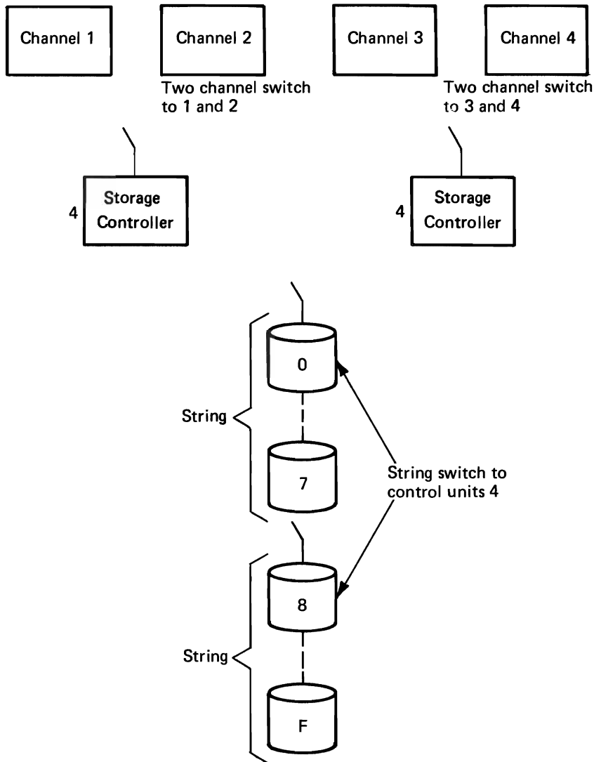
Figure 3.12 Two-channel switch plus string switch
