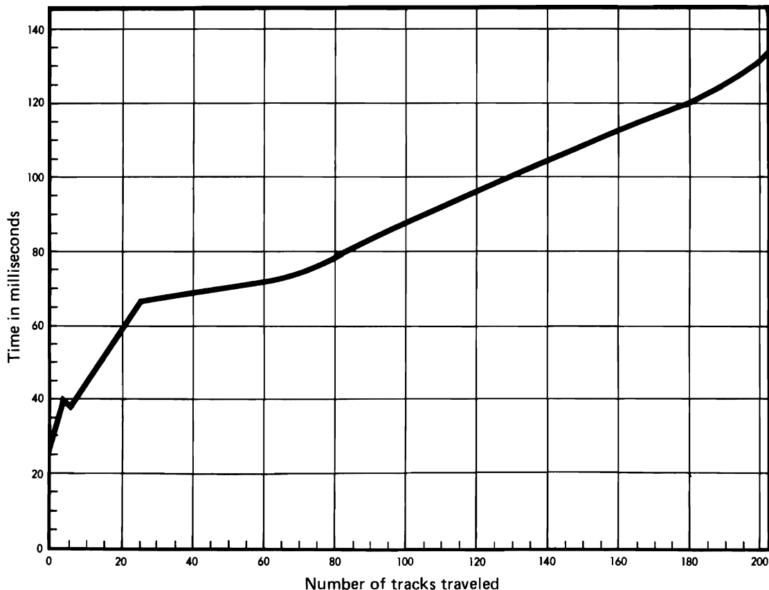
Figure 2.14 2314 access time
