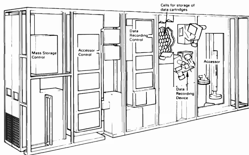
Figure 4.5 3851 Mass Storage Facility Components
