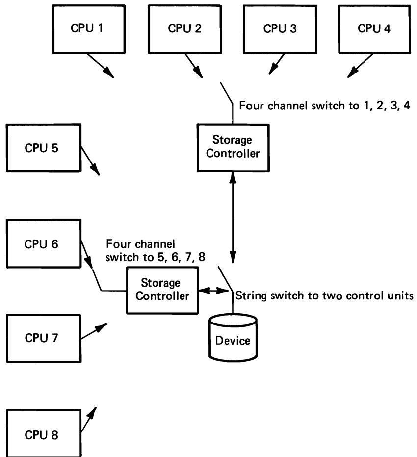
Figure 3.13 Maximum switching configuration
