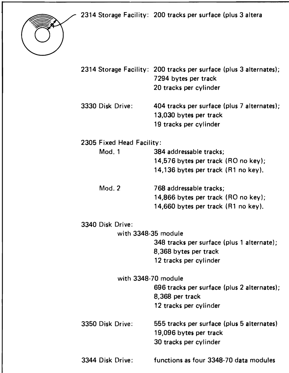
Figure 2.7 DASD tracks
