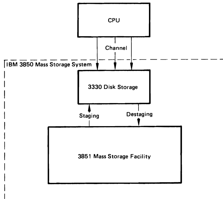
Figure 4.1 Mass Storage System Data Flow
