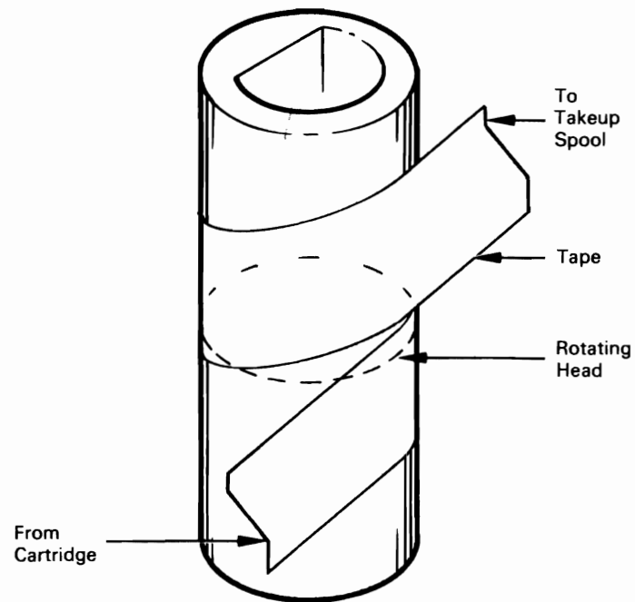
Figure 4.8 Tape Threaded in Recording Position
