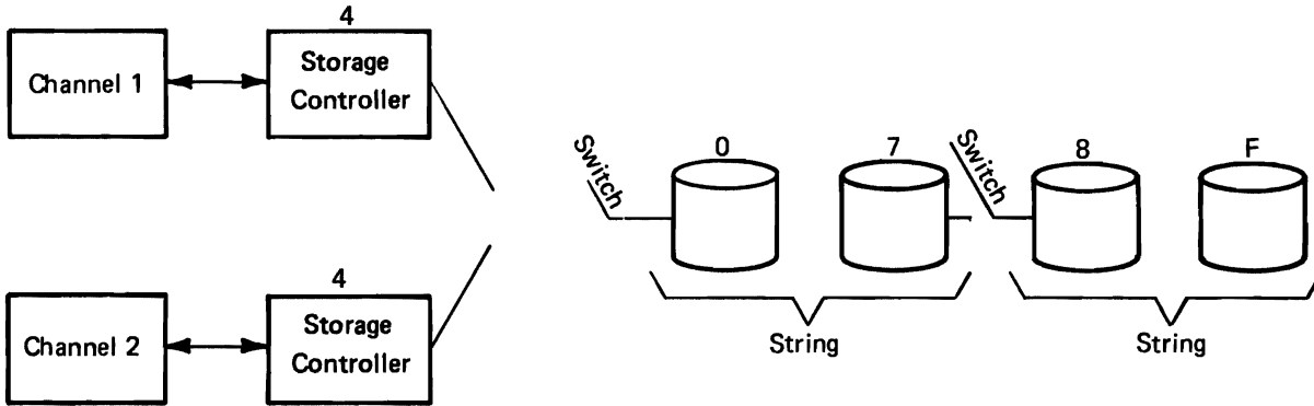
Figure 3.11 String switch-two strings
