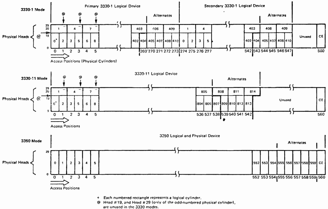
Figure 2.12 3350 mapping
