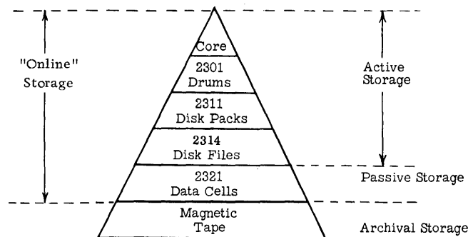
Figure 6. Storage allocation
