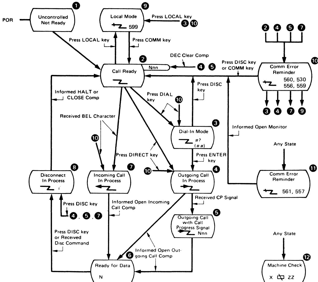
Figure C-1. Data Link Control Function
