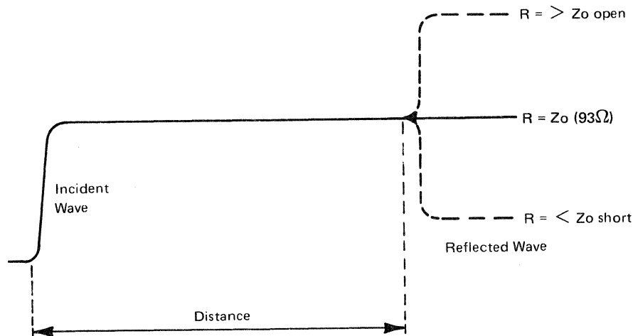
Figure 4-11. Incident and Reflected Waves
