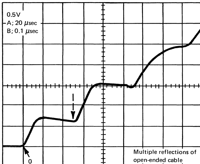
Figure 4-14 (Part 2 of 3). Display Examples
