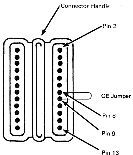
Figure 5-13. 3279 Top-Card Connector CE Jumper
