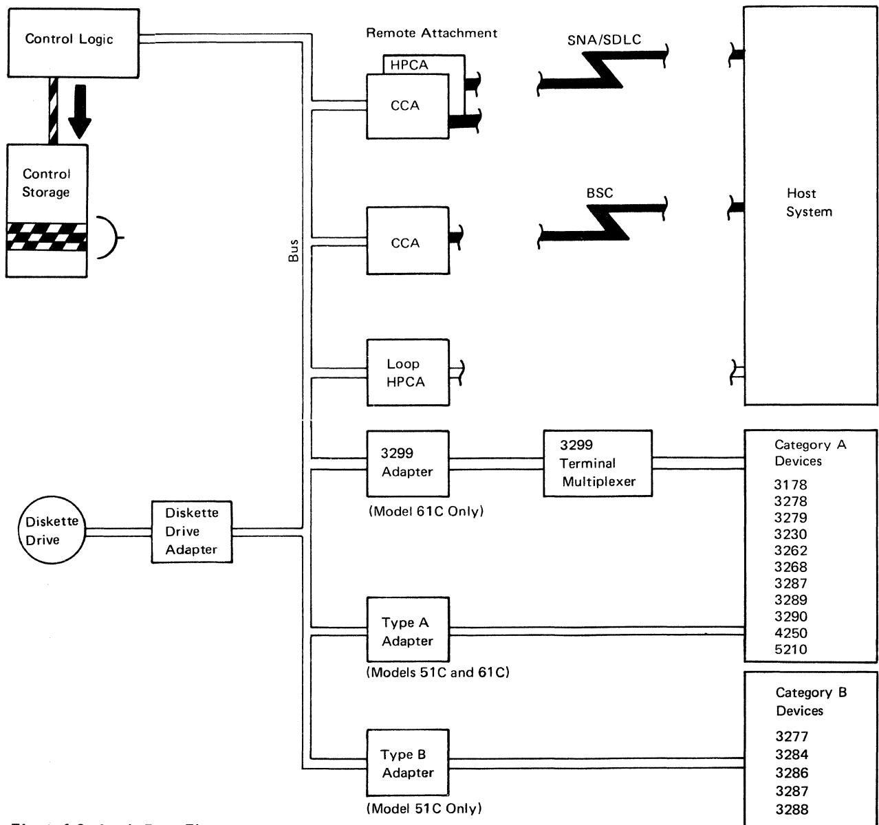
Figure 1-6. Logic Data Flow
