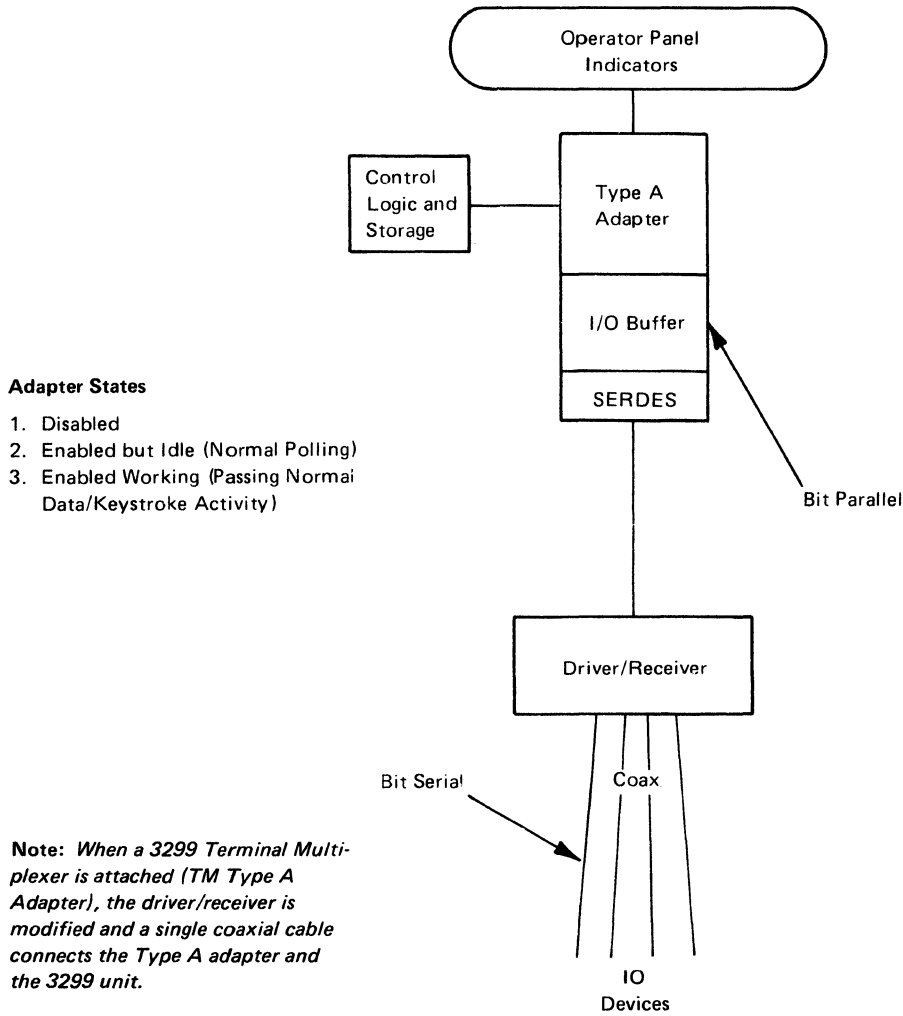
Figure 1-12. Coax to Type A Adapter Data Flow
