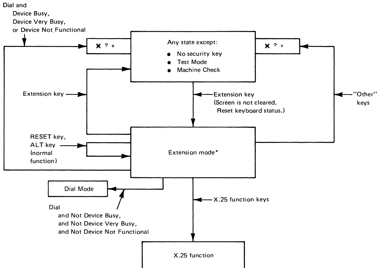
Figure D-3. Extension Mode Definition
