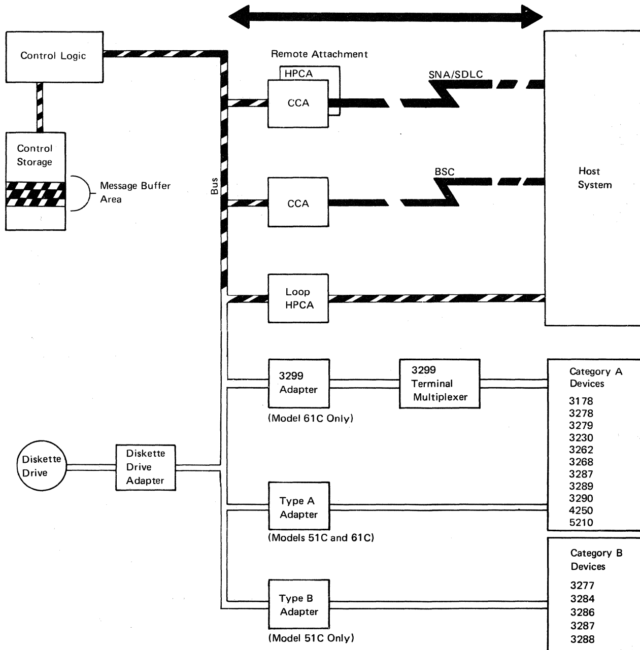
Figure 1-5. Message Data Flow between 3274 Control Unit and Host System
