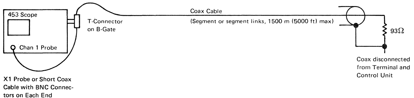
Figure 4-12. Scope Setup
