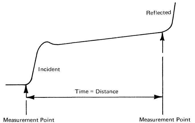
Figure 4-13. Measurement Points
