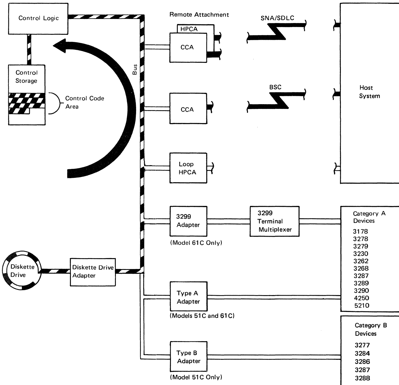
Figure 1-3. Initial Machine Load (IML) Data Flow
