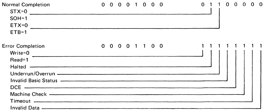
Figure 3-3 (Part 3 of 4). CCA BSC Operation Ending Chart (Code CCCC)
