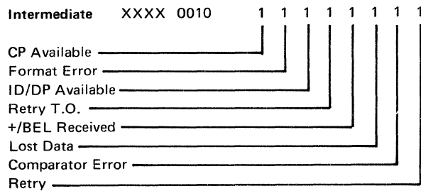
Figure 3-11 (Part 1 of 2). X.21 Switched Log Settings
