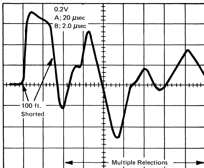
Figure 4-14 (Part 3 of 3). Display Examples
