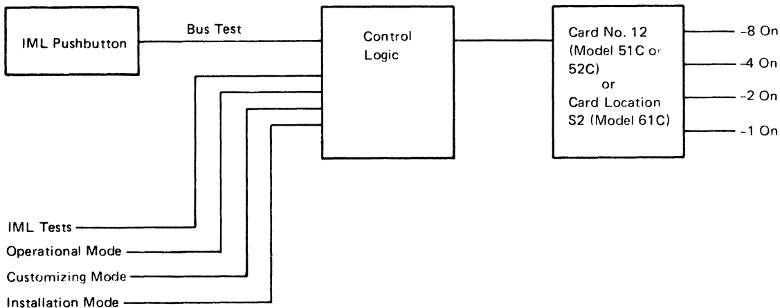
Figure 2-1. 8 4 2 1 Indicator Control Logic
