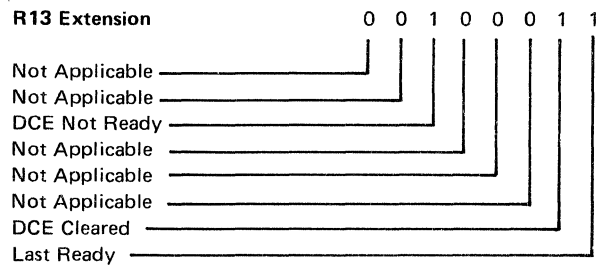
Figure 3-11 (Part 2 of 2). X.21 Switched Log Settings
