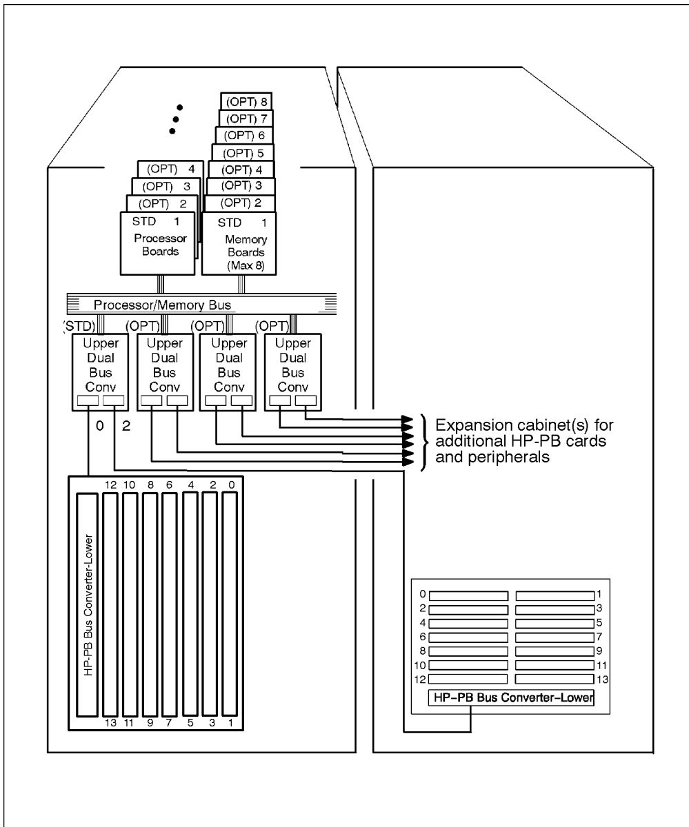
Figure B-7 HP 9000 T500 Configuration and Bus Relationships
