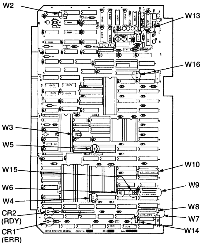
Figure 3-1. Jumper Locations
