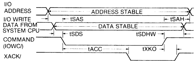
SLAVE COMMAND TIMING
