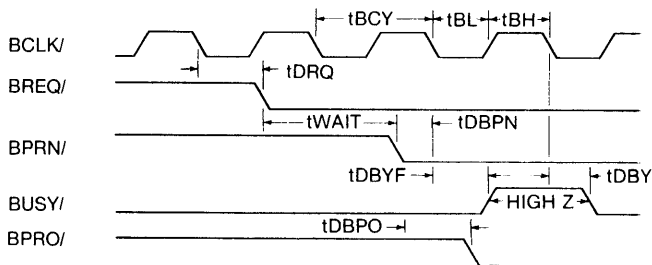
BUS EXCHANGE TIMING
