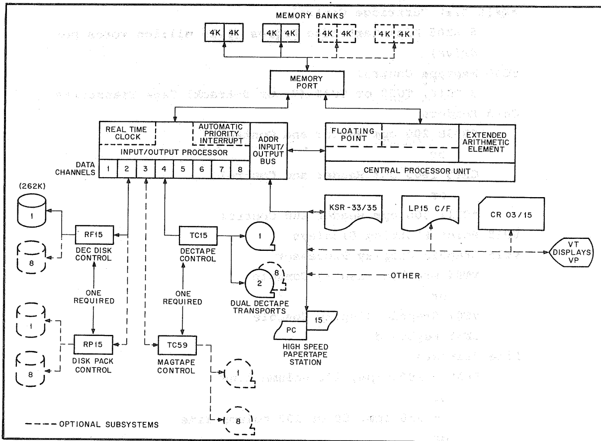
Figure 1-1 Hardware Environment
