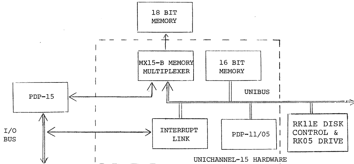
Figure 1-2 Unichannel-15 Hardware
