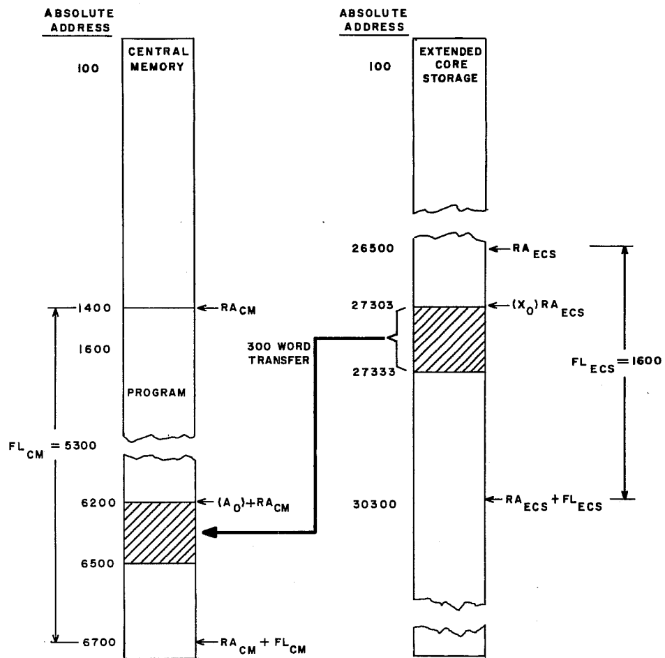
Figure 2-2. Memory Map (Read ECS Example)
