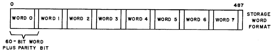
Figure 1-2. ECS Word Format
