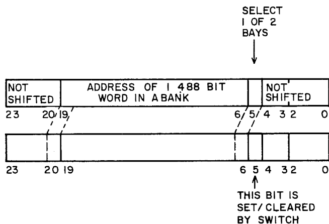
Figure 3-3. Example of Address Shifting for 1000K
