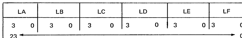
Figure .2-2. L Register
