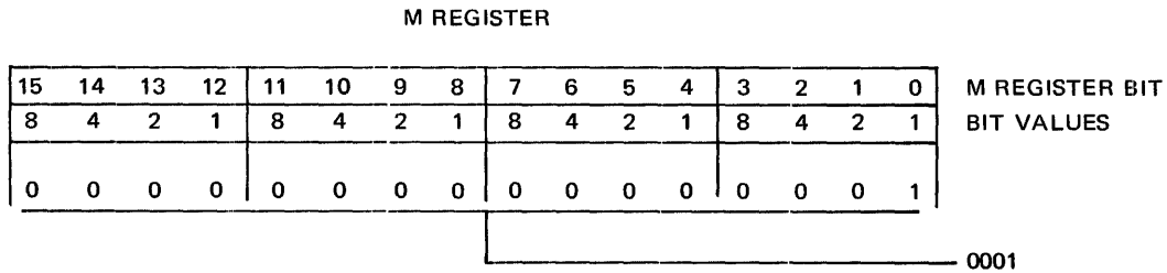
Figure 4-28. Halt (0001)
