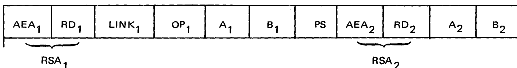
Figure 7-14. Reader Sorter I/O Descriptor
