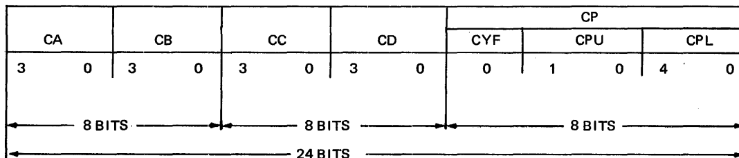
Figure 3-10. - C Register
