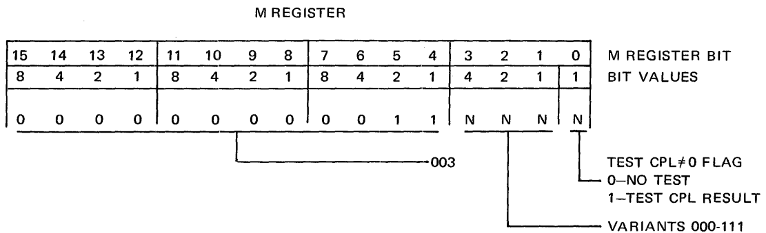
Figure 4-24. Bias (003N)
