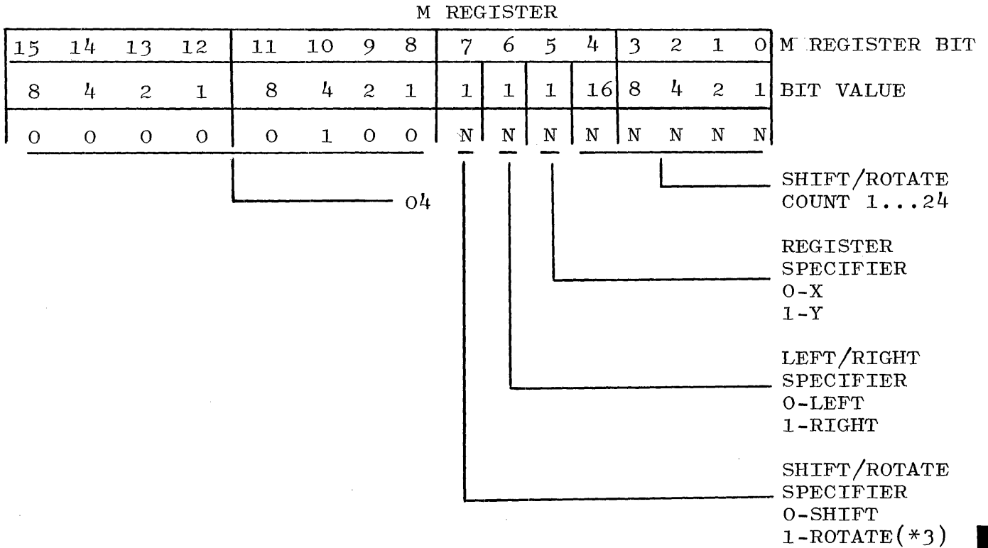
Figure 4-17. Shift/Rotate X or Y (04NN)
