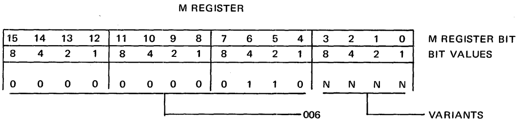
Figure 4-27. Set CYF (006N)
