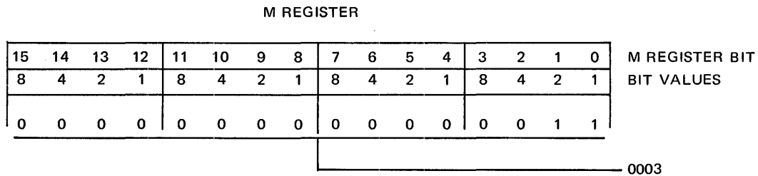
Figure 4-30. Normalize X (0003)
