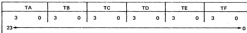
Figure 3-6. T Register
