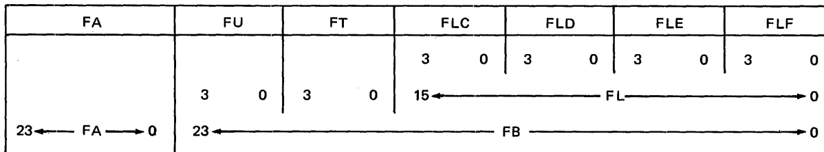
Figure 3-7. F Register
