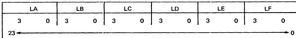
Figure 3-5. L Register
