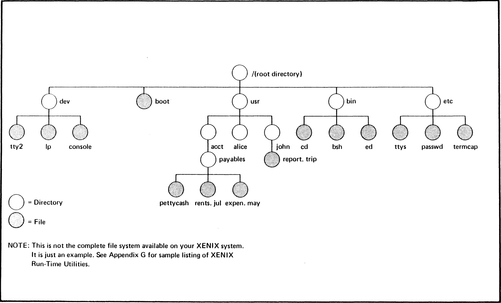
Figure 2-2. Example of XENIX Hierarchical File System
