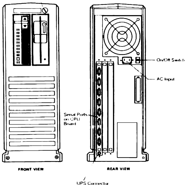
Altos 386 Series 600 Front and Rear Panels
